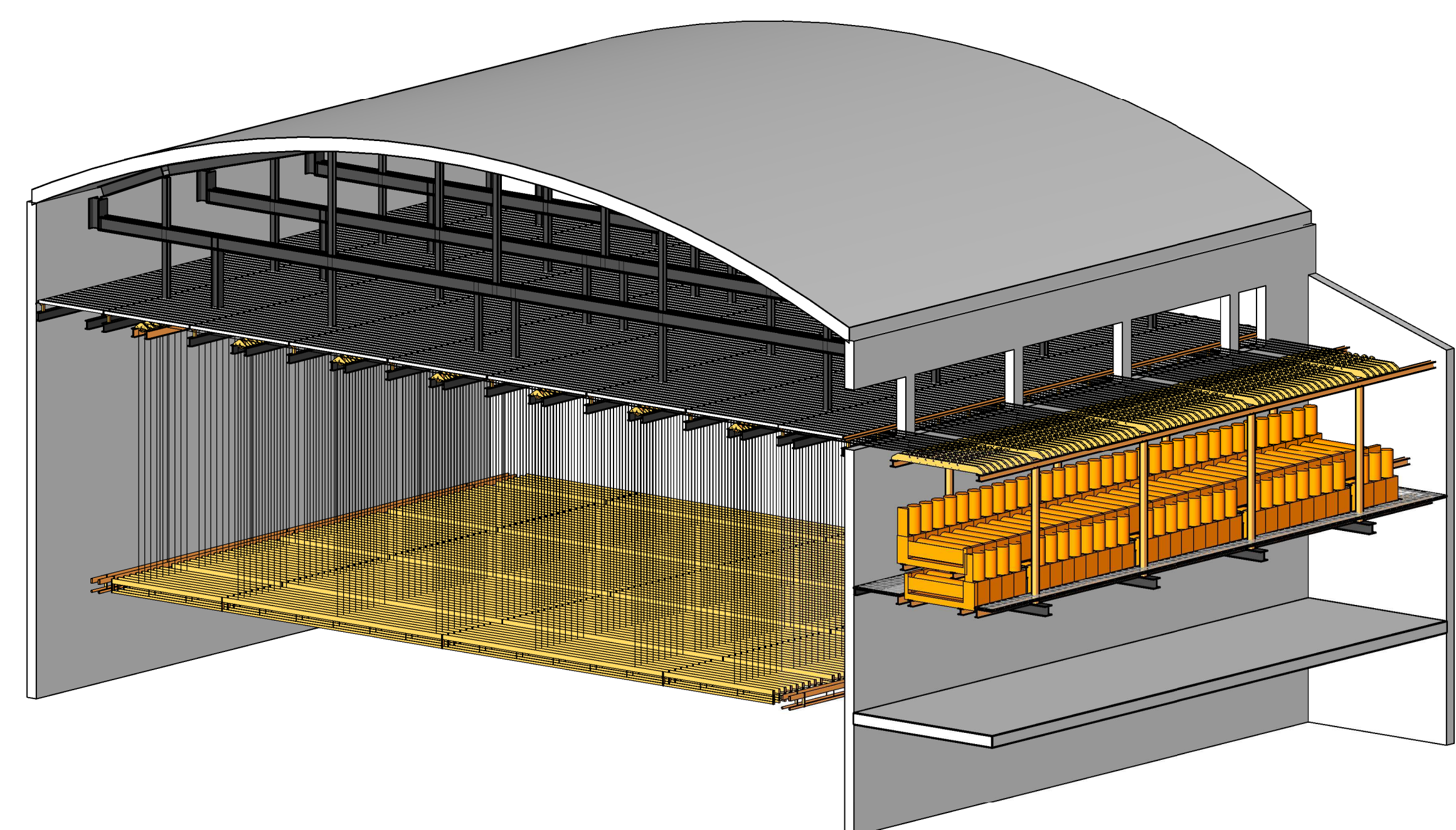
3D Langsdoorsnede
