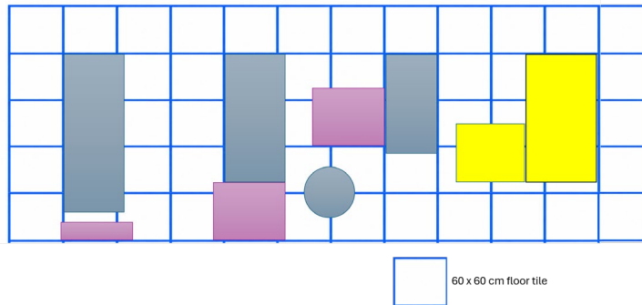
Figure 6.3.1 System positioning and footprint. The footprint of the system may not be larger than the area marked by two yellow boxes. The smaller yellow box is allocated for system computers.
