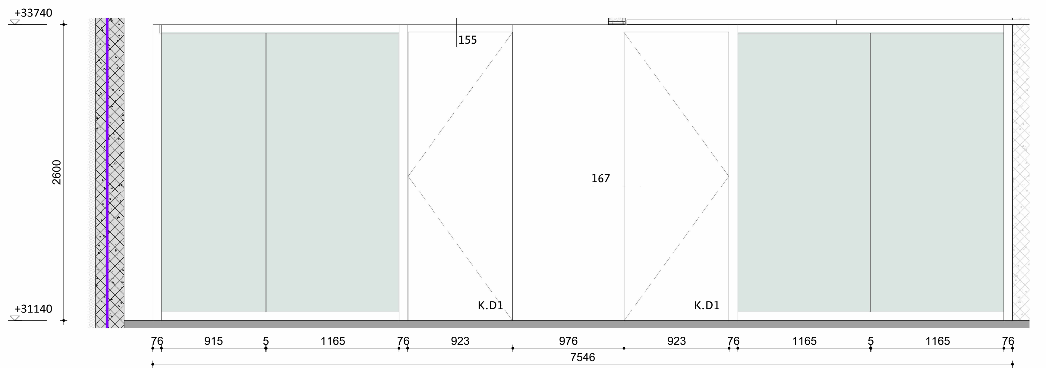
wandaanzicht kantoren as 5
