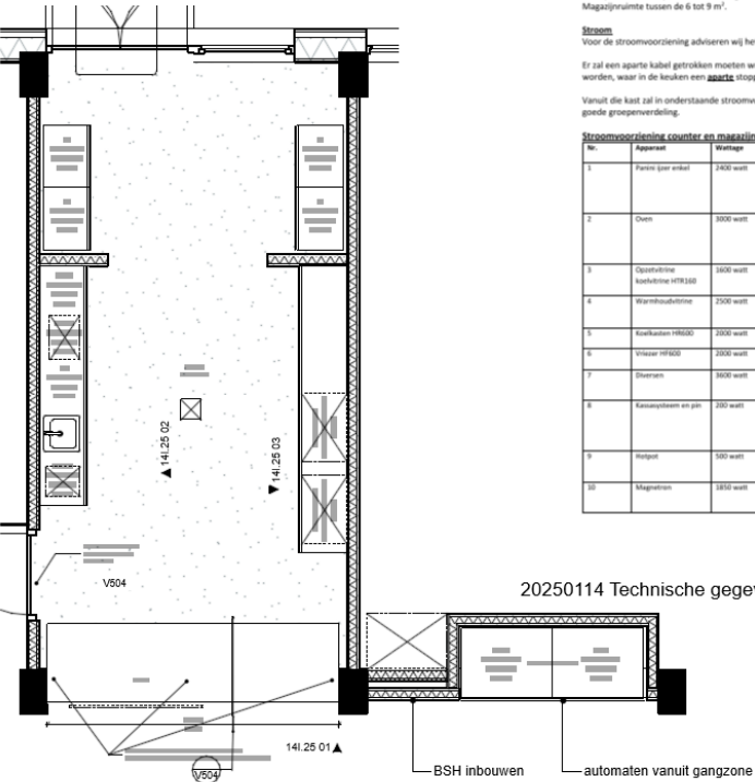
00 Begane grond
