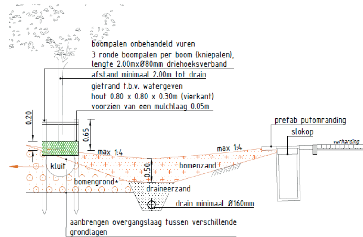
Standaard detail 3.1.5. Boom in wadi
