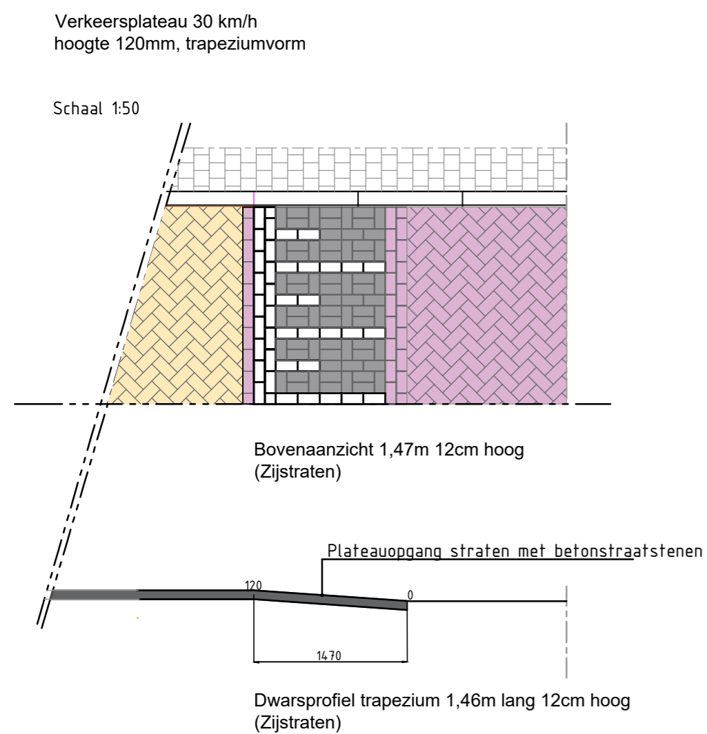
Principe profiel plateau's
