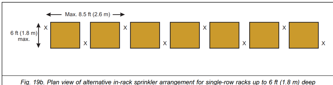
Fig. 19b. Plan view of alternative in-rack sprinkler arrangement for single-row racks up to 6 ft (1.8 m) deep
