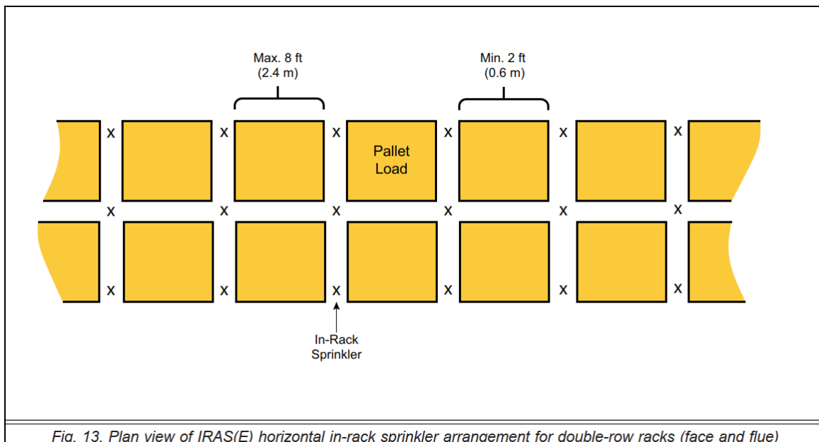
Fig. 13. Plan view of IRAS(E) horizontal in-rack sprinkler arrangement for double-row racks (face and flue)
