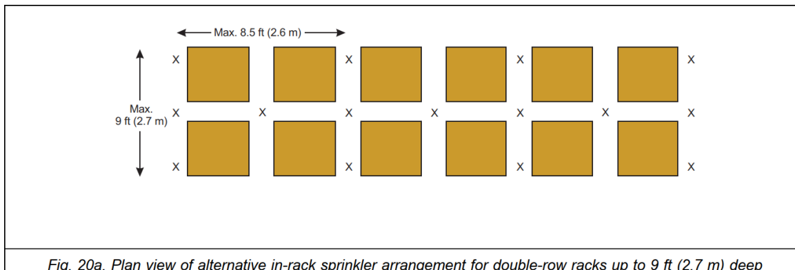
Fig. 20a. Plan view of alternative in-rack sprinkler arrangement for double-row racks up to 9 ft (2.7 m) deep
