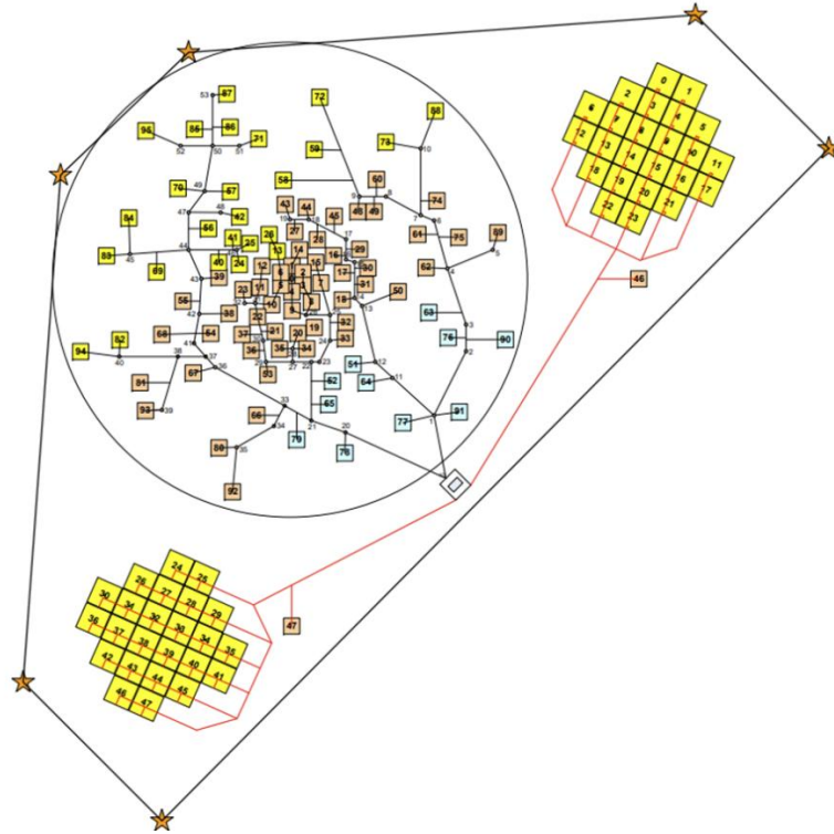
LOFAR CS001
