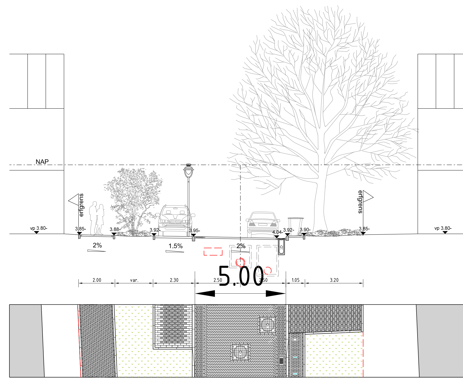
Profiel 13 links
