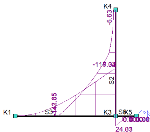
Fu.C. Omhullende Momenten (My)
