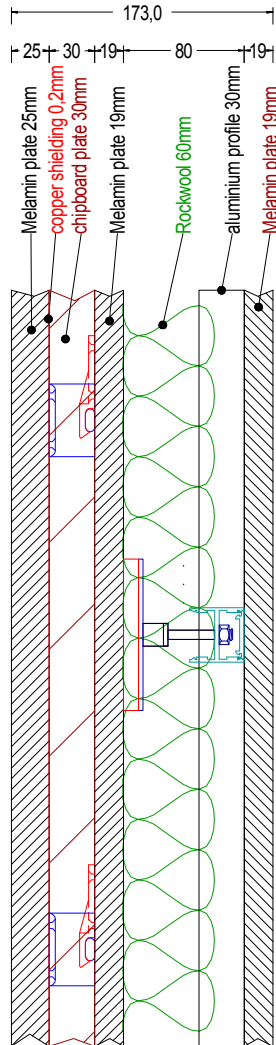
vertical wall section- front, right, rear cabin wall
