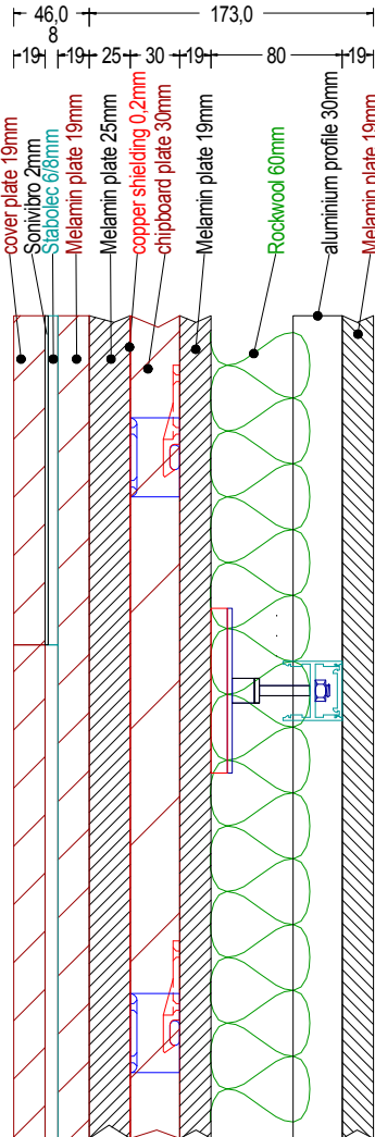
vertical wall section- left cabin wall
