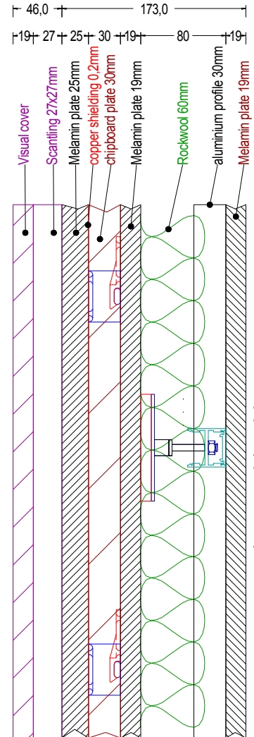
vertical wall section- left, front cabin wall
