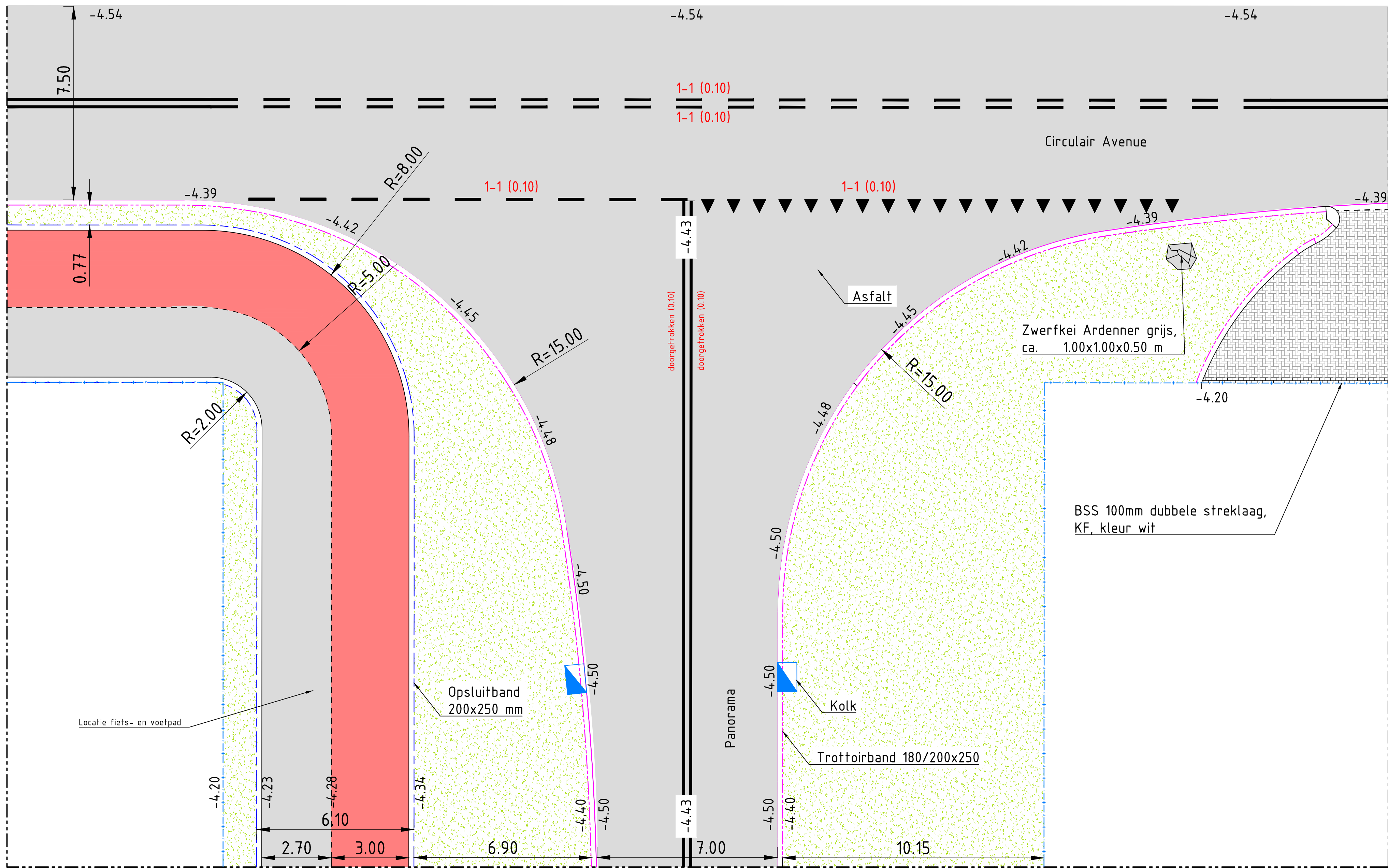
Detail 09: Cruising Panorama SCHAAL 1 : 100
