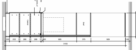
7. Detail A-B
