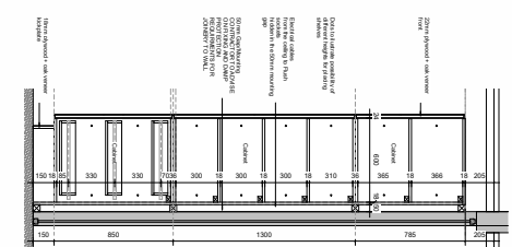
4 / Pegsoos Storage - Section
