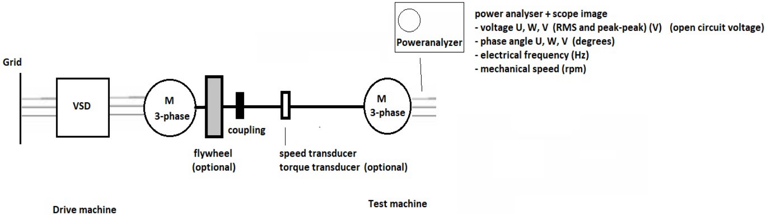
Fig. 3.9: Mechanical overspeed test and BEMF.
