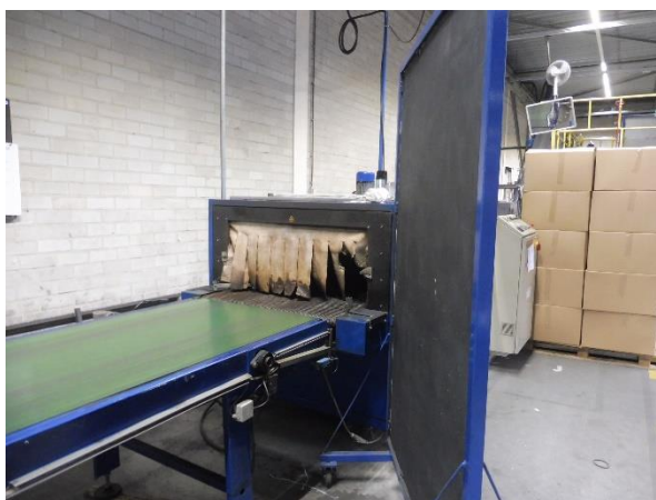
Krimptunnel.
