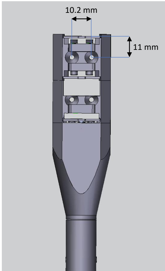
Top view sample cassette (3 slots)
