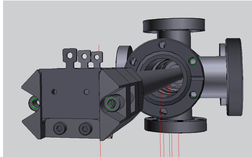
Perspective view of the front of the sample cassette
