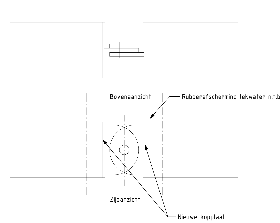
Detail 3 Herziening tand-nok verbinding Schaal 1 : 20
