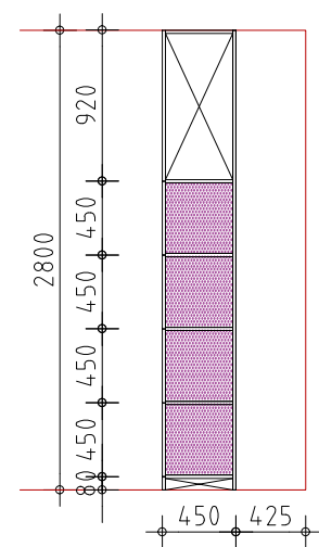
dwarsdoorsnede lockers
