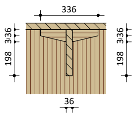
Detail 1:10
