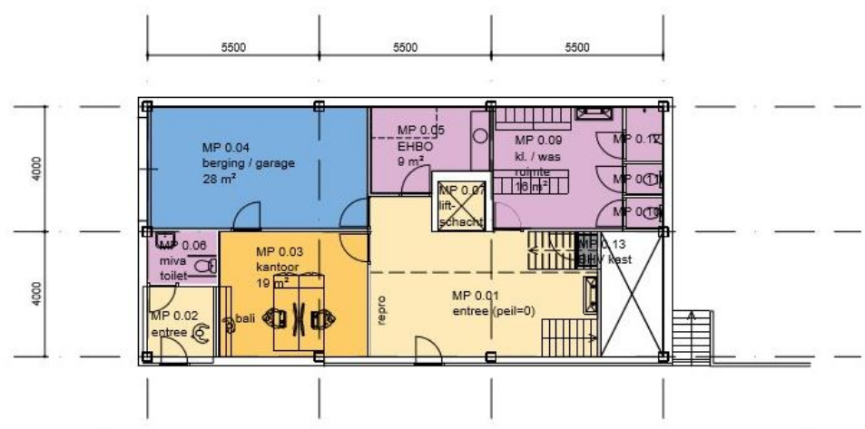
MP - begane grond 137 m² bvo
