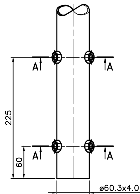
A (1:4)
