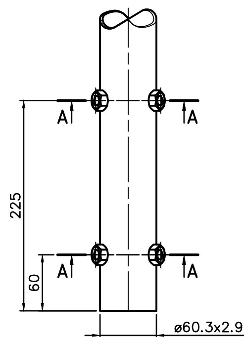
A (1:4)
