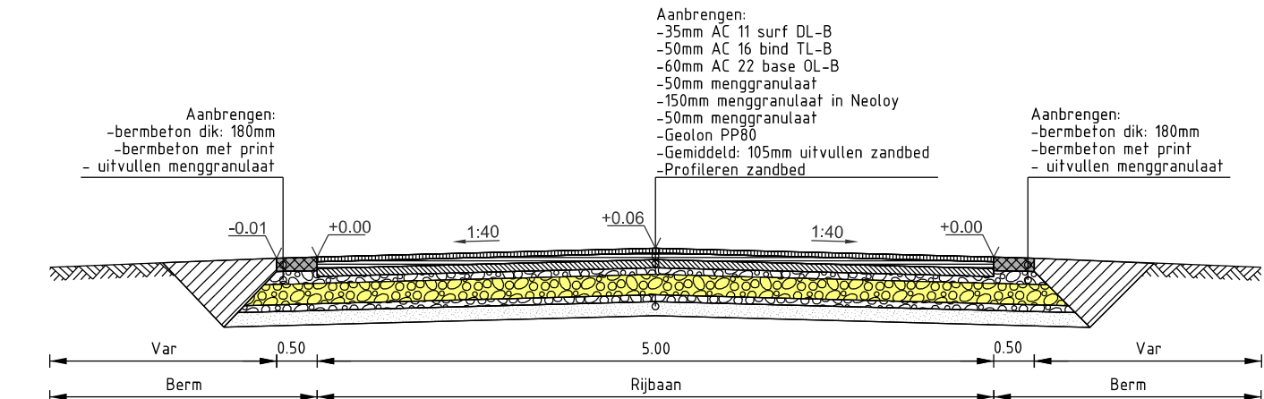
Principeprofiel H-H
