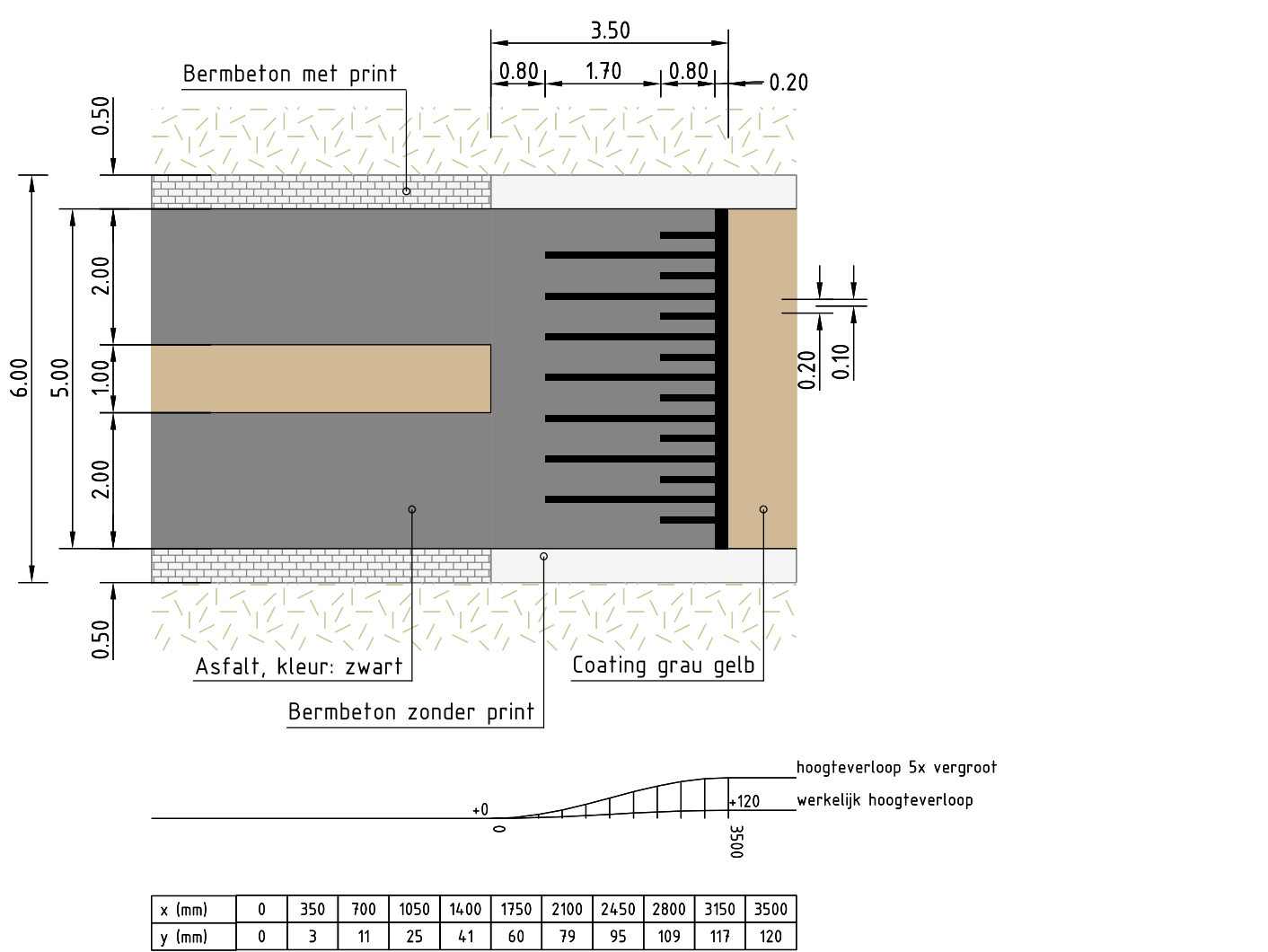
Principedetail plateauhelling
