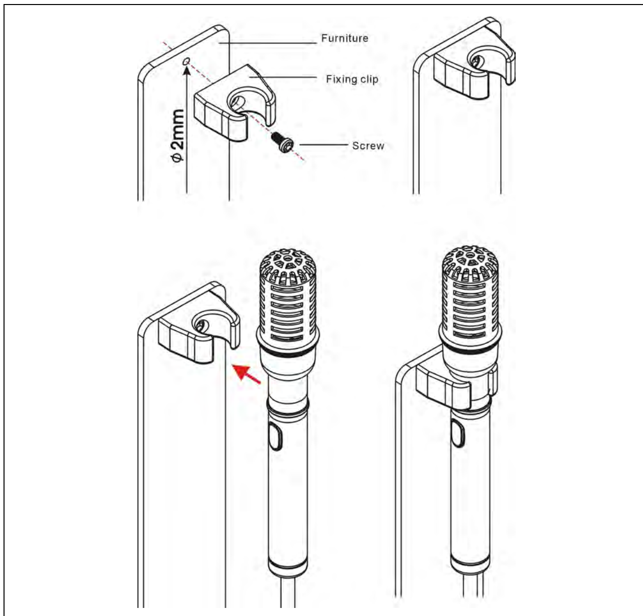
Figure 3.12.8 Installation diagram of HCS-4327HDA/50
