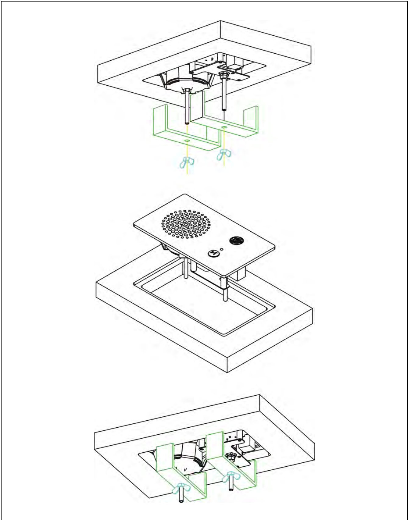
Figure 3.3.9 Installation of HCS-48U7MICSPK series flush-mounted congress unit
