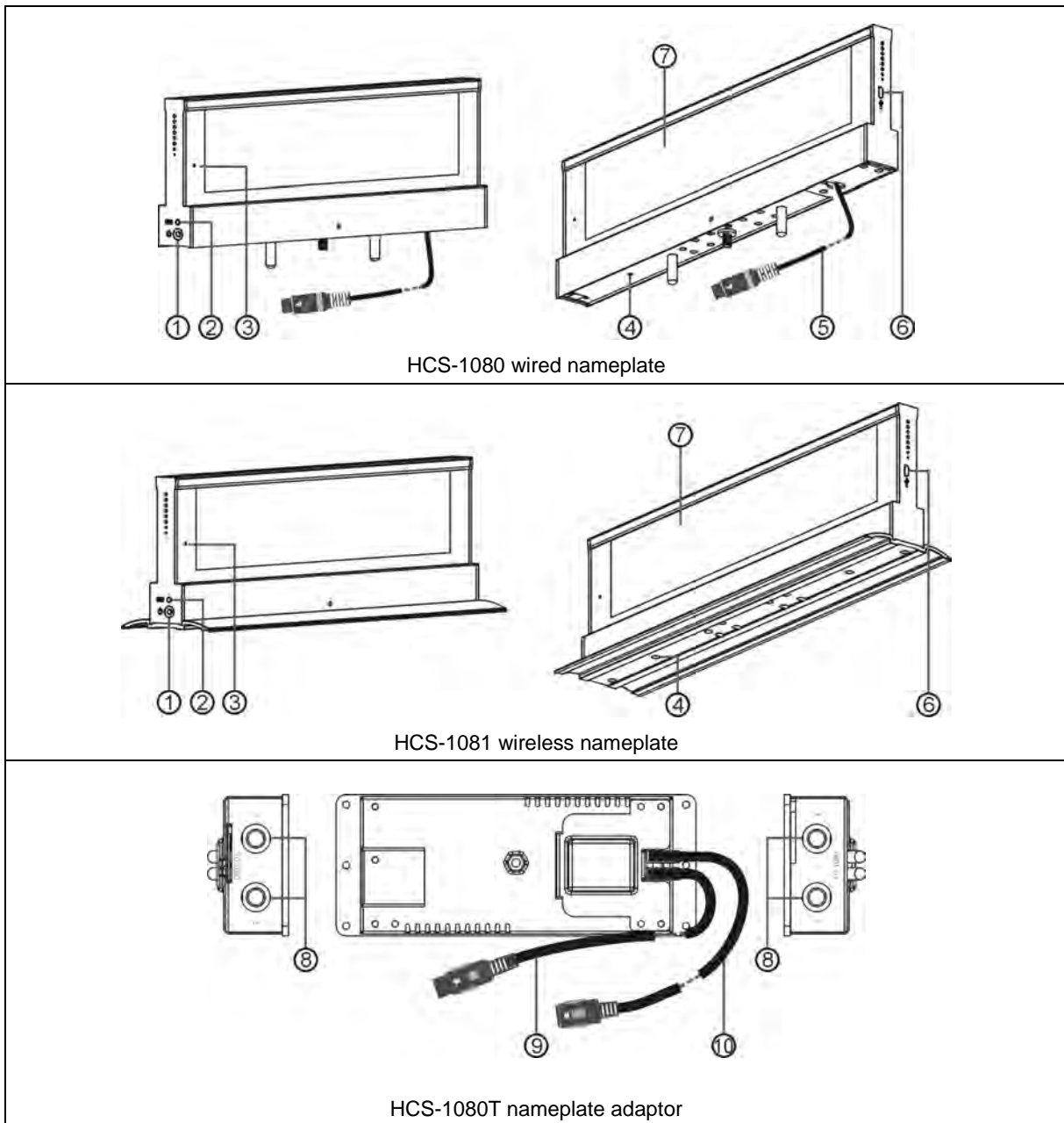
Figure 3.17.1 HCS-1080 series E-ink nameplate
