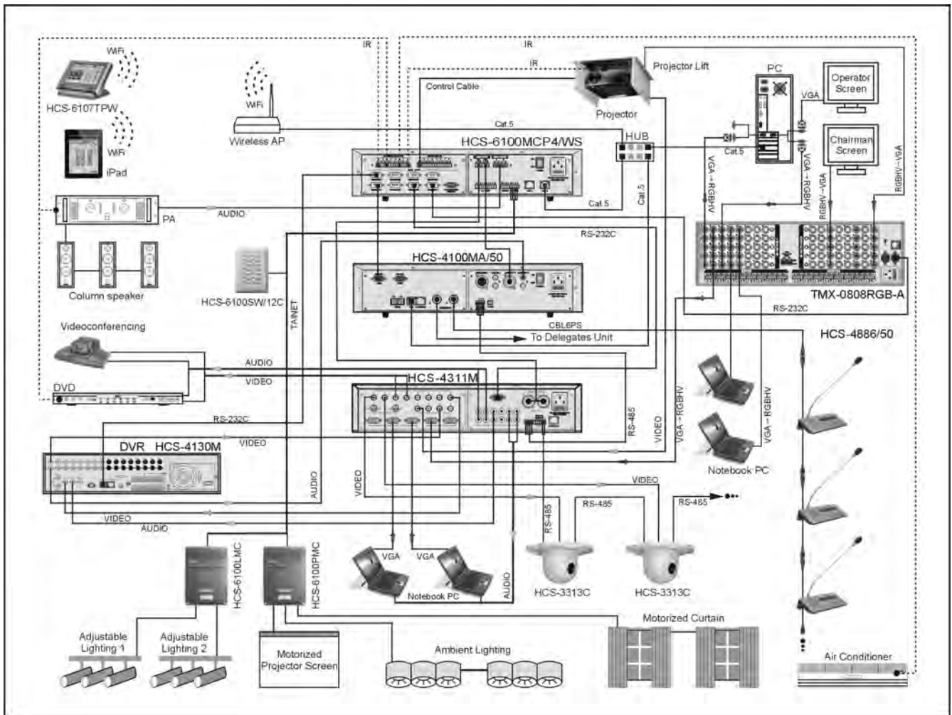
Figure 5.1.8 HCS-4100M/50 congress system main unit connecting to central control system
