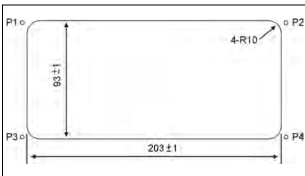
Figure 3.7.2 Fixing hole positioning diagram of HCS-4360/61/62/63 series congress unit (unit: mm)
