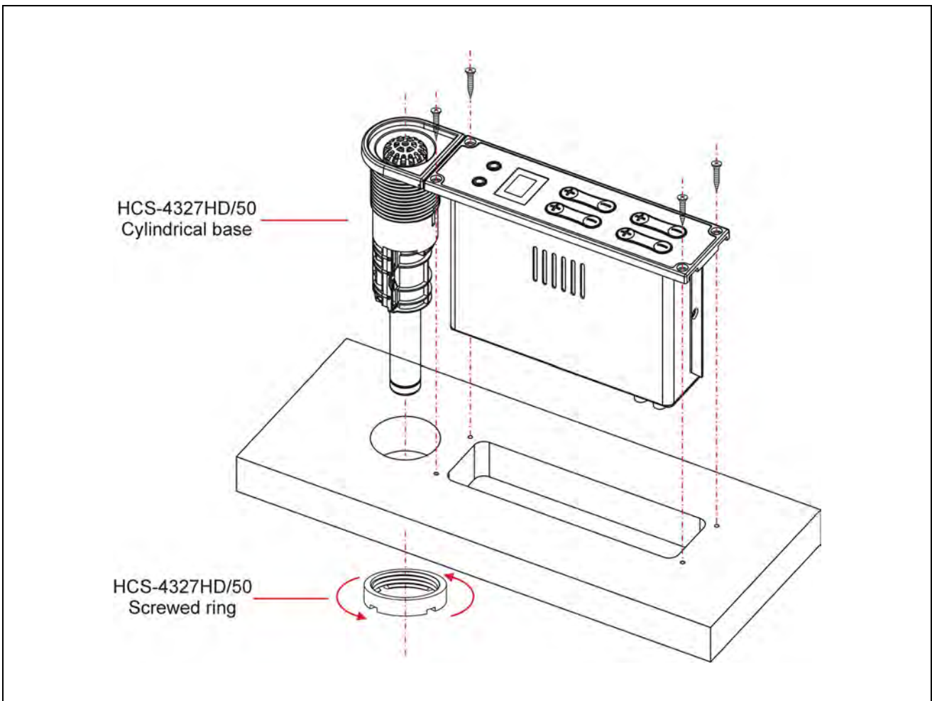
Figure 3.12.5 Installation diagram of HCS-4325/26 series congress unit with HCS-4327HD/50
