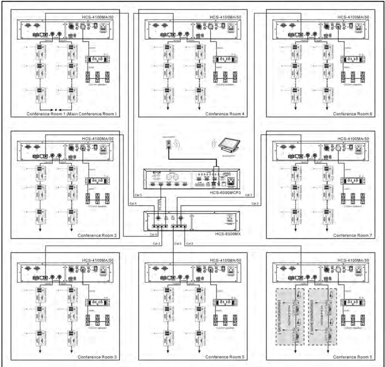
Figure 5.1.10 Combining/splitting meeting rooms with HCS-8300MX Congress Room Combiner and Cat. 5 cables
