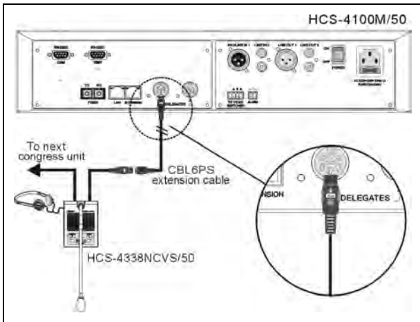
Figure 3.8.2 HCS-4338N/50 series congress unit connected to the CMU/EMU
