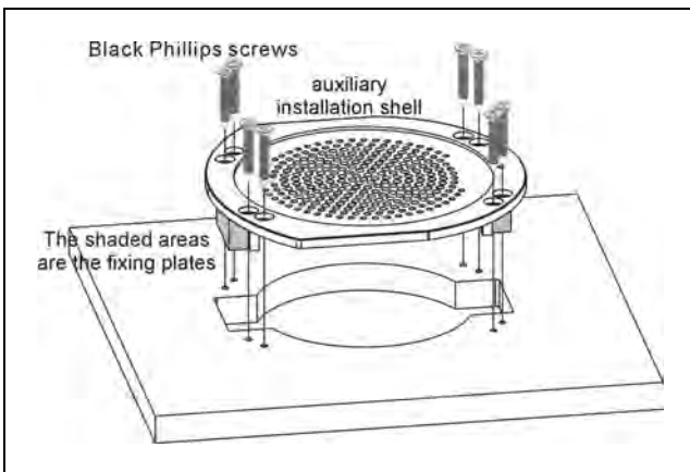
Figure 3.14.12 Installation diagram of the fixing plates of the HCS-4844/50 series flush-mounted loudspeaker
