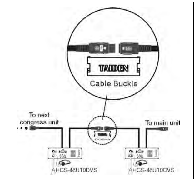
Figure 3.4.6 “Daisy-chain” connection between HCS-48U10 series congress units
