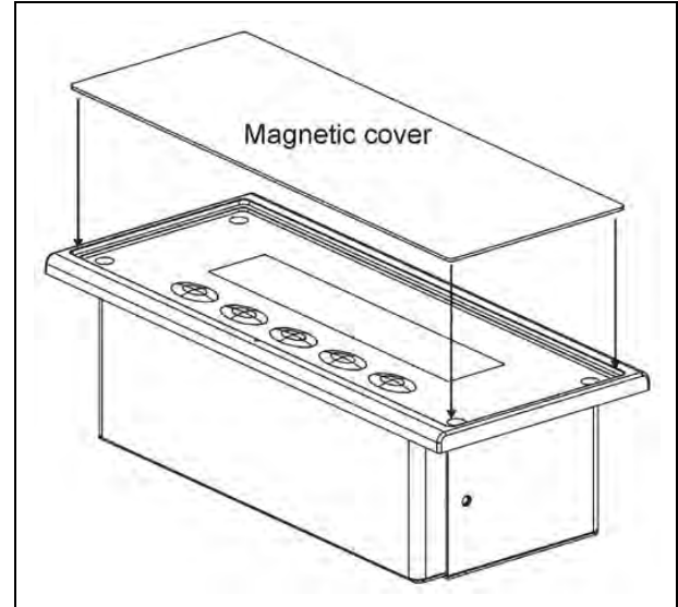
Figure 3.15.4 Installation diagram of the protective cover of HCS-4368/50 series flush-mounted voting unit
