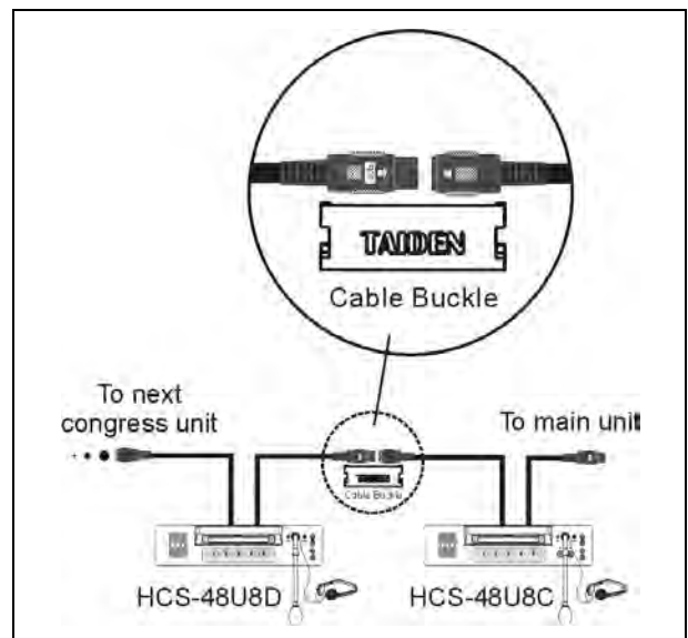
Figure 3.3.17 “Daisy-chain” connection between HCS-48U7/U8/U9 series congress units
