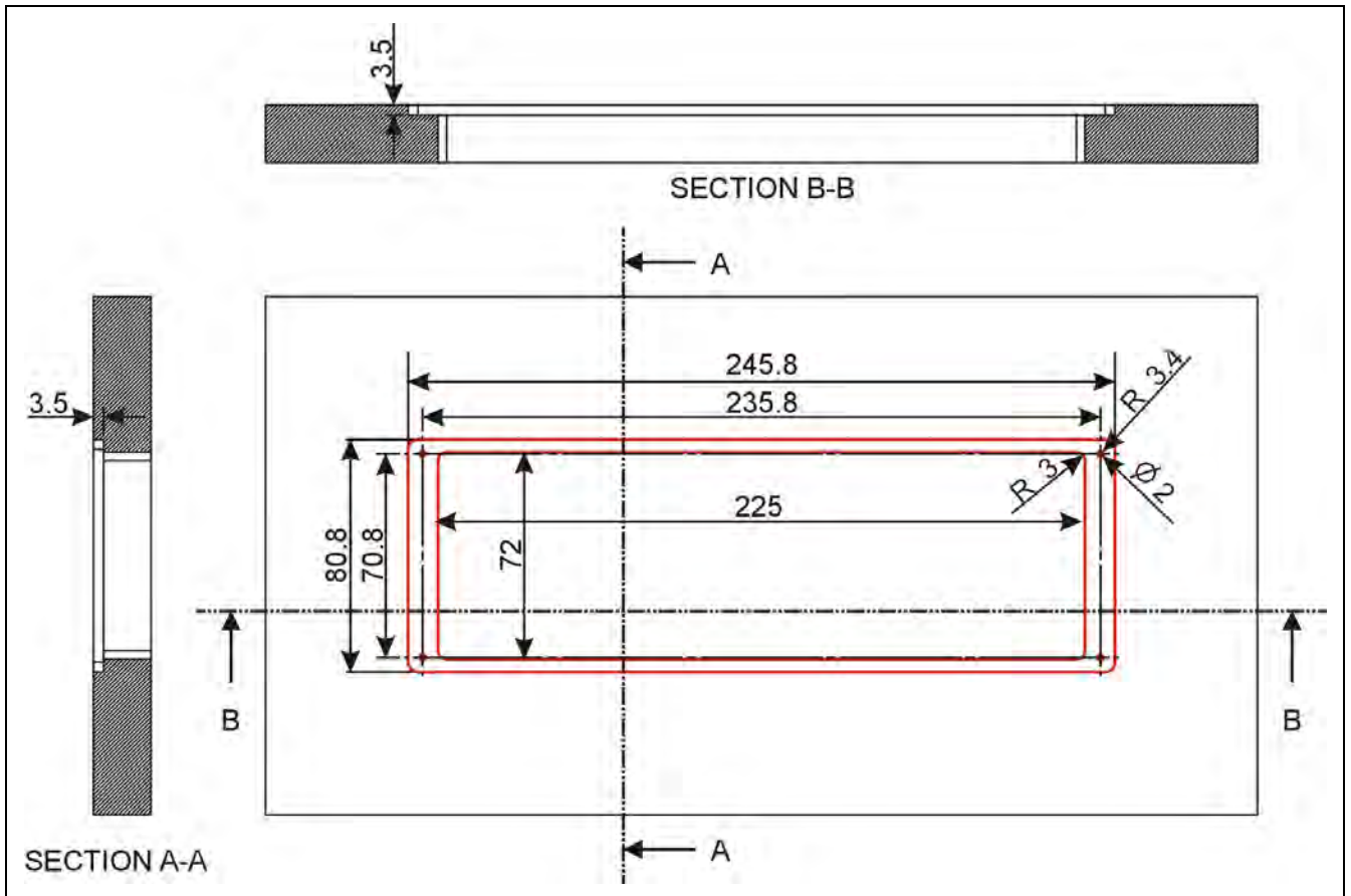
Figure 3.4.2 Cutout of HCS-48U10 series congress unit (unit: mm)
