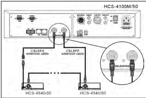
Figure 3.14.16 “Closed Loop - Daisy Chain” connection between the CMU and multi-function connectors
