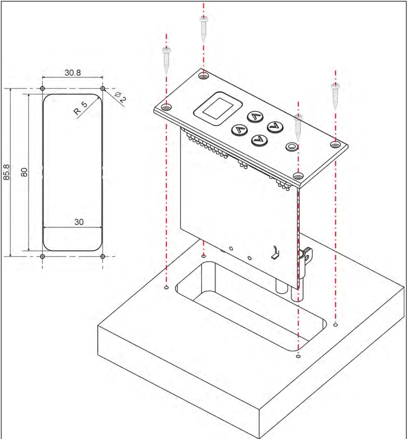
Figure 3.14.10 Installation of the HCS-4842NA/50 flush-mounted channel selector
