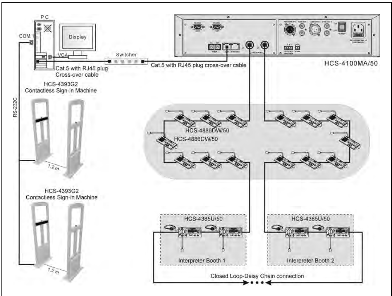
Figure 5.1.9 Connection between Conference Sign-in System and HCS-4100/50 system
