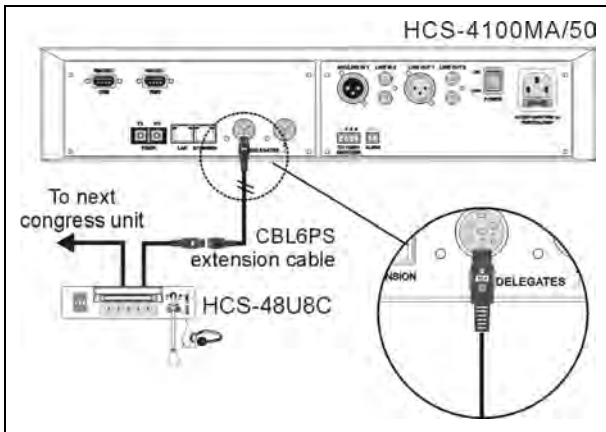
Figure 3.3.15 HCS-48U7/U8/U9 series congress unit connected to the CMU/EMU
