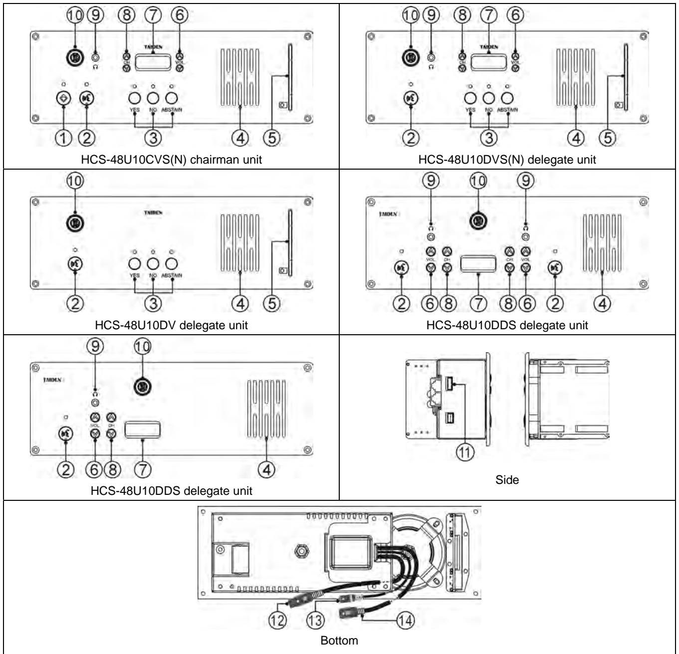
Figure 3.4.1 HCS-48U10 series congress units
