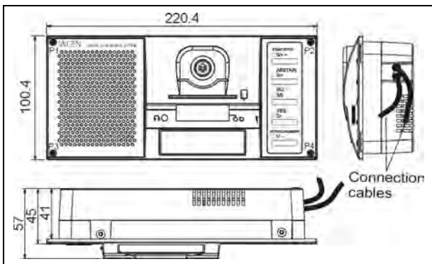
Figure 3.7.3 Flush-mounted installation diagram of the HCS-4360/61/62/63 series congress unit
