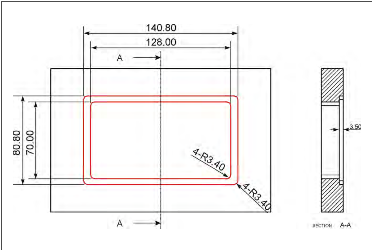
Figure 3.3.6 Cutout of HCS-48U7MICSPK flush-mounted congress unit (unit: mm)
