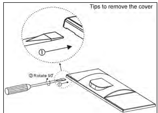
Figure 3.7.5 Dismounting the protective cover of HCS-4360/61/62/63 series congress unit
