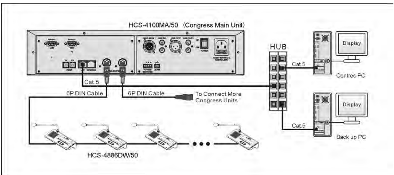
Figure 5.1.12 Dual PC server hot spare
