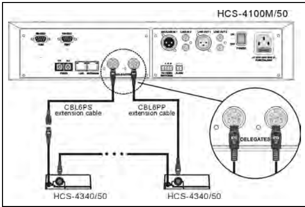
Figure 3.13.5 “Closed Loop - Daisy Chain” connection between the CMU and HCS-4340/50 series multi-function connector
