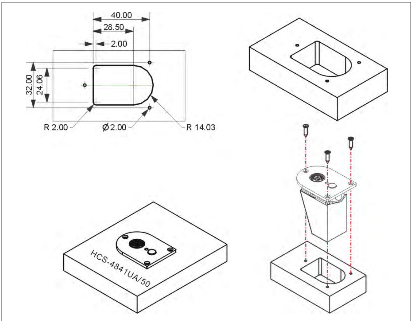
Figure 3.14.9 Installation of the HCS-4841UA/50 flush-mounted channel selector
