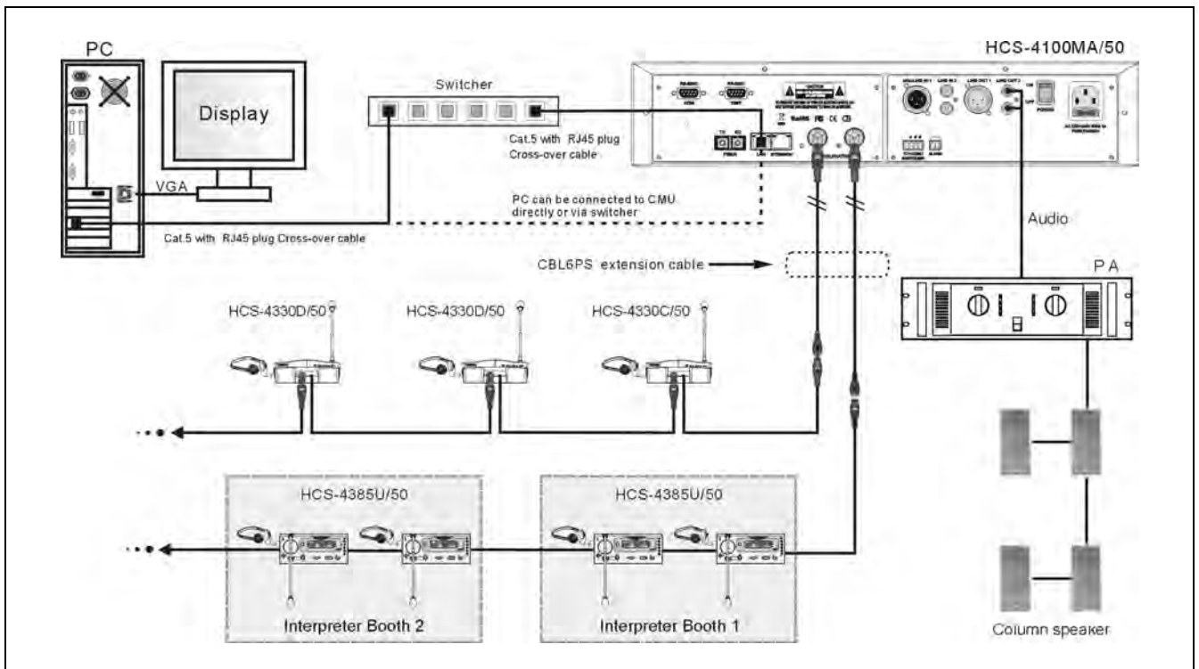
Figure 5.1.2 Congress main unit connecting to HCS-4330/50 series contribution units and HCS-4385U/50 interpreter units
