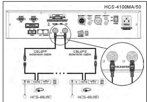
Figure 3.2.16 “Closed Loop - Daisy Chain” connection between the CMU and HCS-48U6 series congress unit
