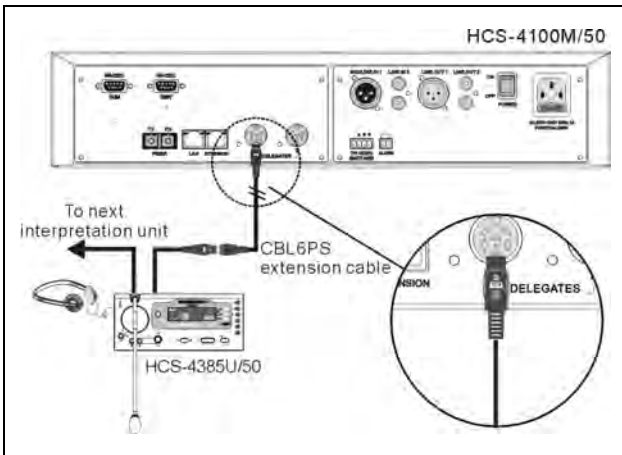
Figure 4.3.1 HCS-4385U/50 interpreter unit connected to the CMU or the EMU
