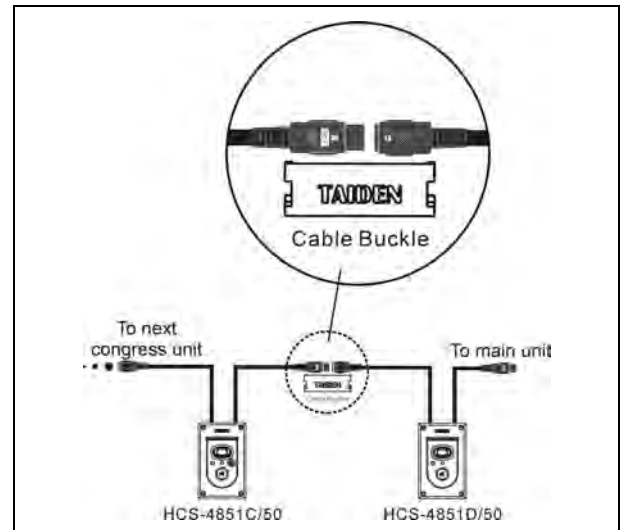
Figure 3.10.4 “Daisy-chain” connection between HCS-4851/50 series congress units
