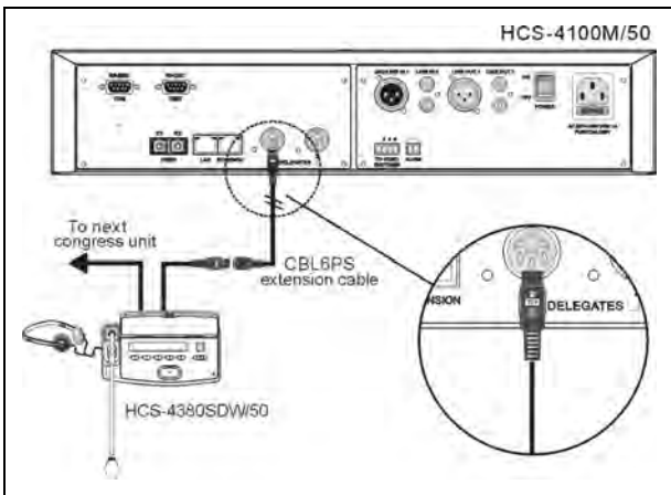
Figure 3.6.2 HCS-4380/82/70/71 series congress unit connected to the CMU/EMU
