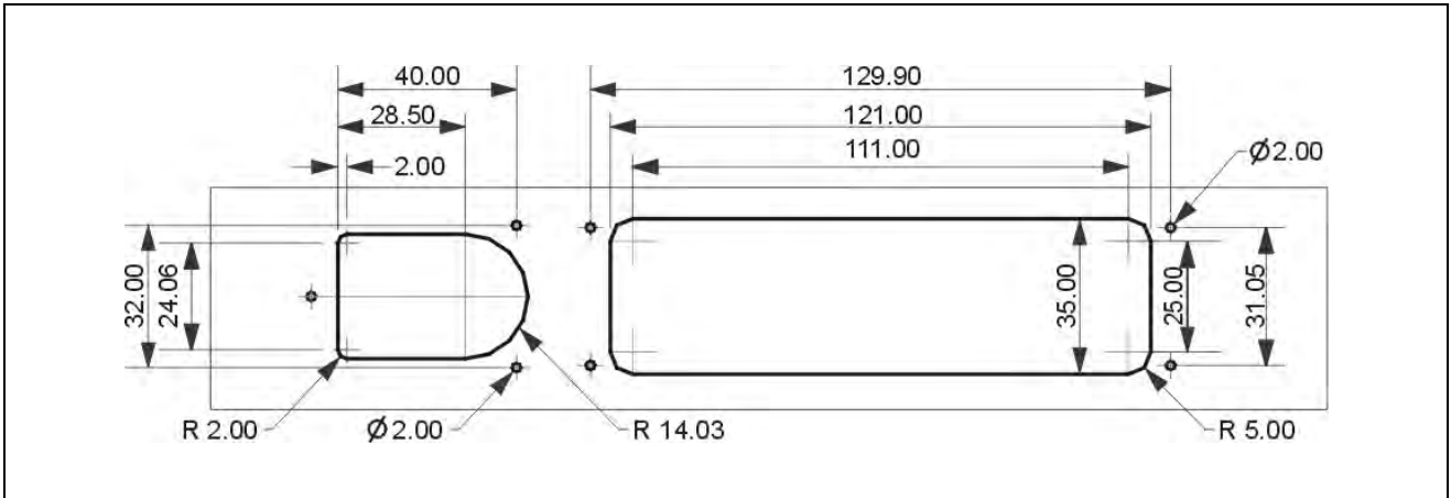
Figure 3.12.6 Fixing hole positioning diagram of HCS-4325/26 series congress unit with HCS-4327D/50 (unit: mm)
