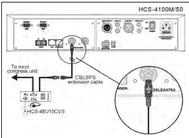
Figure 3.4.4 HCS-48U10 series congress unit connected to the CMU/EMU
