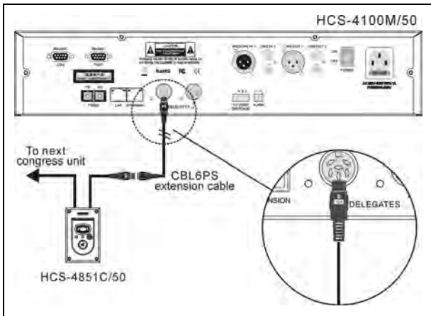
Figure 3.10.2 HCS-4851/50 series congress unit connected to the CMU/EMU
