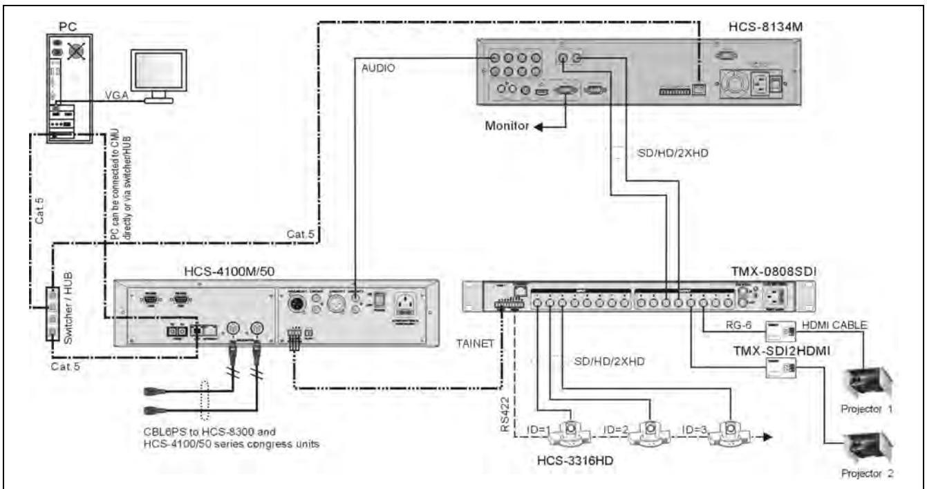
Figure 5.1.5 HCS-4100M/50 congress main unit connecting to the automatic video tracking system
