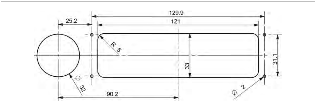
Figure 3.12.4 Fixing hole positioning diagram of HCS-4325/26 series congress unit with HCS-4327HD/50 (unit: mm)
