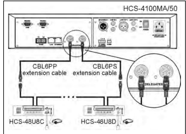
Figure 3.3.16 “Closed Loop - Daisy Chain” connection between the CMU and HCS-48U7/U8/U9 series congress units
