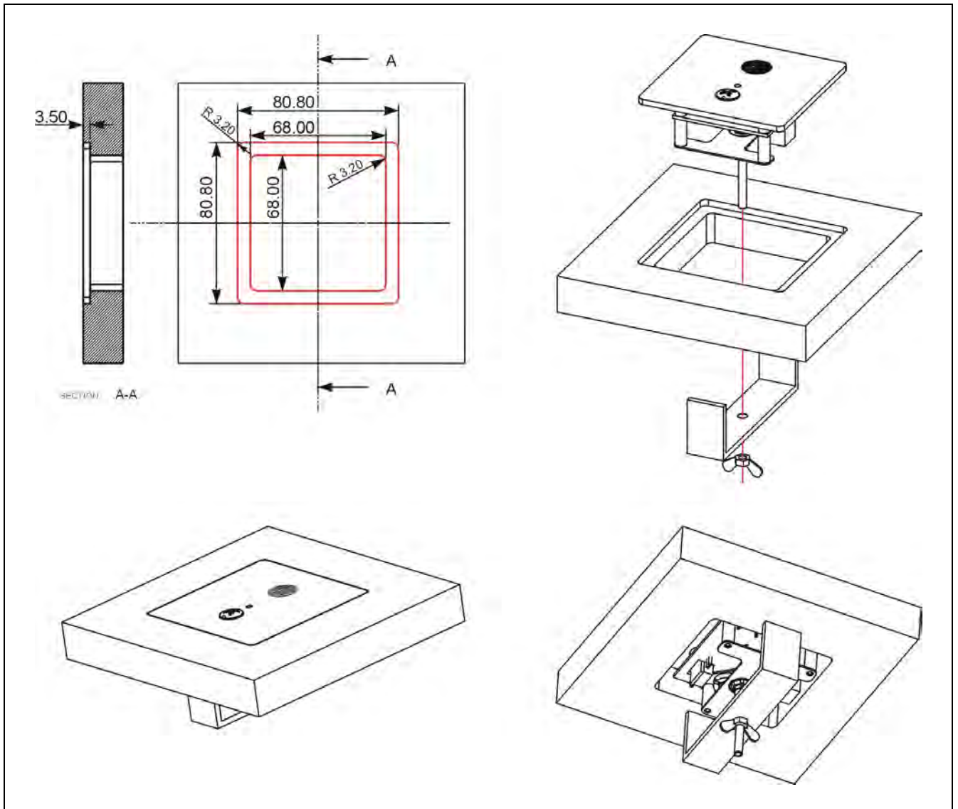
Figure 3.14.8 Installation of the HCS-4841U/50 flush-mounted channel selector
