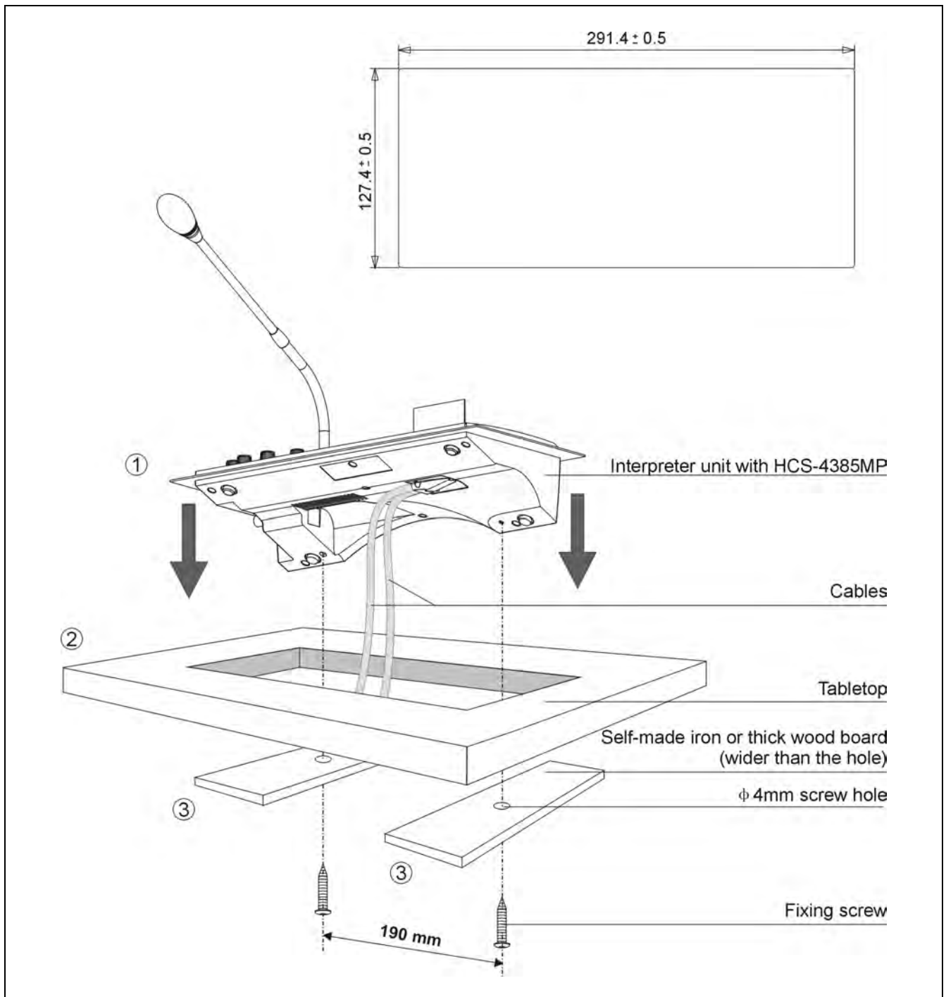
Figure 4.2.1 Installation diagram (unit: mm)
