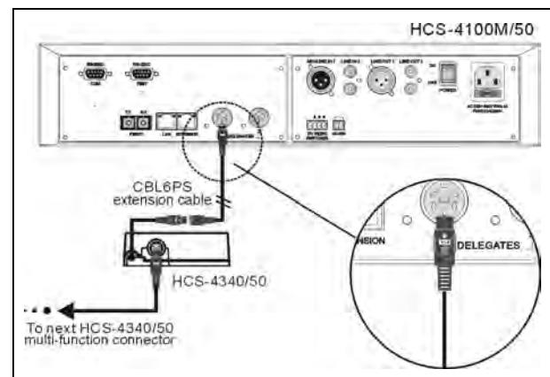
Figure 3.14.15 Multi-function connector connected to the CMU/EMU
