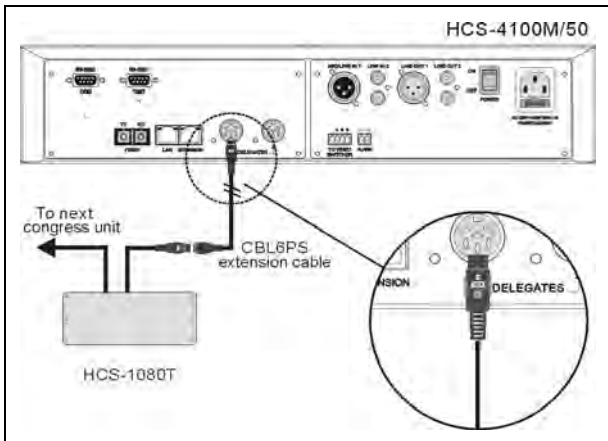
Figure 3.17.3 HCS-1080T connected to the CMU/EMU
