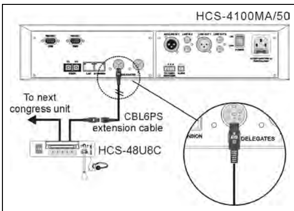
Figure 2.3.1 Congress unit connected to the CMU/EMU
