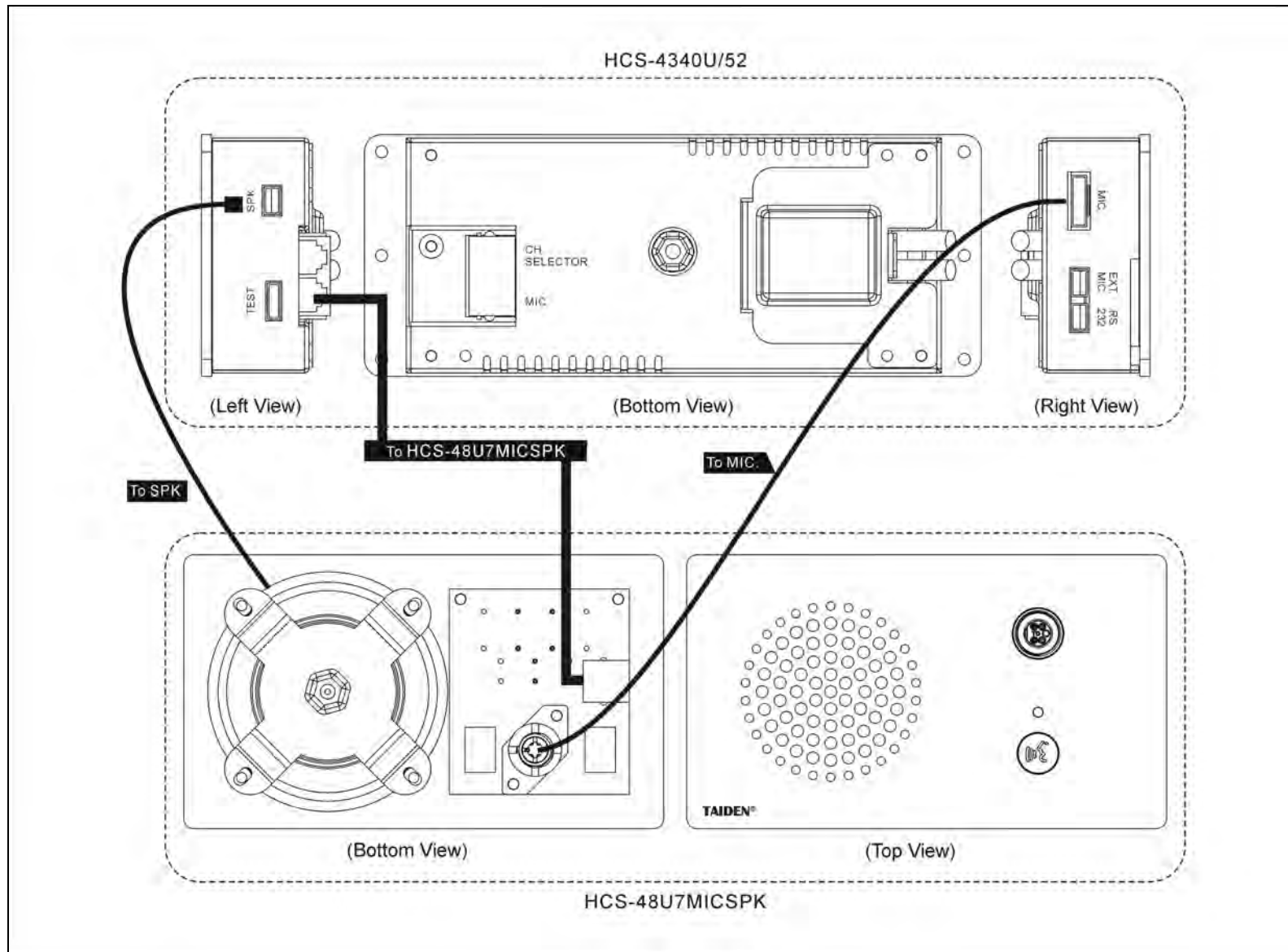
Figure 3.3.14 Connection between HCS-48U7MICSPK congress unit and HCS-4340U/52 multi-function connector
