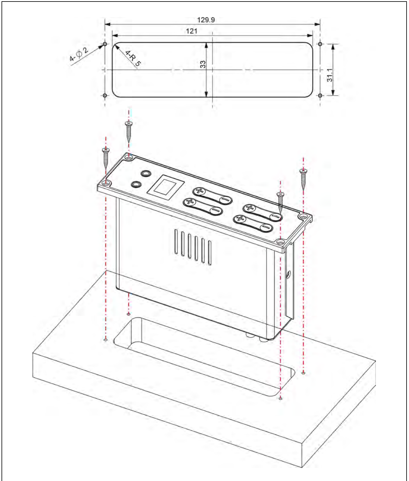
Figure 3.12.2 Installation of HCS-4325/26 series congress unit (except HCS-4325U/50) (unit: mm)
