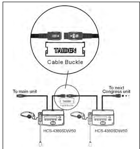
Figure 3.6.4 “Daisy-chain” connection between HCS-4380/82/70/71 series congress units
