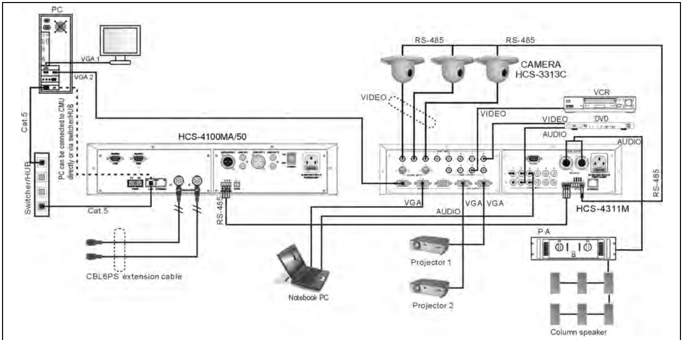
Figure 5.1.4 HCS-4100M/50 congress main unit connecting to the automatic video tracking system
