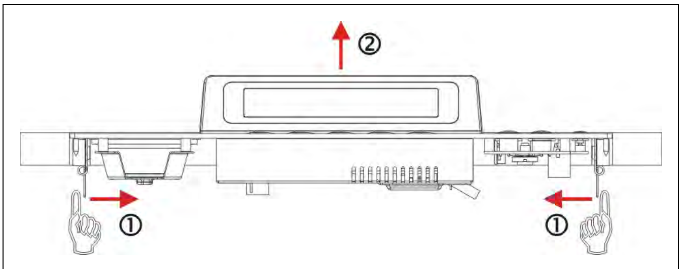
Figure 3.3.11 Disassembly of HCS-48U8 and HCS-48U9 series flush-mounted congress unit (method b)
