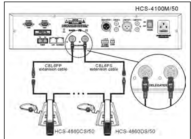
Figure 3.9.3 “Closed Loop - Daisy Chain” connection between the CMU and HCS-4860/50 series congress units
