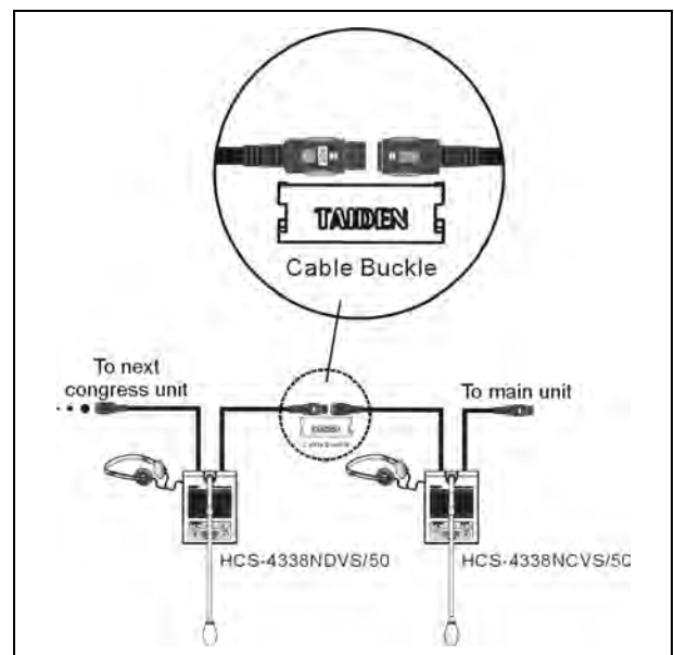
Figure 3.8.4 “Daisy-chain” connection between HCS-4338N/50 series congress units
