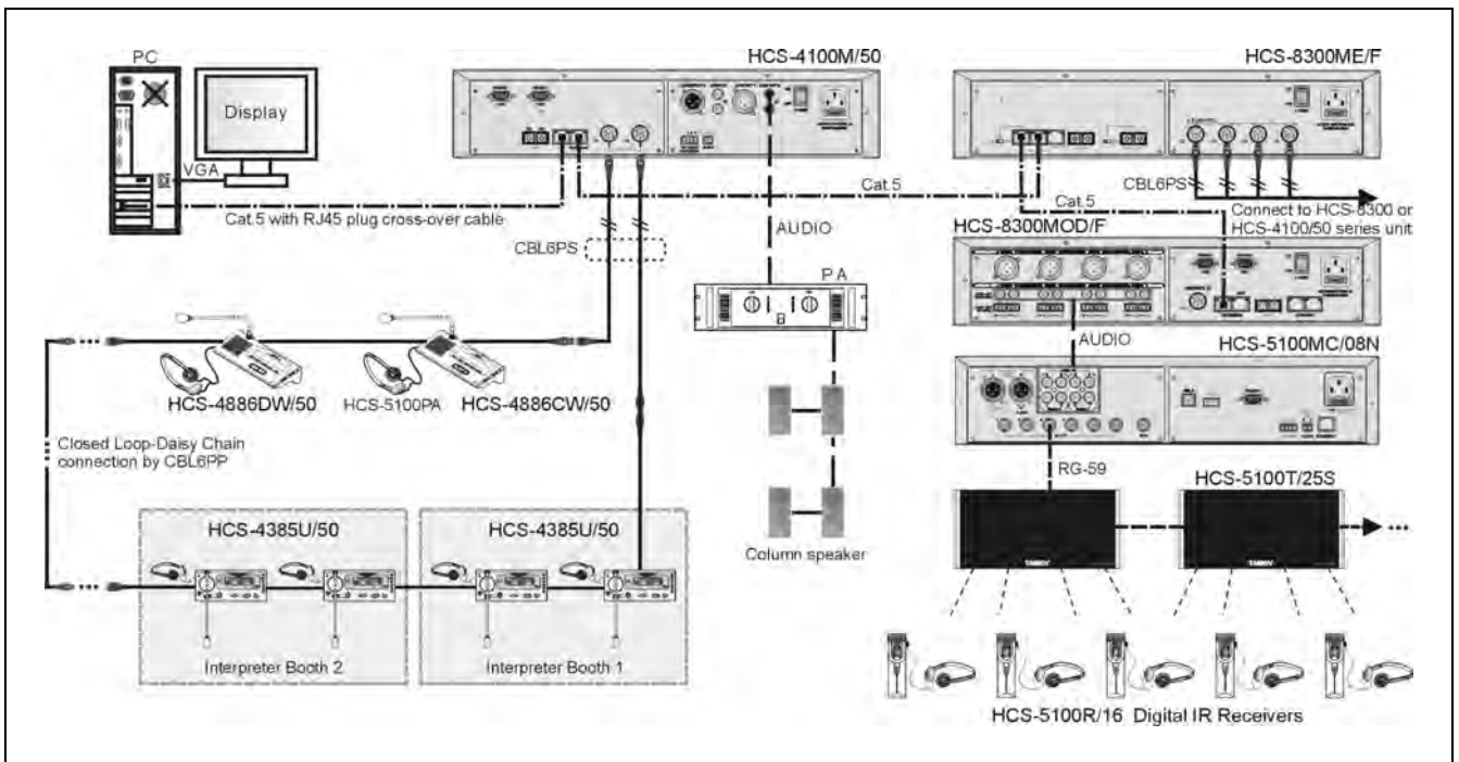
Figure 5.1.7 Congress main unit connecting to digital infrared language distribution system via HCS-5100MC/N
