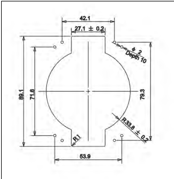
Figure 3.14.11 Positioning diagram of HCS-4844/50 series flush-mounted loudspeaker (unit: mm)
