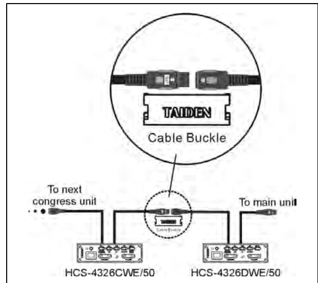
Figure 3.12.11 “Daisy-chain” connection between HCS-4325/26 series congress units
