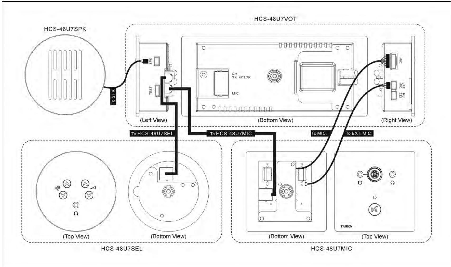
Figure 3.3.13 Connection among the modules of HCS-48U7 congress unit
