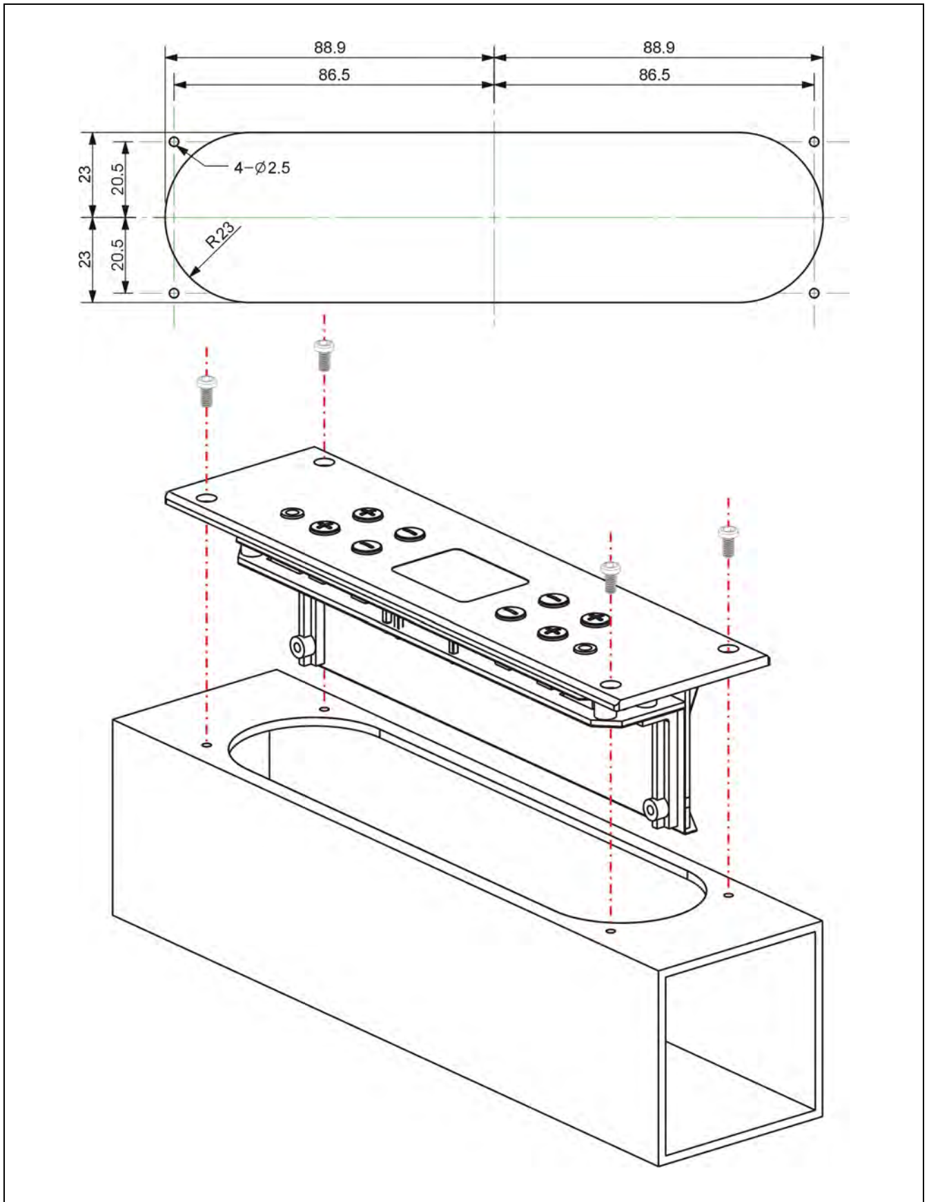
Figure 3.12.3 Installation of HCS-4325U/50 congress unit (unit: mm)
