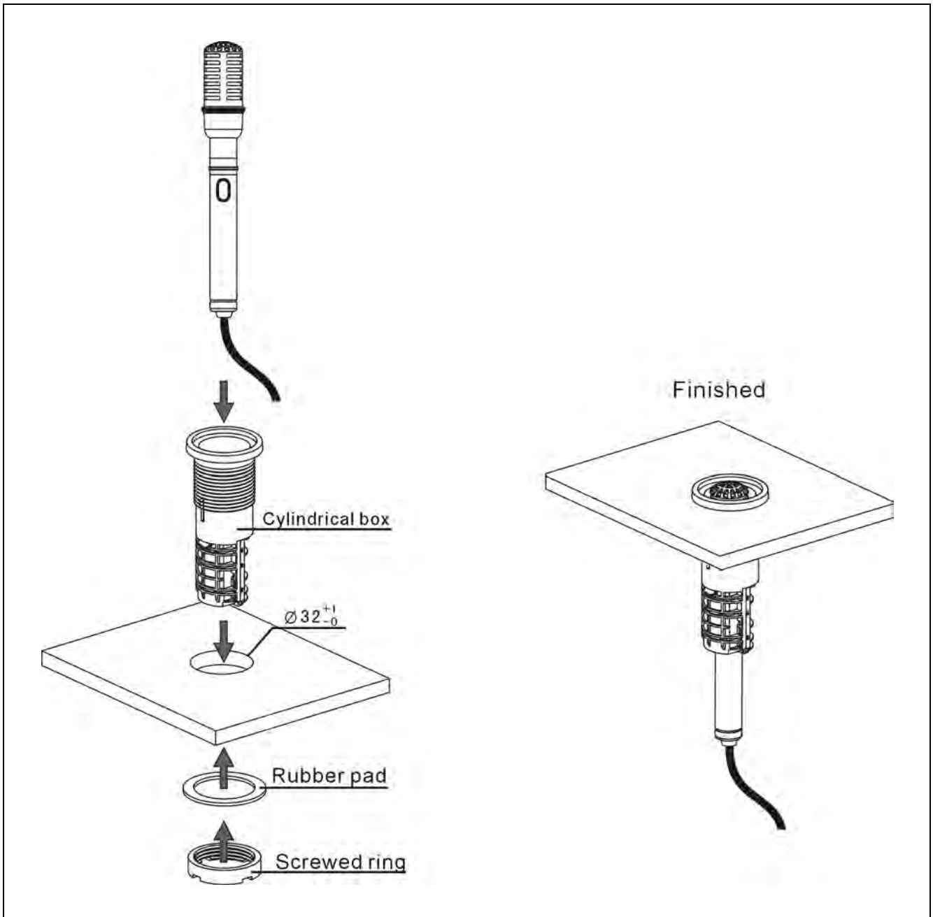
Figure 3.13.3 Installation diagram of flush-mounted handheld microphone (unit: mm)
