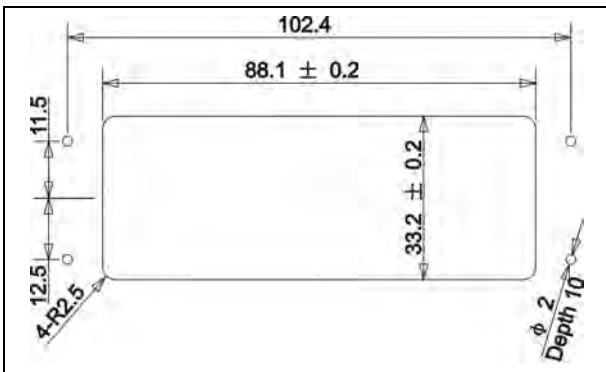
Figure 3.14.3 Positioning diagram of HCS-4841(N)/42N/43N series congress unit (unit: mm)
