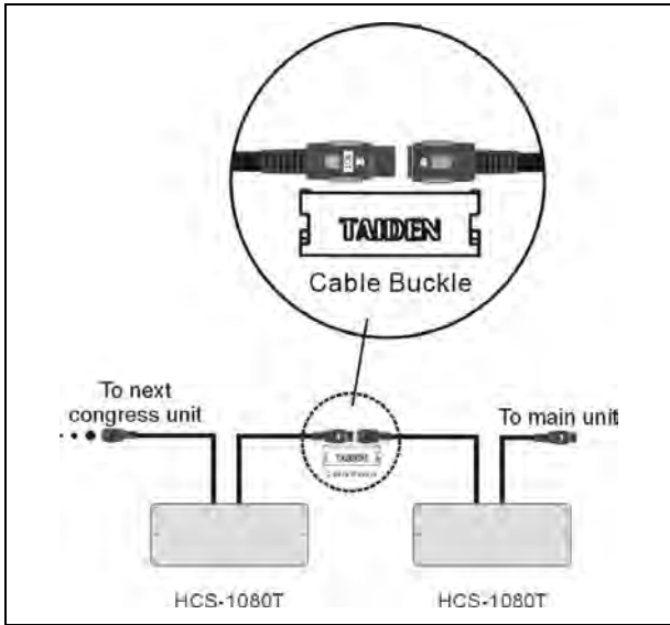
Figure 3.17.5 "Daisy-chain" connection between HCS-1080T nameplate adaptors
