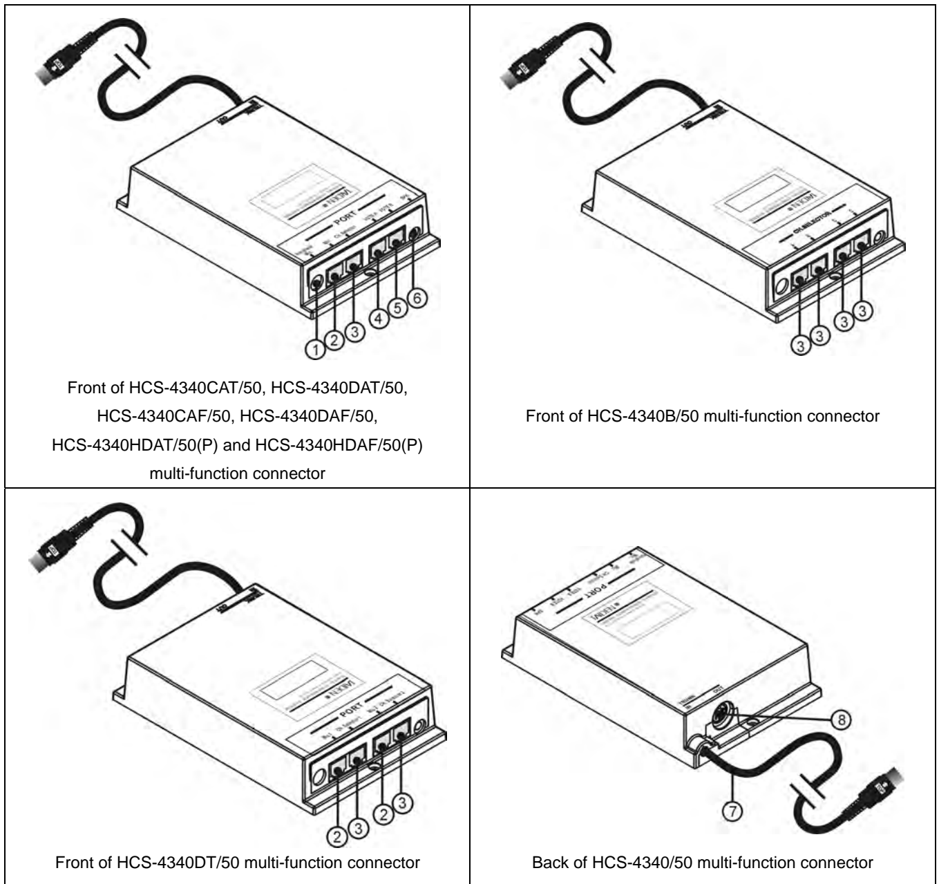
Figure 3.13.2 HCS-4340/50 series multi-function connectors
