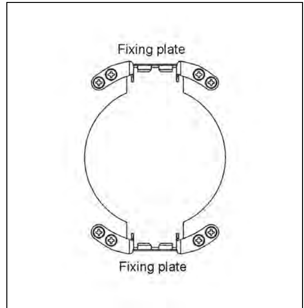
Figure 3.14.13 Diagram of the finished installation of the fixing plates of the HCS-4844/50 series flush-mounted loudspeaker
