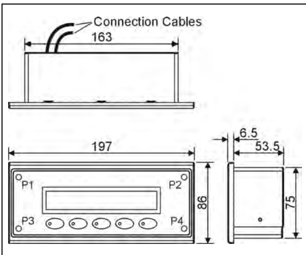
Figure 3.15.3 Dimension diagram of HCS-4368/50 series flush-mounted voting unit (unit: mm)
