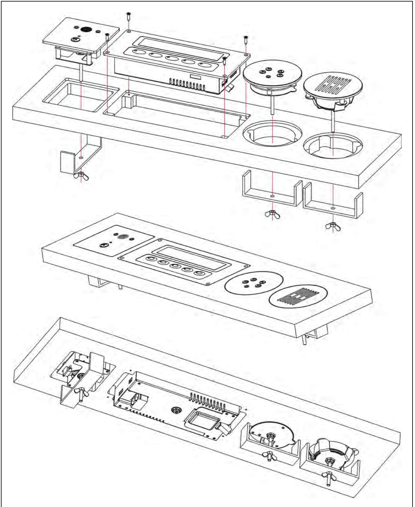
Figure 3.3.7 Installation of HCS-48U7 series flush-mounted congress unit
