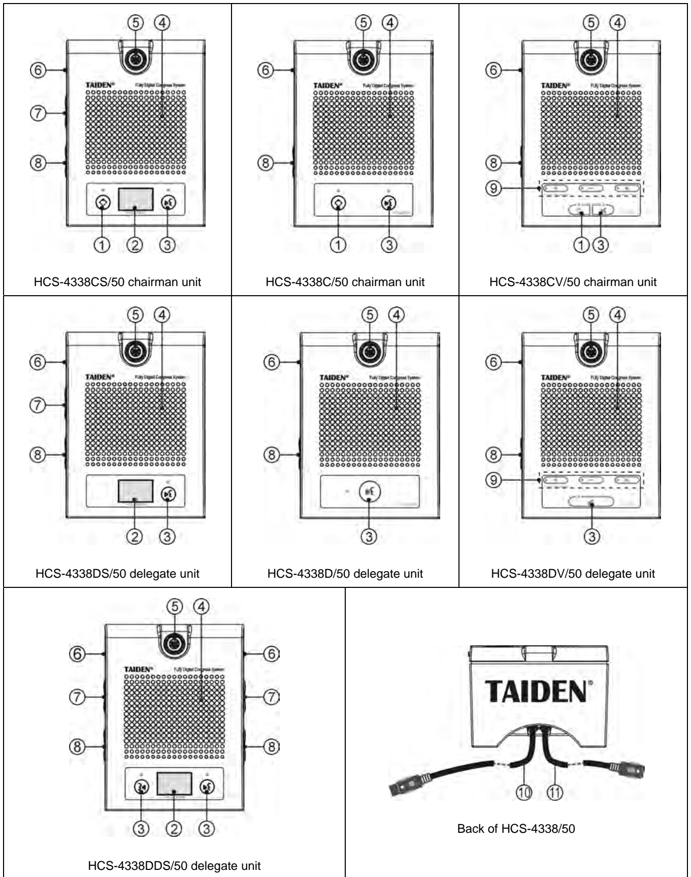
Figure 3.16.1 HCS-4338/50 series congress units
