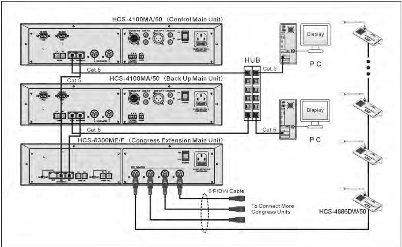
Figure 5.1.11 Dual System Main Unit Hot Spare
