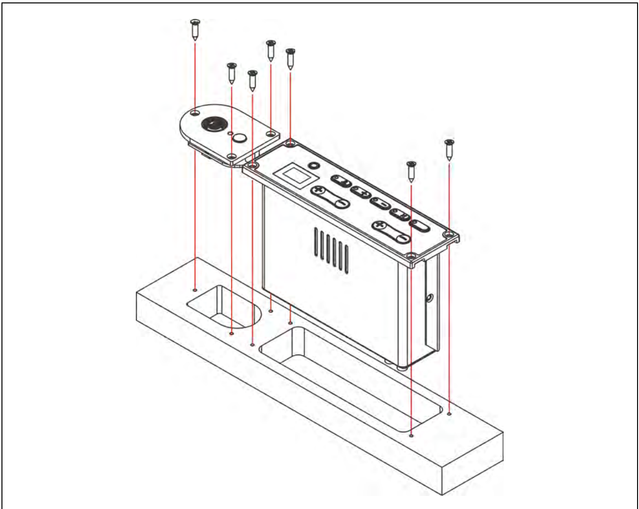
Figure 3.12.7 Installation diagram of HCS-4325/26 series congress unit with HCS-4327D/50
