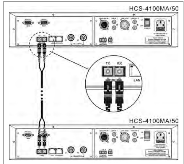
Figure 2.3.4 Connecting between CMUs via fiber cable
