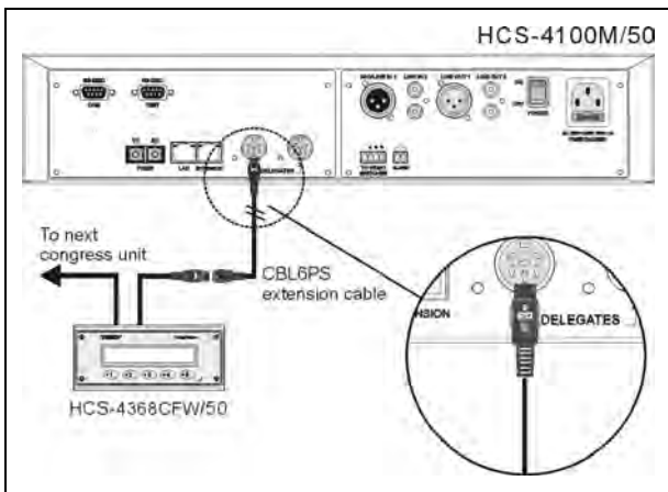
Figure 3.15.6 HCS-4368/50 series voting unit connected to the CMU/EMU
