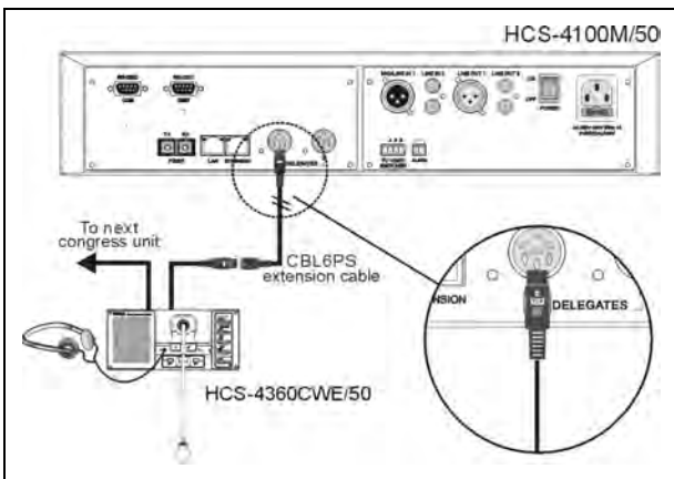
Figure 3.7.6 HCS-4360/61/62/63 series congress unit connected to the CMU/EMU
