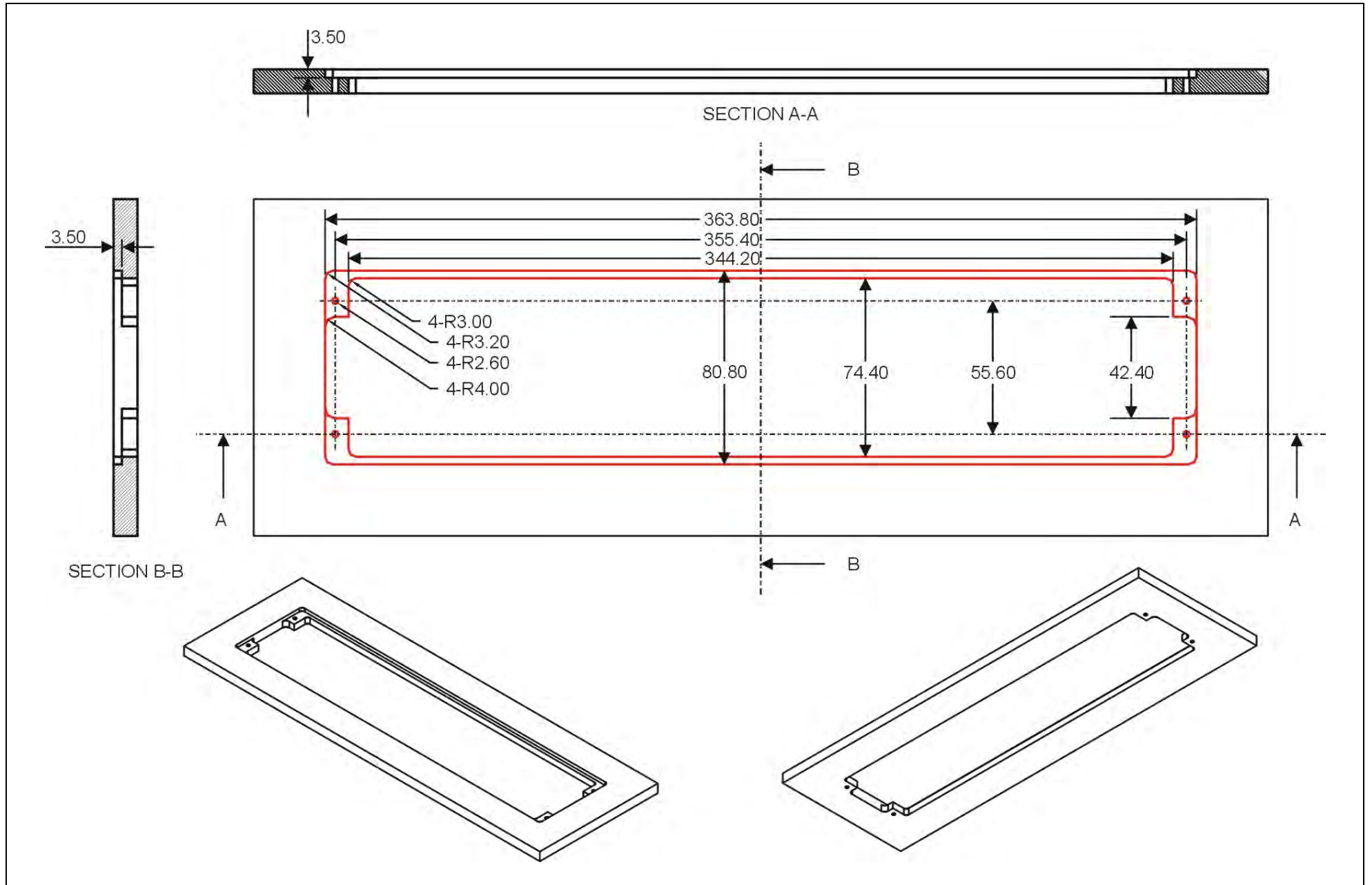
Figure 3.3.5 Cutout of HCS-48U9DFFF flush-mounted congress unit (unit: mm)
