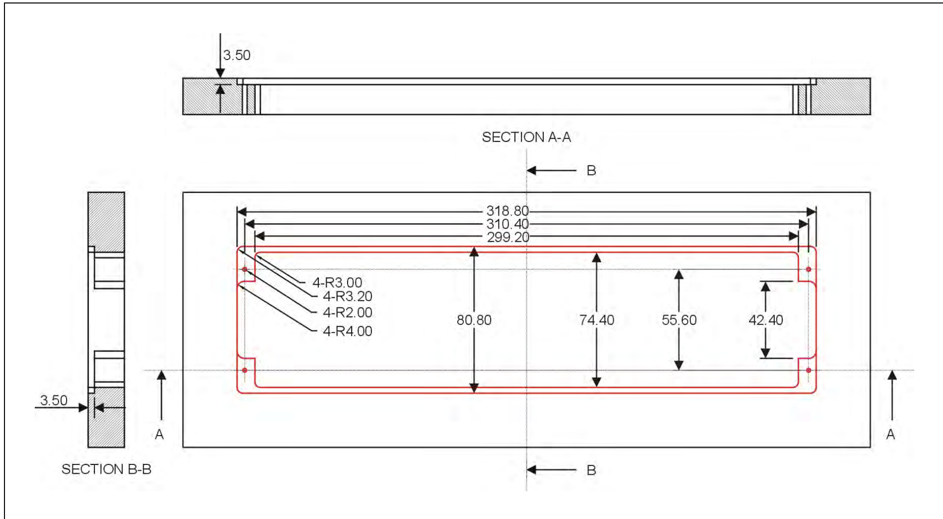
Figure 3.3.4 Cutout of HCS-48U9 series flush-mounted congress unit (unit: mm) (except HCS-48U9DFFF)
