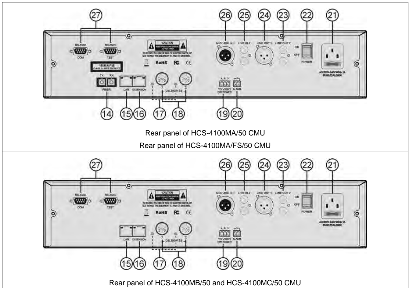
Figure 2.1.2 Rear panel of HCS-4100M/50 CMU
