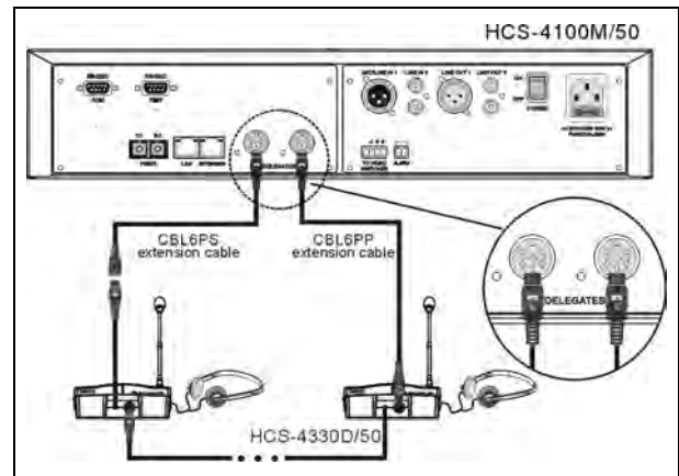
Figure 3.11.3 “Closed Loop - Daisy Chain” connection between the CMU and HCS-4330/50 series congress units
