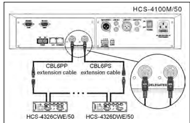
Figure 3.12.10 “Closed Loop - Daisy Chain” connection between the CMU and HCS-4325/26 series congress units
