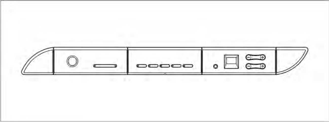
Figure 3.14.7 Diagram showing the finished installation of the HCS-4841N/42N/43N series congress units
