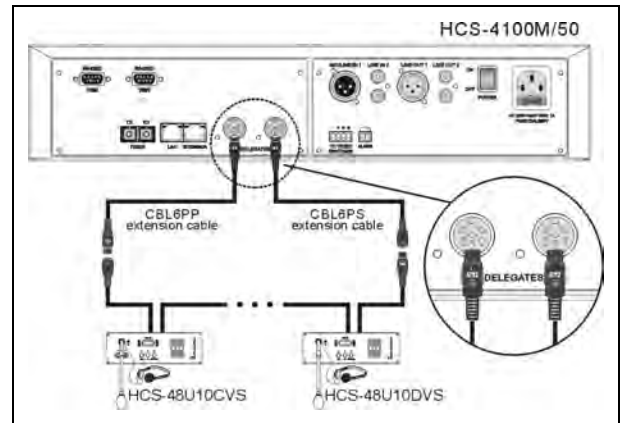
Figure 3.4.5 “Closed Loop - Daisy Chain” connection between the CMU and HCS-48U10 series congress units
