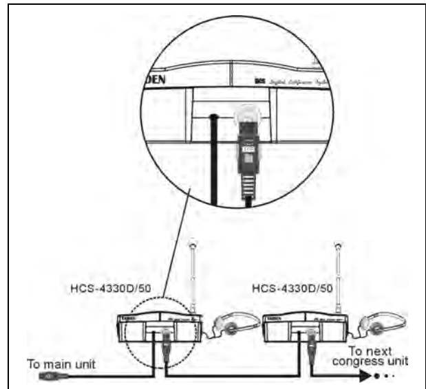
Figure 3.11.4 “Daisy-chain” connection between HCS-4330/50 series congress units
