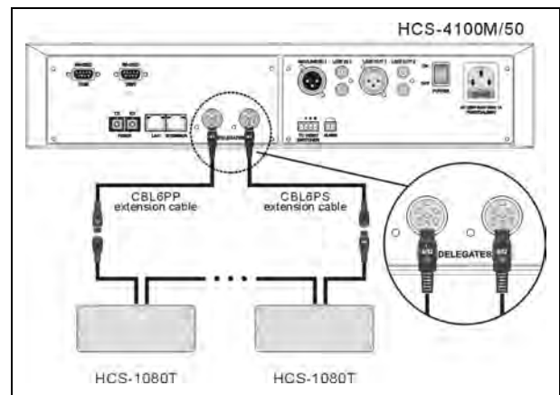
Figure 3.17.4 “Closed Loop - Daisy Chain” connection between the CMU and HCS-1080T
