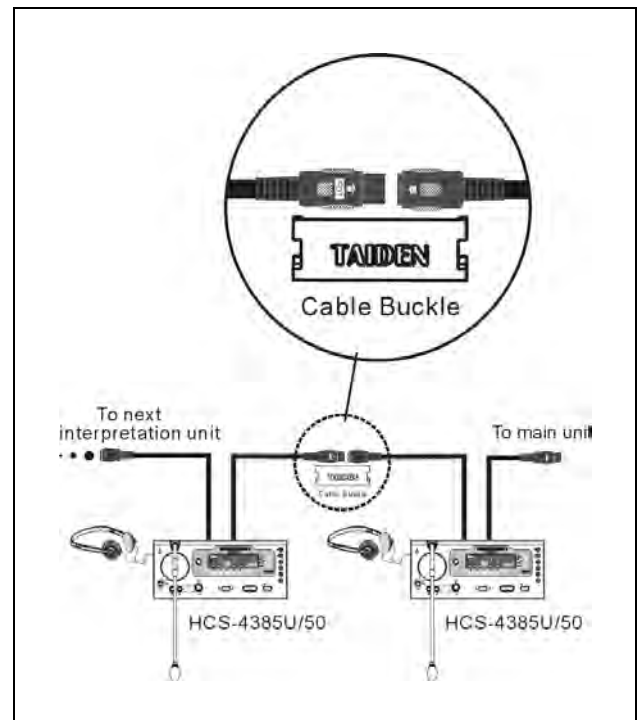
Figure 4.3.3 “Daisy-chain” connection between HCS-4385U/50 interpreter units
