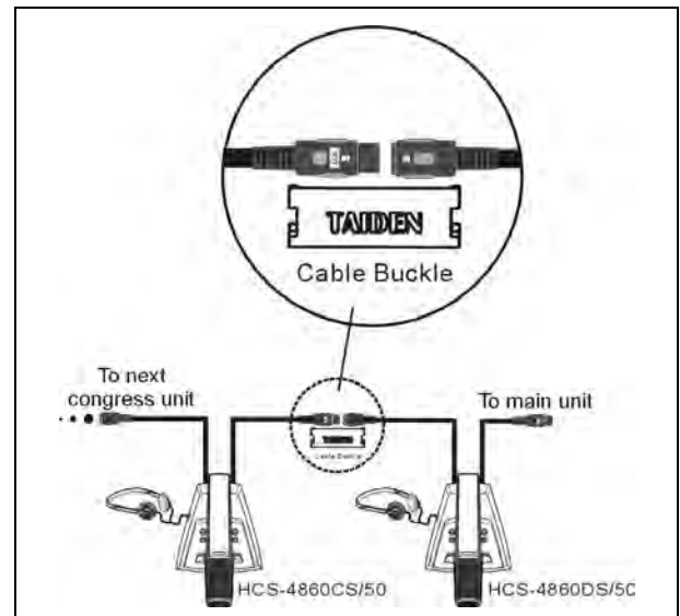
Figure 3.9.4 “Daisy-chain” connection between HCS-4860/50 series congress units
