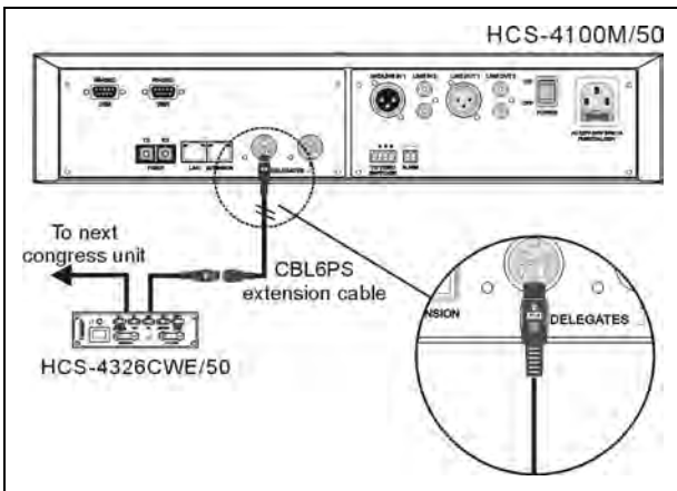
Figure 3.12.9 HCS-4325/26 series congress unit connected to the CMU/EMU
