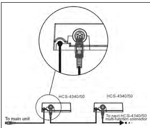
Figure 3.14.17 “Daisy-chain” connection between HCS-4340/50 series multi-function connectors
