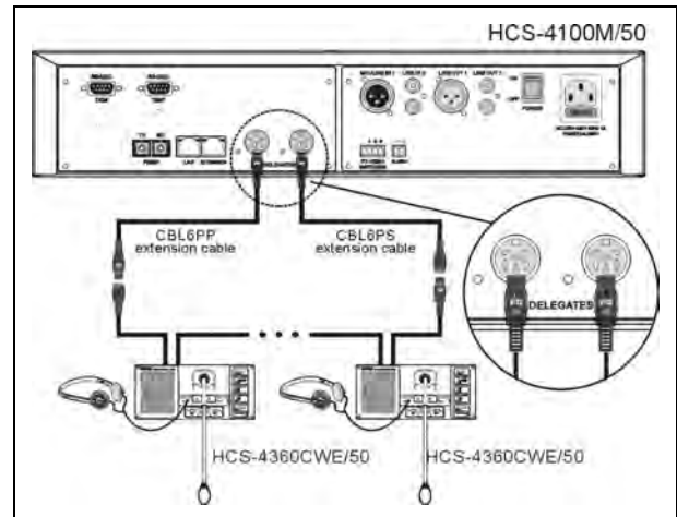
Figure 3.7.7 “Closed Loop - Daisy Chain” connection between the CMU and HCS-4360/61/62/63 series congress units
