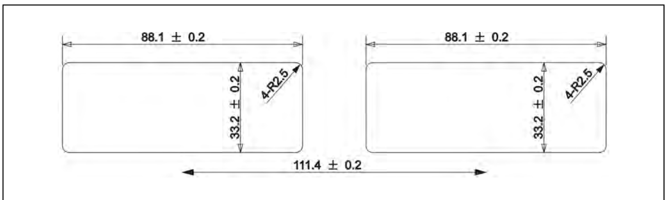
Figure 3.14.5 Positioning and assembly installation diagram of several HCS-4841N/42N/43N series congress units (unit: mm)
