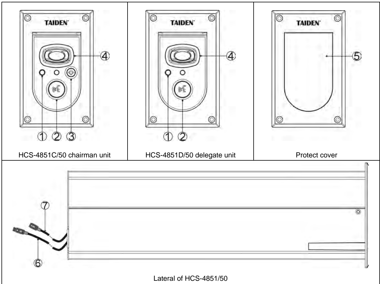
Figure 3.10.1 HCS-4851/50 series congress units
