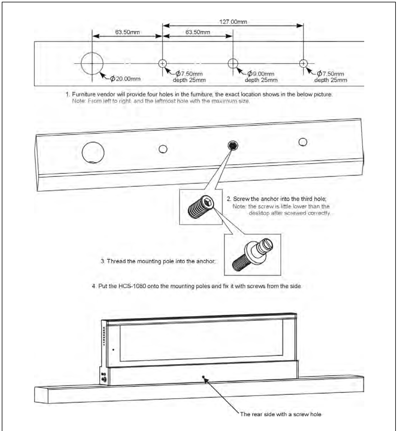
Figure 3.17.2 Installation of HCS-1080 electronic nameplate
