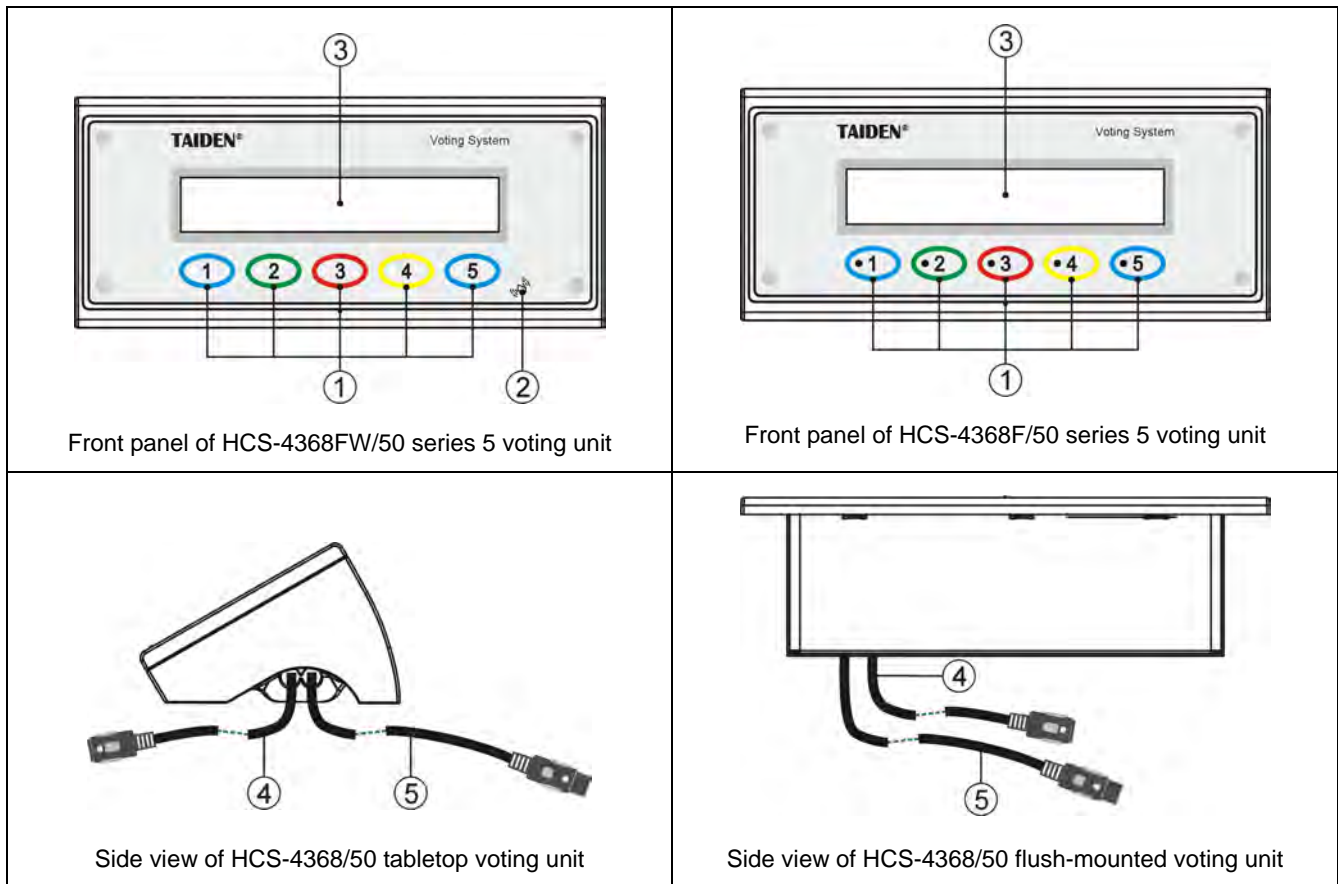
Figure 3.15.1 HCS-4368/50 series wired voting units
