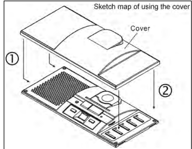
Figure 3.7.4 Installation diagram of the protective cover of HCS-4360/61/62/63 series congress unit
