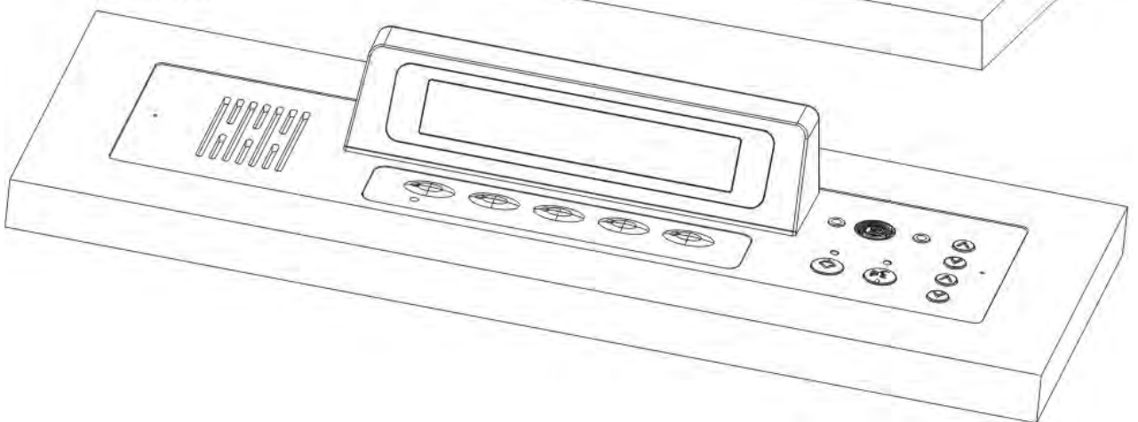
Figure 3.3.8 Installation of HCS-48U8 series and HCS-48U9 series flush-mounted congress unit
