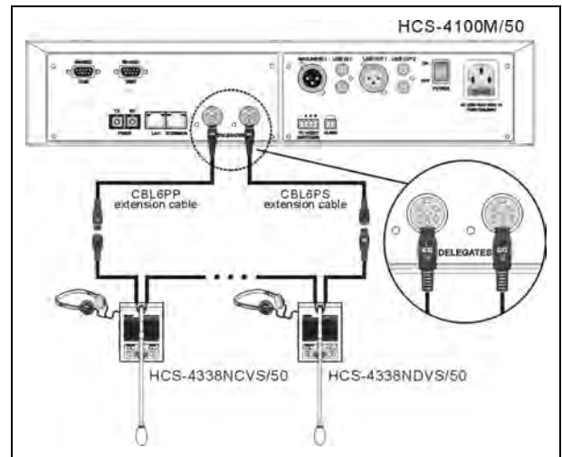
Figure 3.8.3 “Closed Loop - Daisy Chain” connection between the CMU and HCS-4338N/50 series congress units
