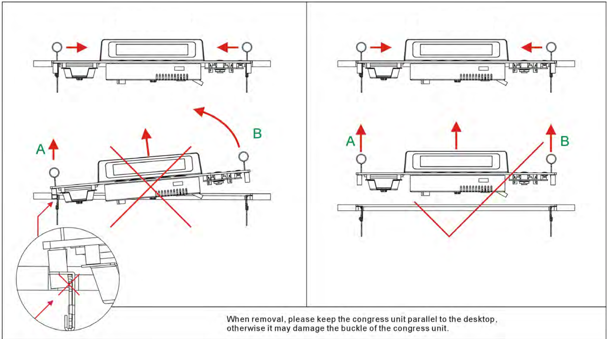
Figure 3.3.12 Disassembly caution of HCS-48U8 and HCS-48U9 series flush-mounted congress unit
