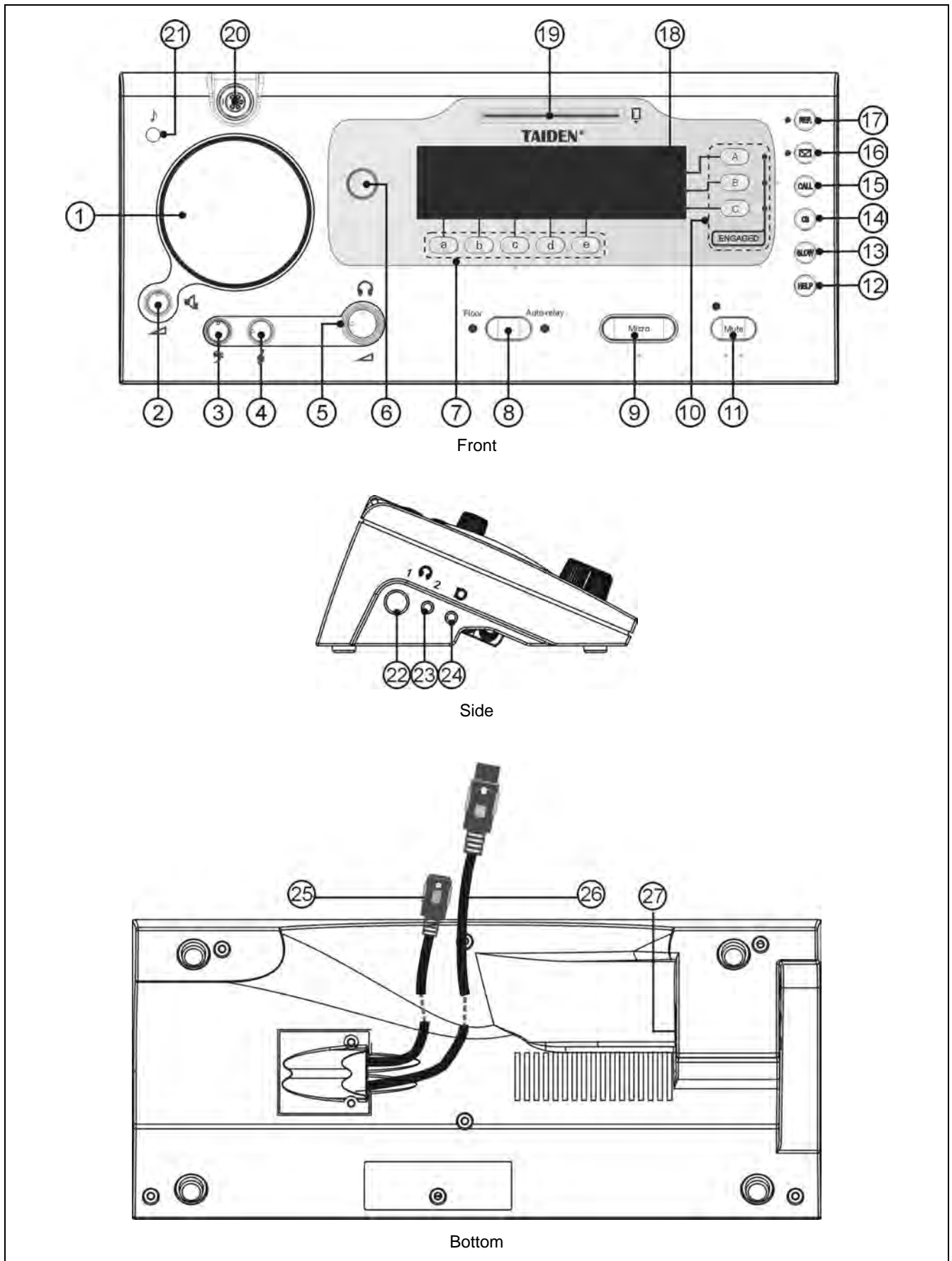
Figure 4.1.1 HCS-4385U/50 Interpreter unit
