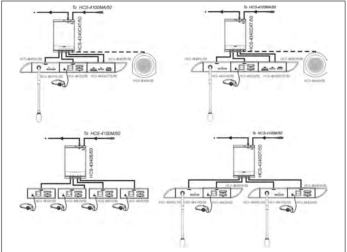
Figure 3.14.18 Multi-function connector connected to HCS-4841/42/43 series congress units
