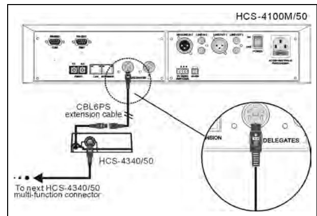
Figure 3.13.4 HCS-4340/50 series multi-function connector connected to the CMU/EMU
