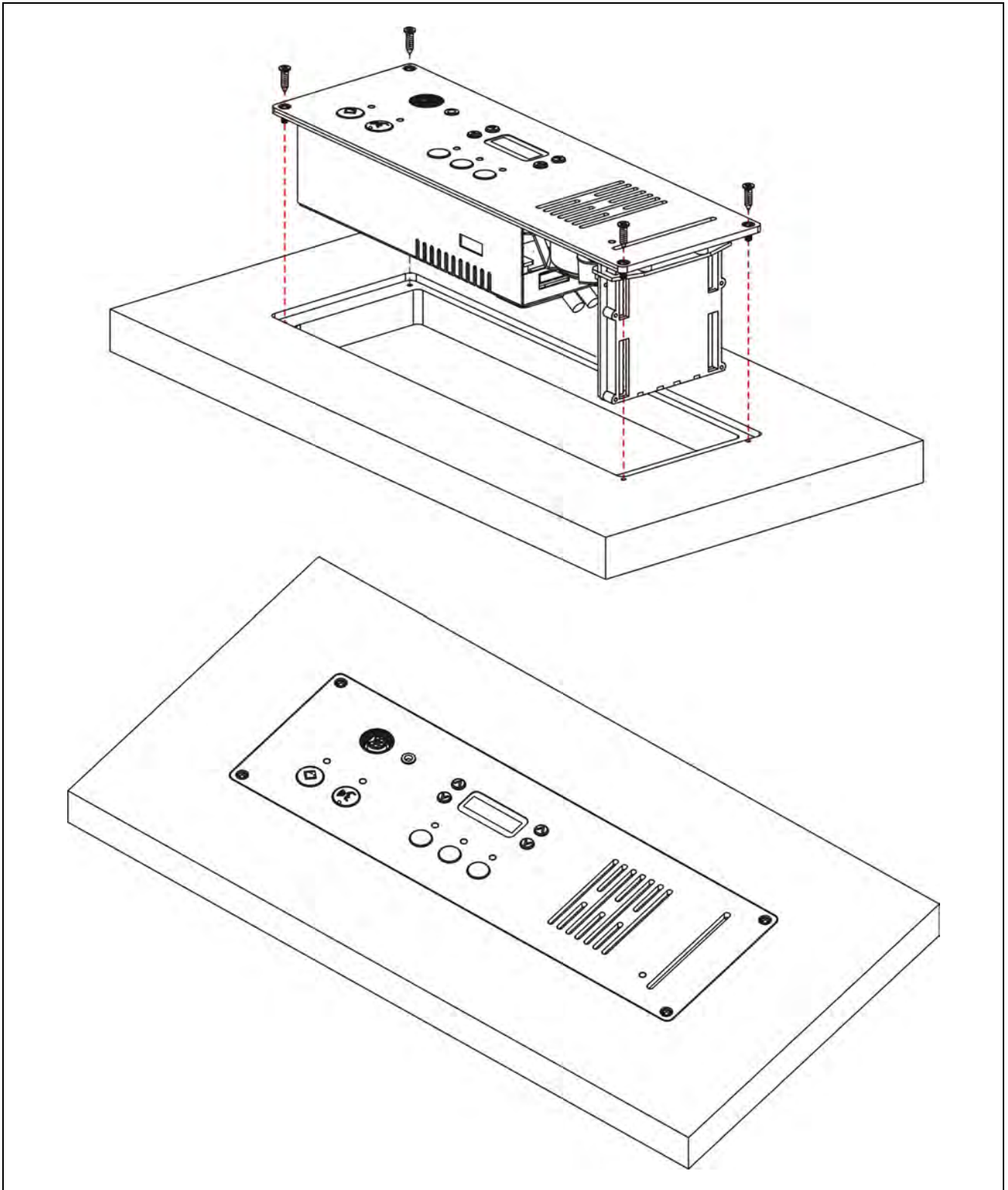
Figure 3.4.3 Installation of HCS-48U10 series congress unit
