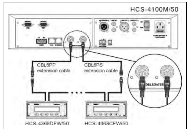
Figure 3.15.7 “Closed Loop - Daisy Chain” connection between the CMU and HCS-4368/50 series voting units
