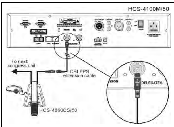
Figure 3.9.2 HCS-4860/50 series congress unit connected to the CMU/EMU
