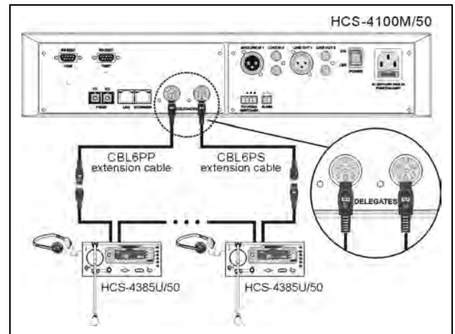
Figure 4.3.2 “Closed Loop - Daisy Chain” connection between the CMU and HCS-4385U/50 interpreter units
