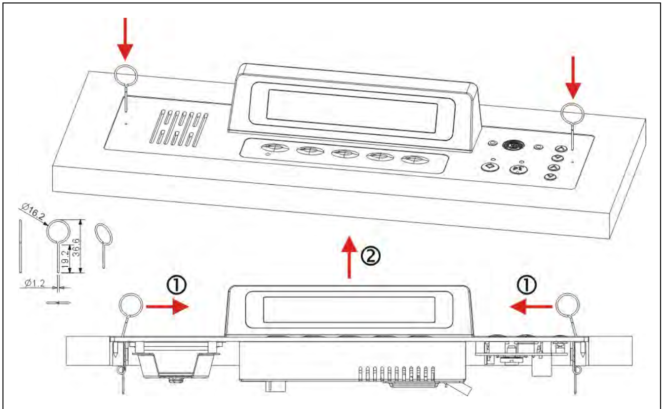
Figure 3.3.10 Disassembly of HCS-48U8 and HCS-48U9 series flush-mounted congress unit (method a)
