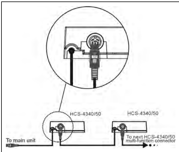
Figure 3.13.6 “Daisy-chain” connection between HCS-4340/50 series multi-function connectors
