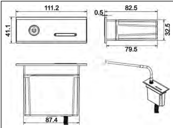
Figure 3.14.2 Dimension diagram of HCS-4841(N)/42N/43N series congress unit (unit: mm)
