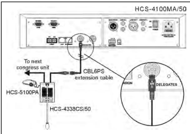
Figure 3.16.2 HCS-4338/50 series congress unit connected to the CMU/EMU
