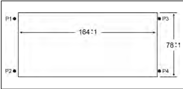
Figure 3.15.2 Fixing hole positioning diagram of HCS-4368/50 series flush-mounted voting unit (unit: mm)
