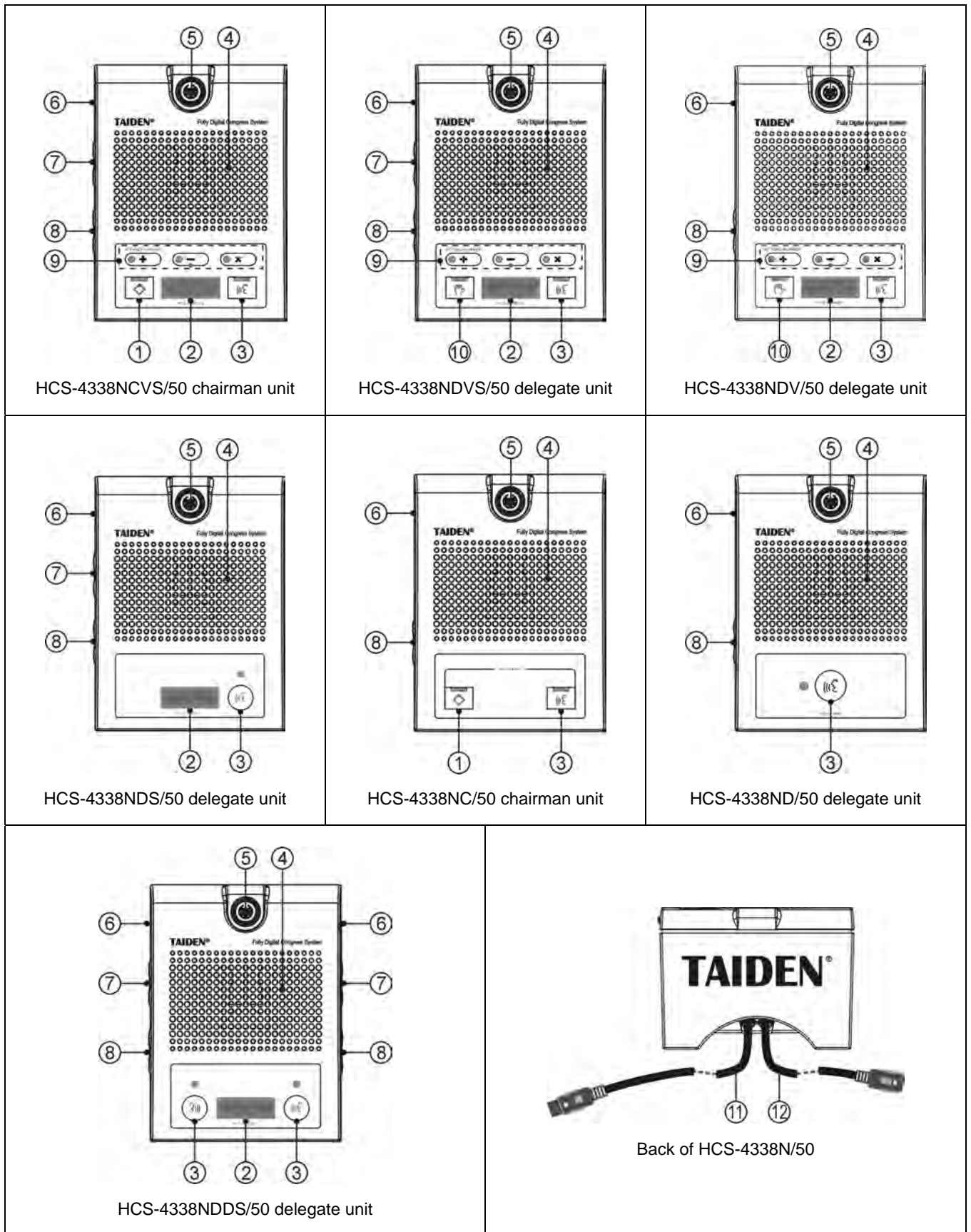
Figure 3.8.1 HCS-4338N/50 series congress units
