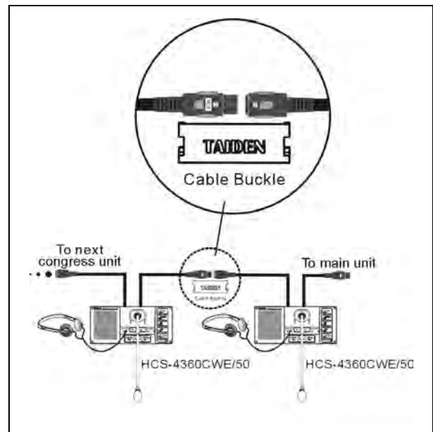
Figure 3.7.8 “Daisy-chain” connection between HCS-4360/61/62/63 series congress units
