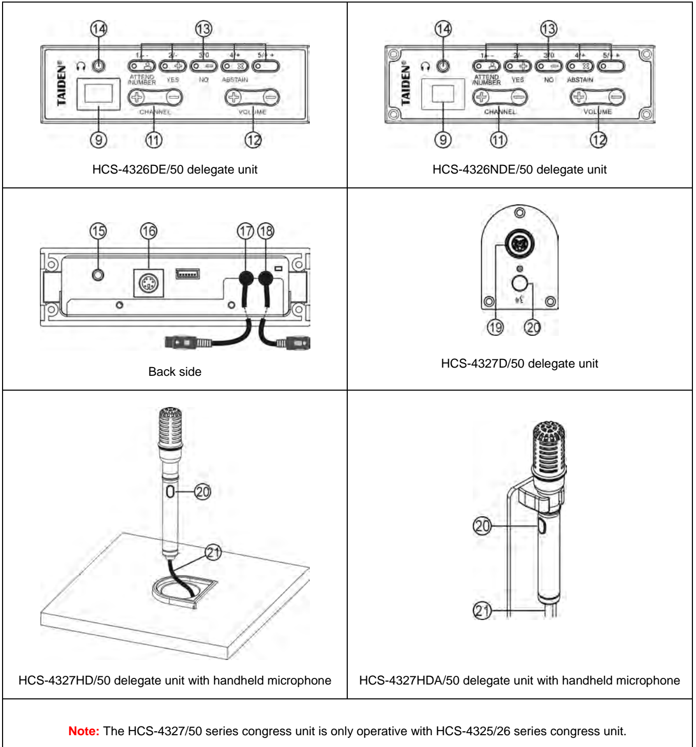
Figure 3.12.1 HCS-4325/26/27 series congress units
