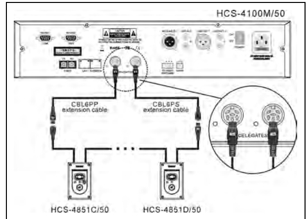
Figure 3.10.3 “Closed Loop - Daisy Chain” connection between the CMU and HCS-4851/50 series congress units
