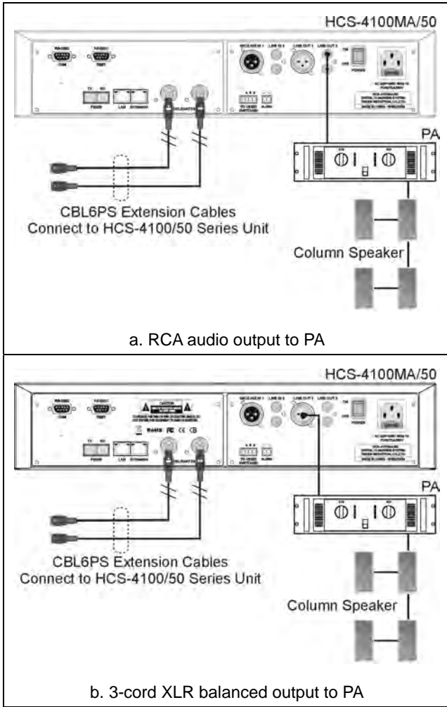
Figure 2.3.3 CMU connecting to PA
