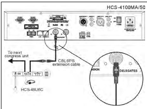
Figure 3.2.15 Multi-function connector connected to the CMU/EMU
