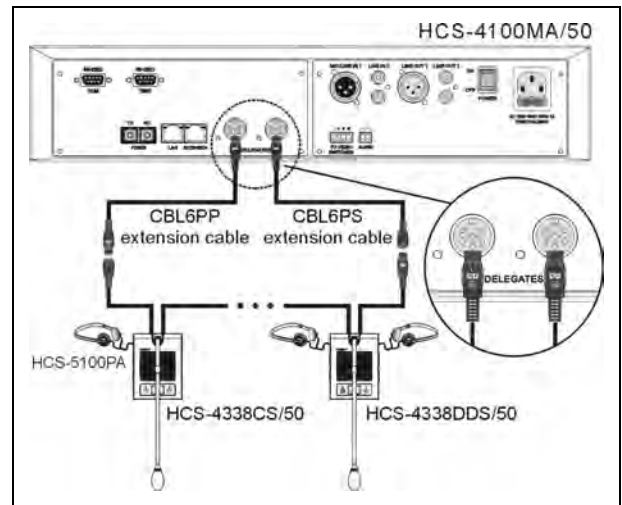
Figure 3.16.3 “Closed Loop - Daisy Chain” connection between the CMU and HCS-4338/50 series congress units
