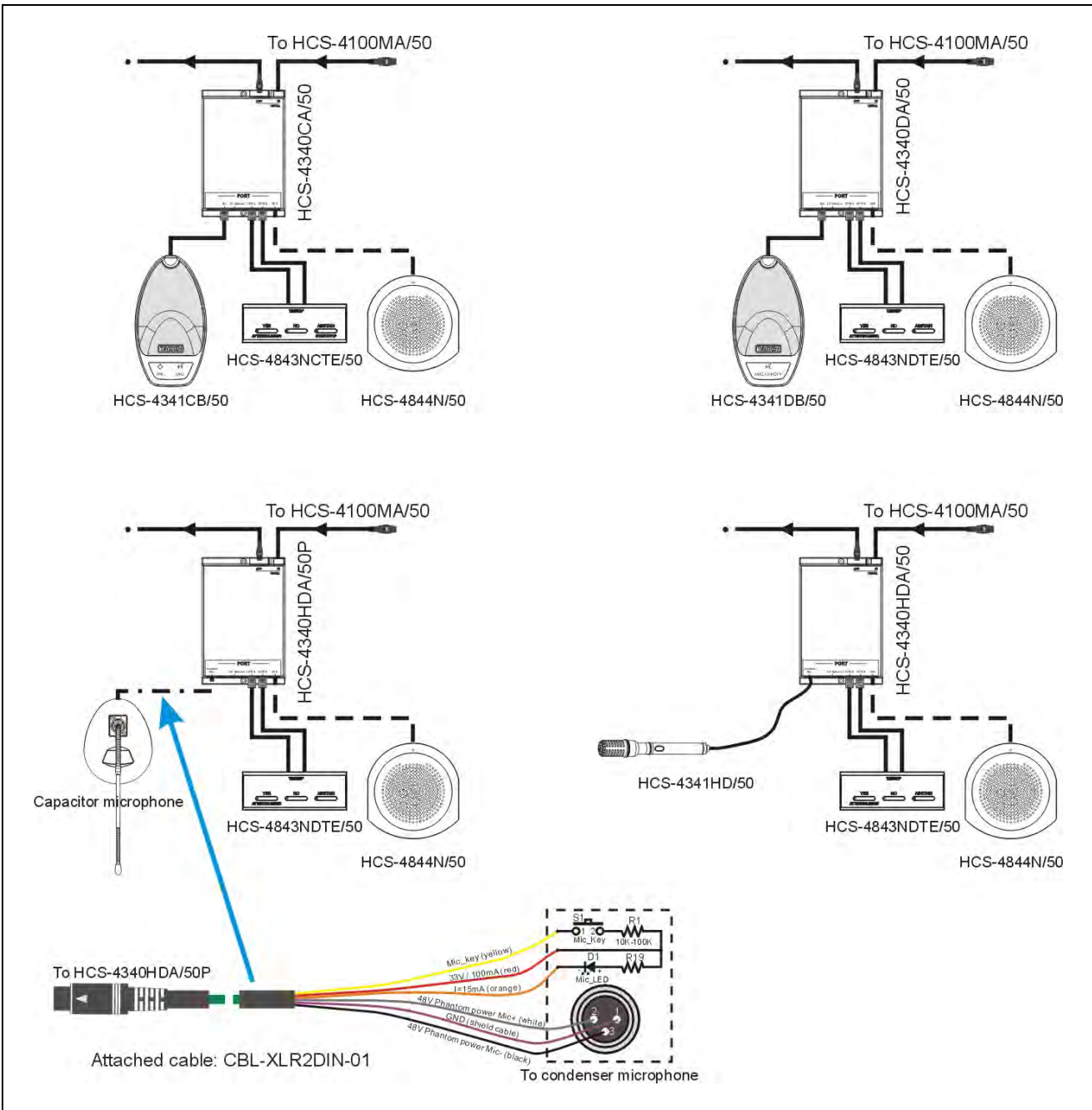
Figure 3.13.7 Multi-function connector connected to the HCS-4341/50 series congress unit
