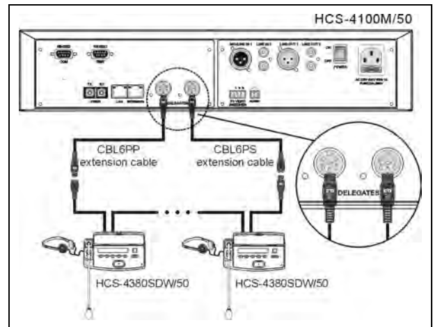
Figure 3.6.3 “Closed Loop - Daisy Chain” connection between the CMU and HCS-4380/82/70/71 series congress units
