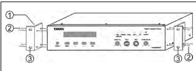
Figure 2.2.1 Installation of the CMU
