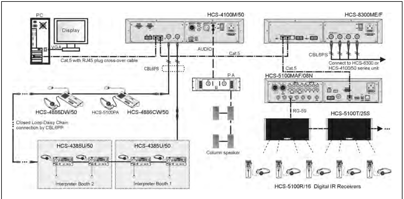
Figure 5.1.6 Congress main unit connecting to digital infrared language distribution system via HCS-5100MAF/N
