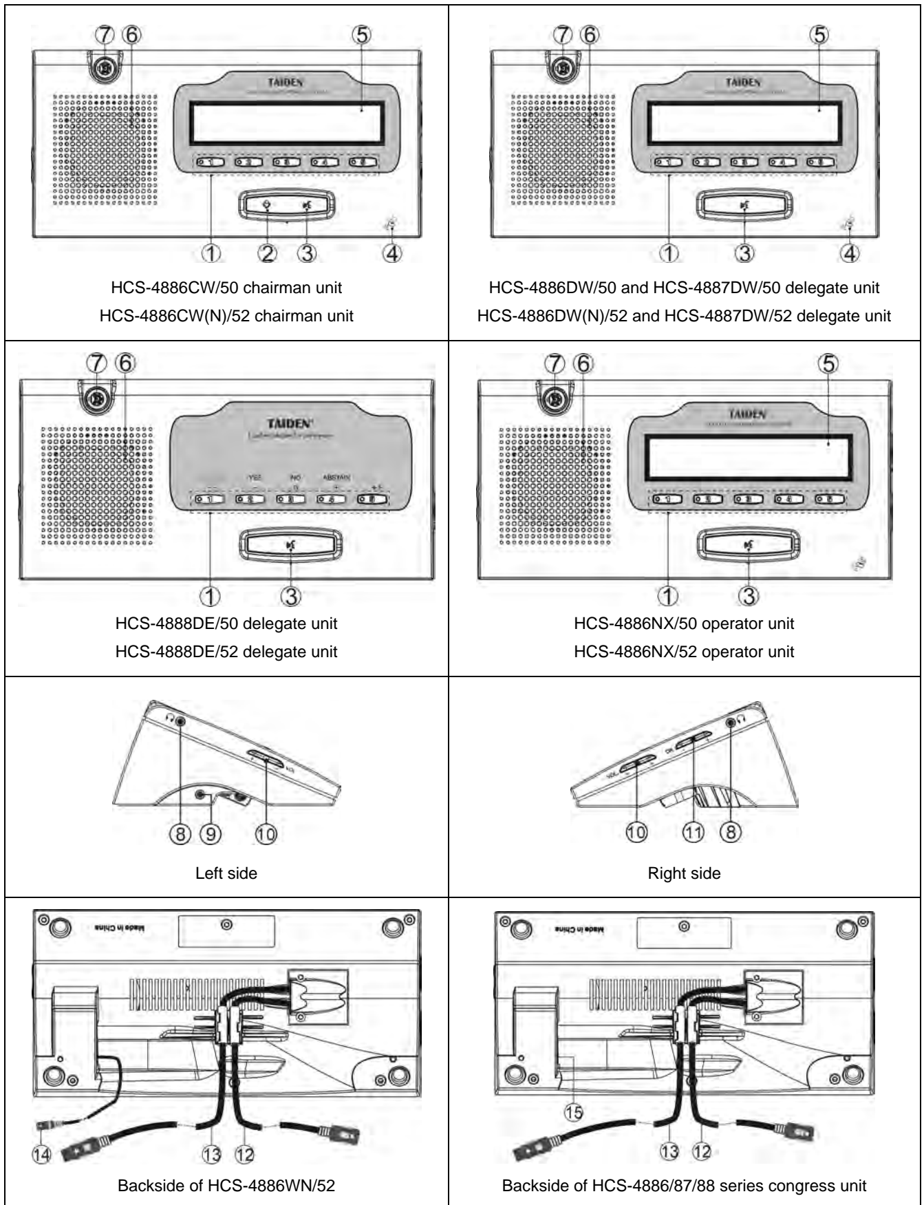
Figure 3.5.1 HCS-4886/87/88 series congress units
