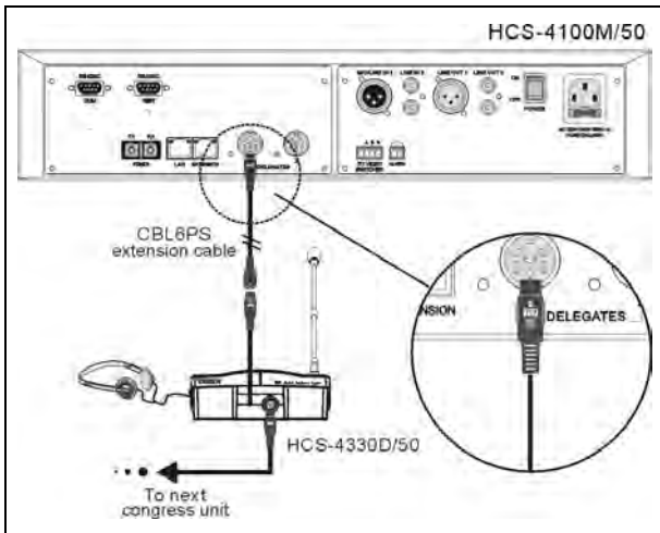
Figure 3.11.2 HCS-4330/50 series congress unit connected to the CMU/EMU
