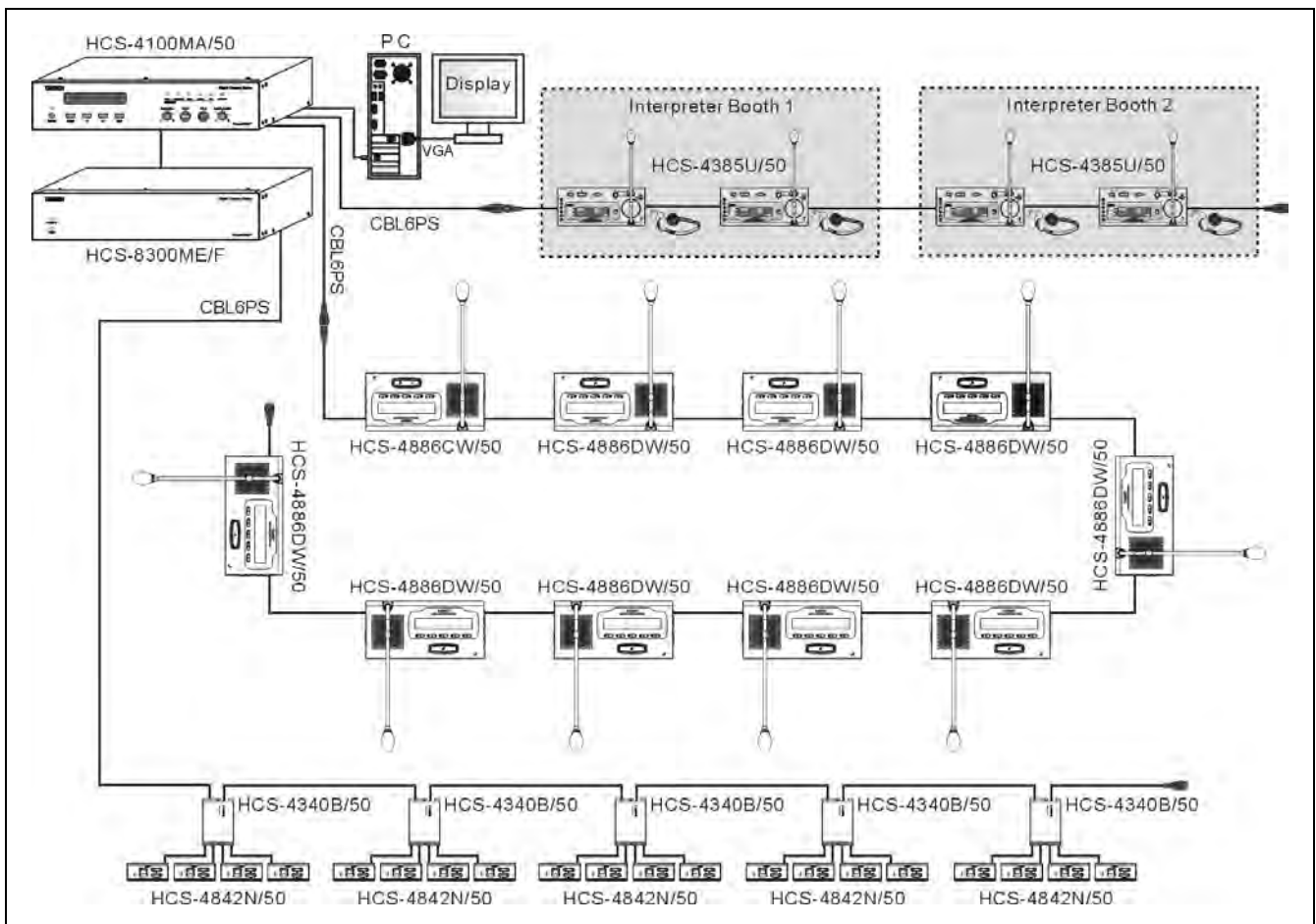
Figure 1.1.1 System overview
