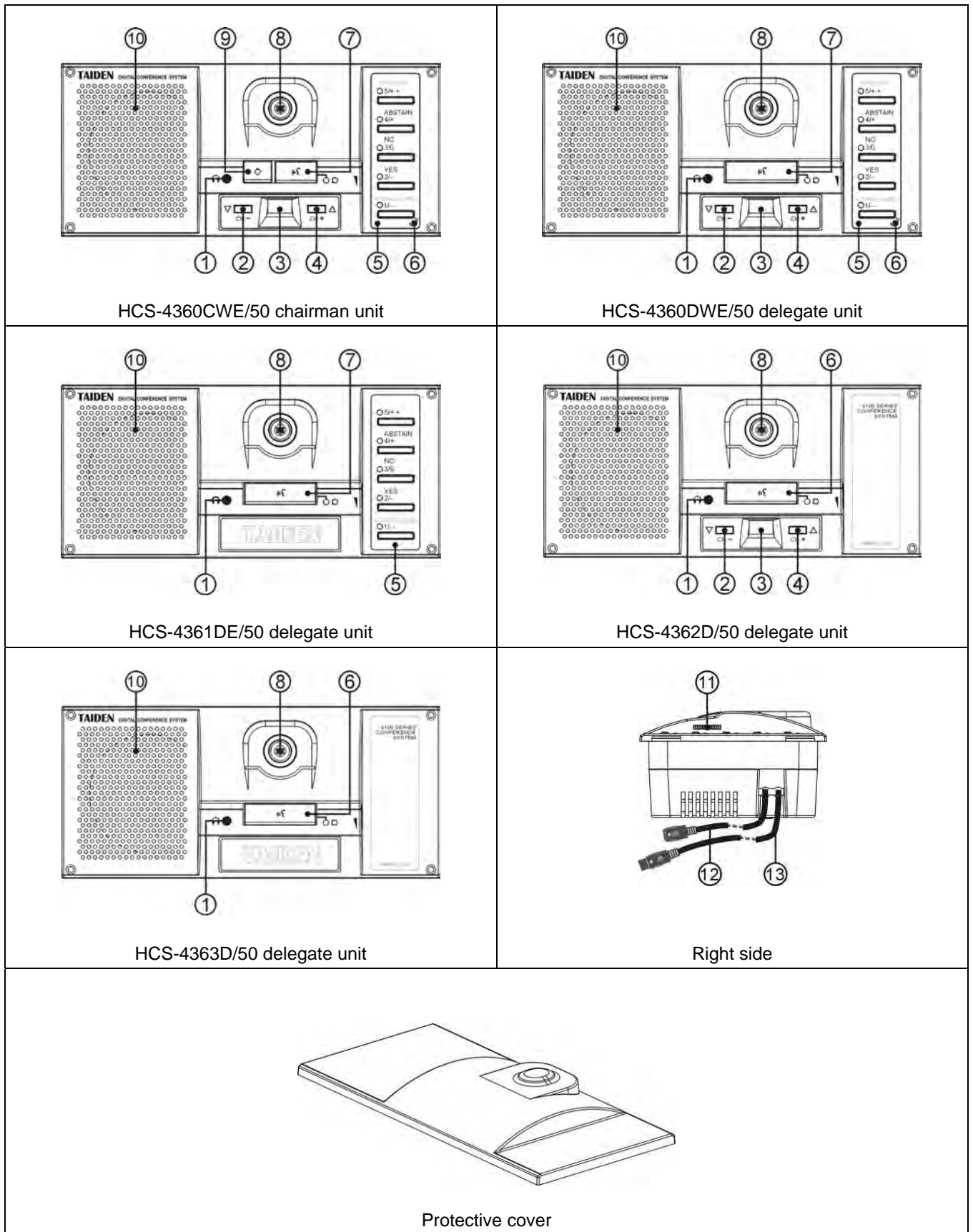
Figure 3.7.1 HCS-4360/61/62/63 series congress units
