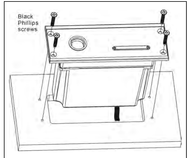
Figure 3.14.4 Installation diagram of HCS-4841(N)/42N/43N series congress unit (unit: mm)
