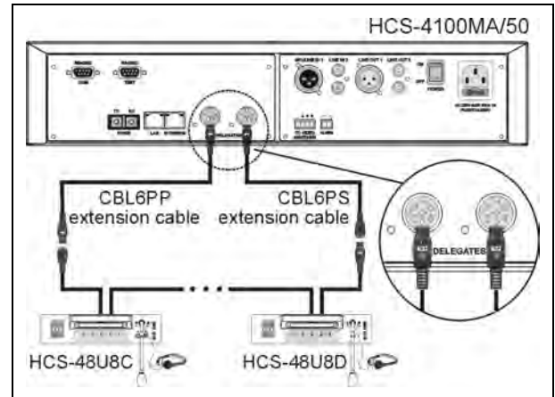
Figure 2.3.2 “Closed Loop - Daisy Chain” connection topology
