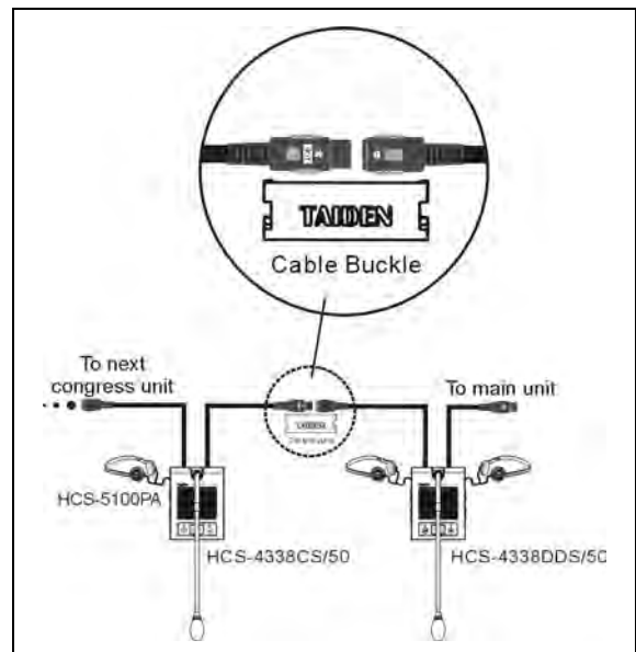
Figure 3.16.4 “Daisy-chain” connection between HCS-4338/50 series congress units
