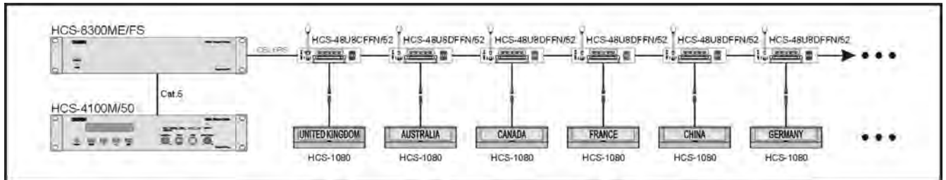
Figure 3.17.6 Connection of HCS-1080 E-ink Nameplate (with HCS-48U8 series congress unit)
