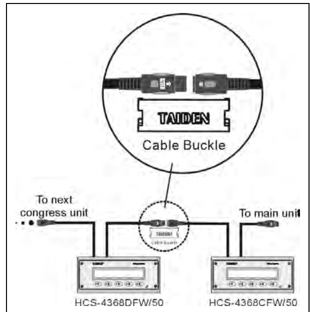
Figure 3.15.8 “Daisy-chain” connection between HCS-4368/50 series voting units
