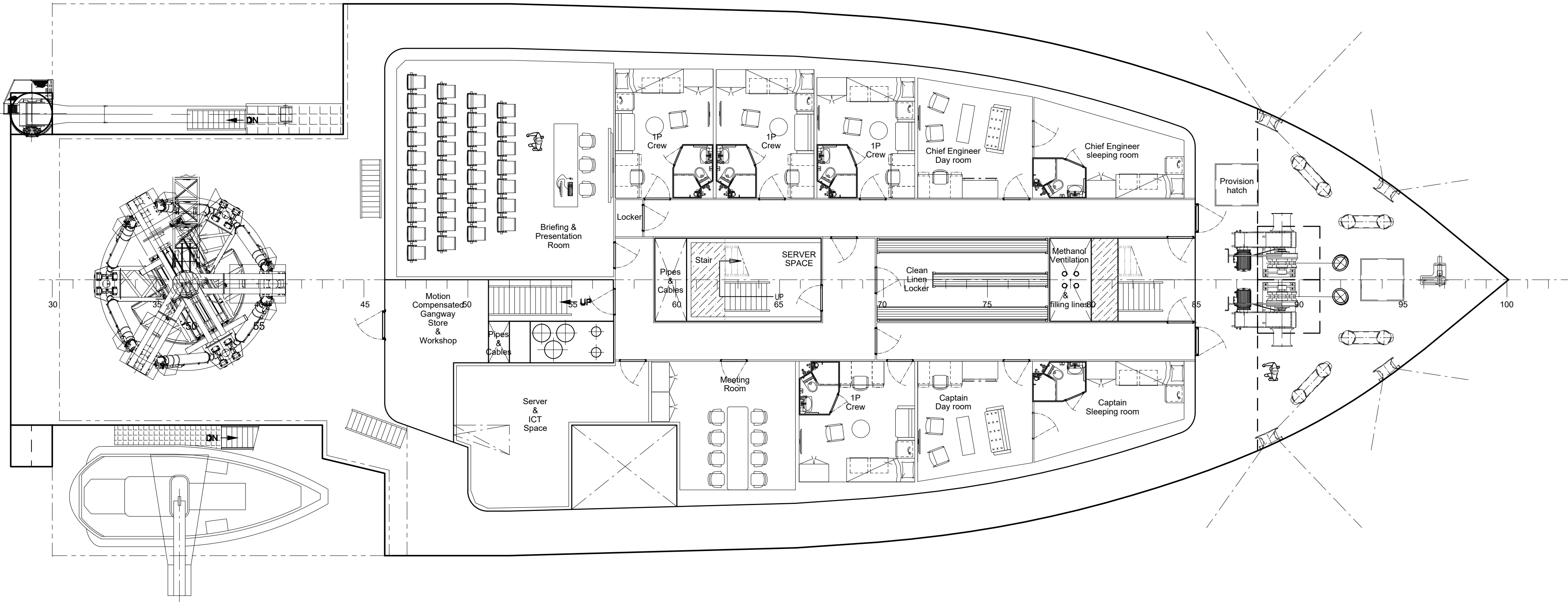
12500 A.B. - FORECASTLE DECK
