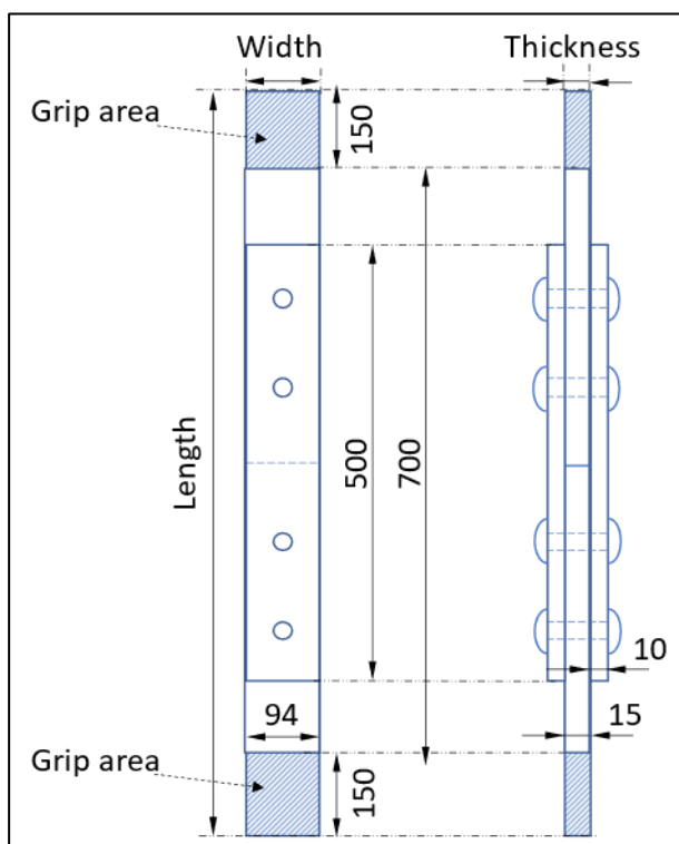
Figure 2: Dimensions of a typical specimen on which fatigue tests are performed in the DBL. Shown is a riveted joint connection with dimensions indicated in [mm].
