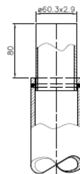
Detail Top (1:3)
