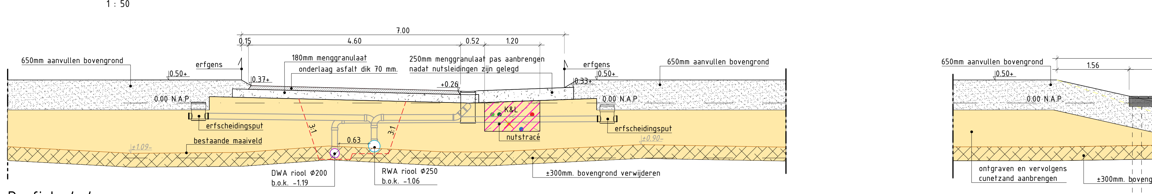
Profiel 4-4
