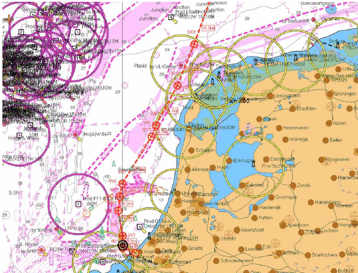
Figure 3 ECDIS overview
