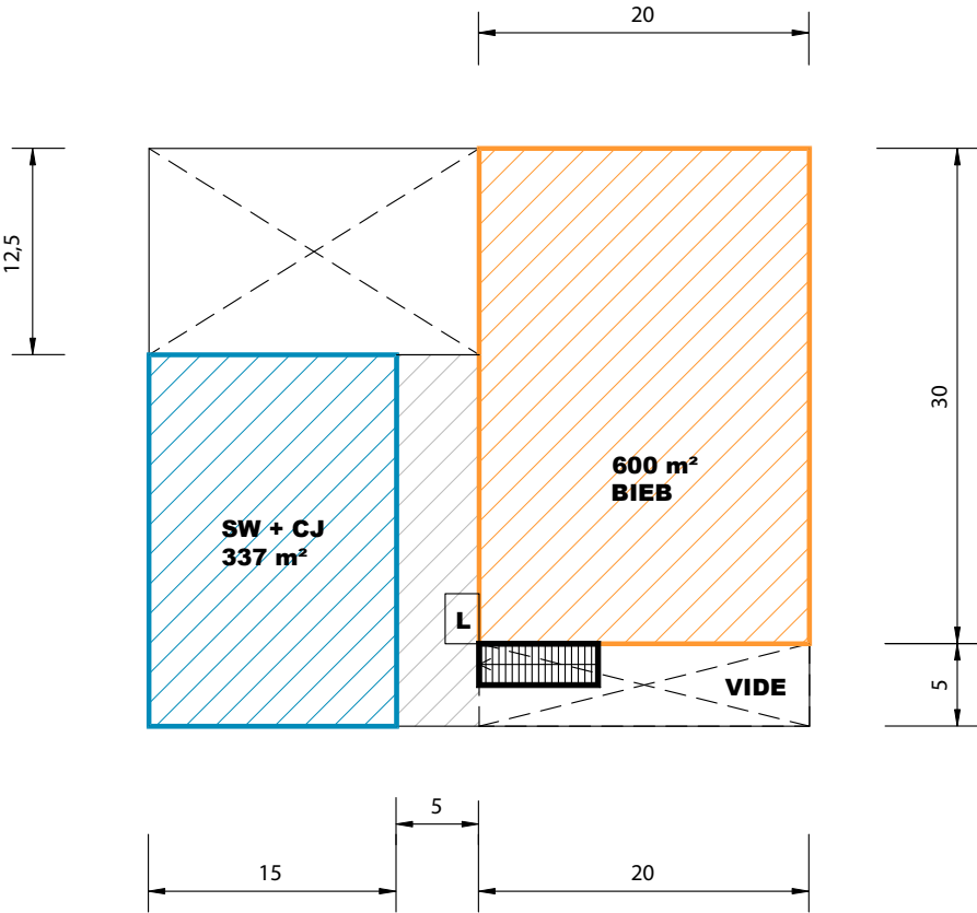
VERDIEPING / 936 m²
