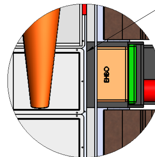
DETAIL F SCALE 1 : 10
