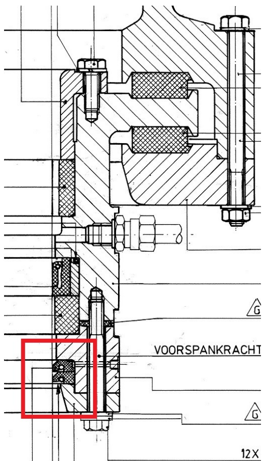
OBT-00141 Conserveringsolie-installatie rubberen ring
