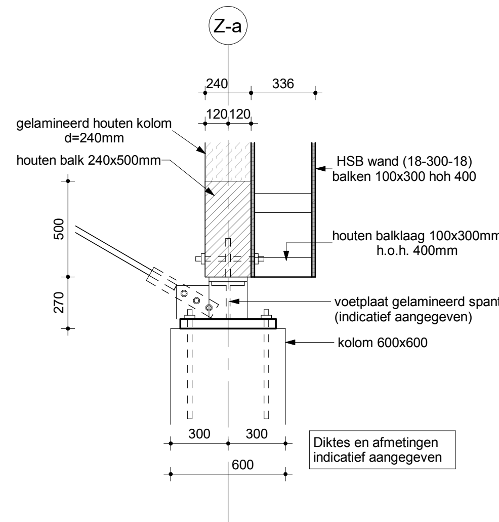
z.05 Detail
