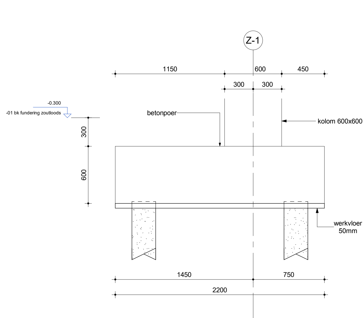
z.01 Detail
