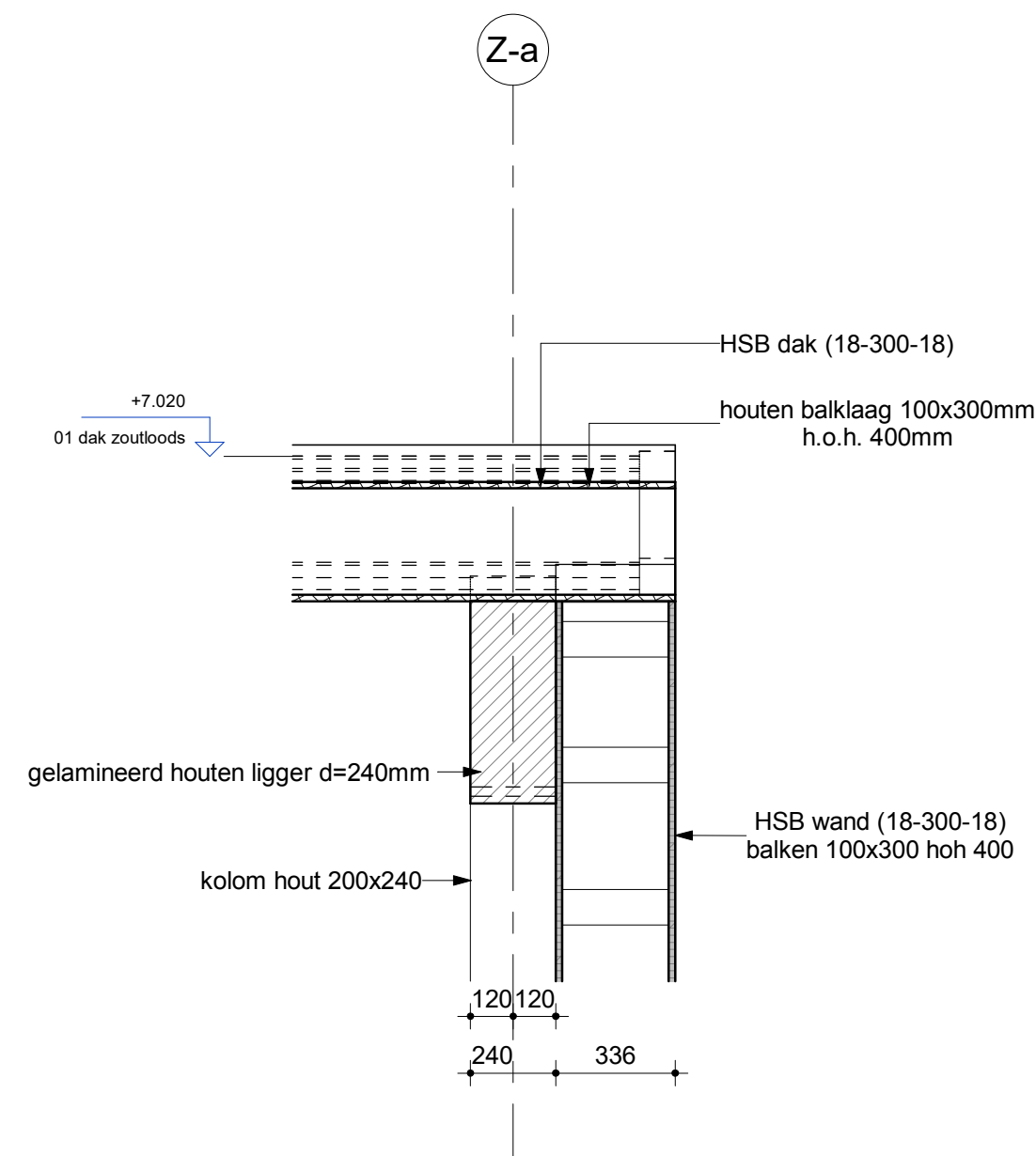
z.12 Detail
