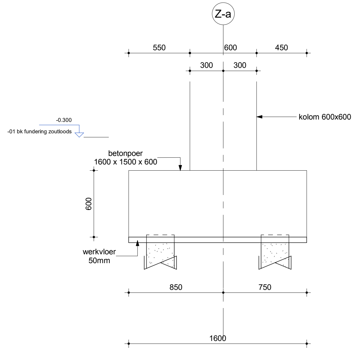
z.02 Detail
