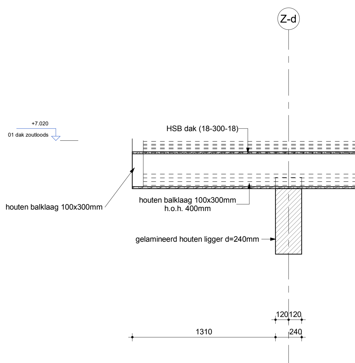
z.13 Detail
