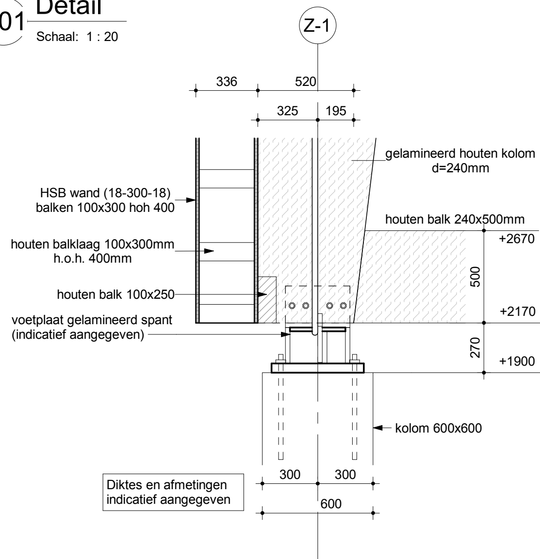
z.04 Detail
