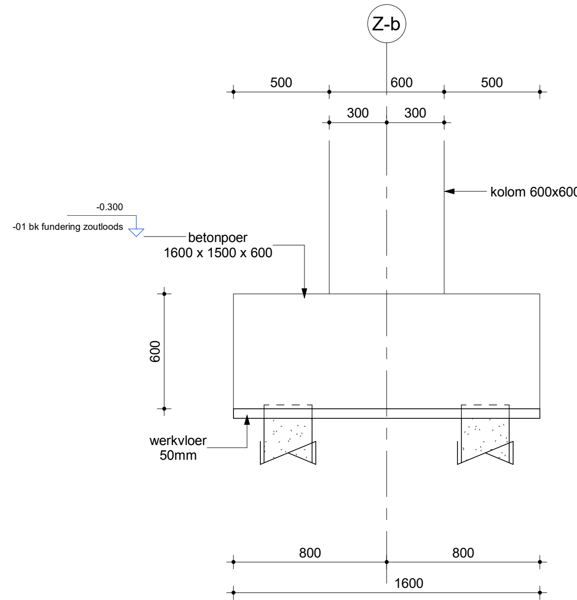
z.03 Detail
