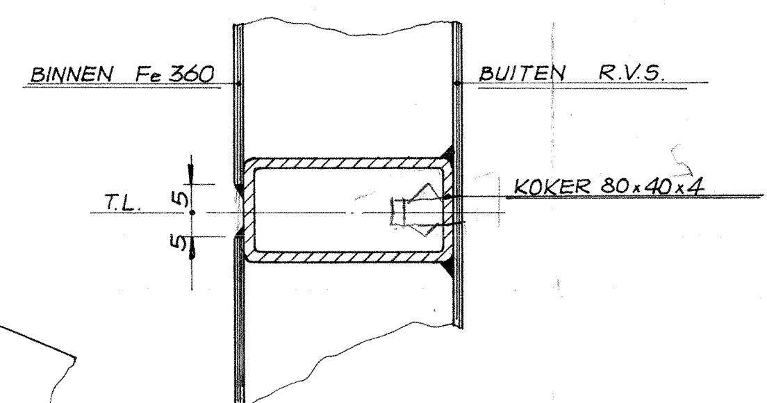
DETAIL III
