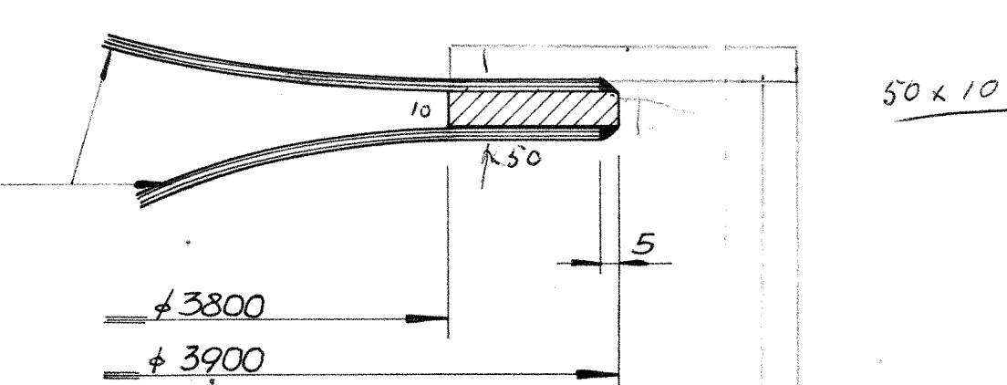
DETAIL IV
