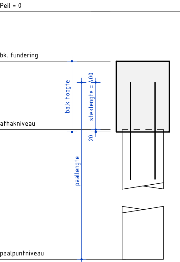
Paaldetail prefab
