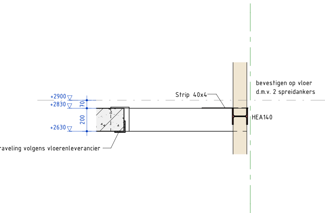
Detail 2.08
