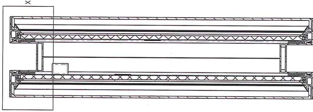
SECTION W-W
