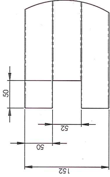
DETAIL V SCALE 1:4
