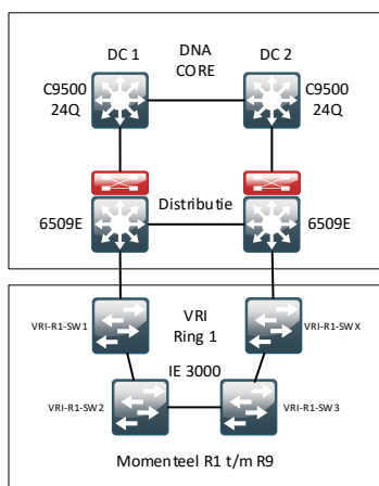
Figuur 7: Configuratie VRI switches
