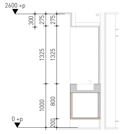
make-up nis doorsnede
