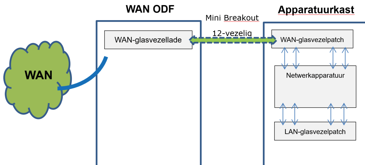
Figuur 7: Principeschema Inter-rack bekabeling WAN-LAN
