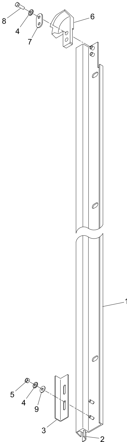
Figure 14 PORTAL SEAL ASSEMBLY, RIGHT (20104022001)
