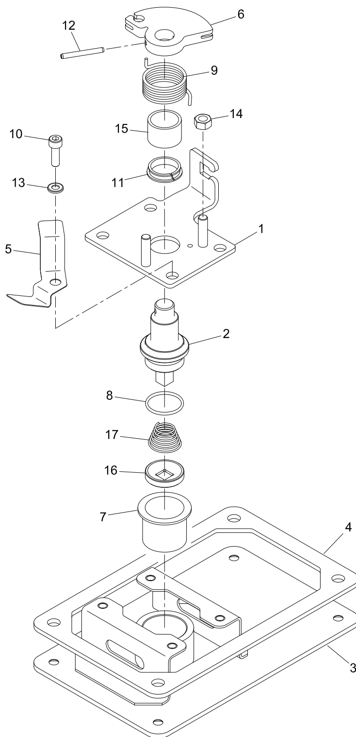
Figure 5.1 EMERGENCY ACCESS DEVICE ASSEMBLY (200940828)
