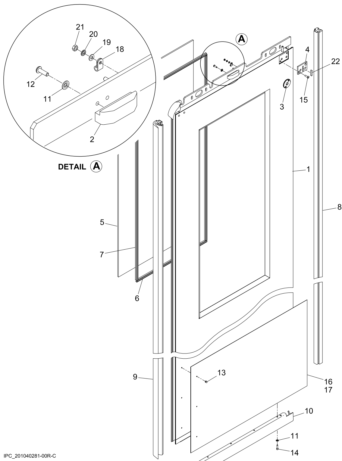
Figure 8.1 DOOR LEAF ASSEMBLY, LH (201040281)
