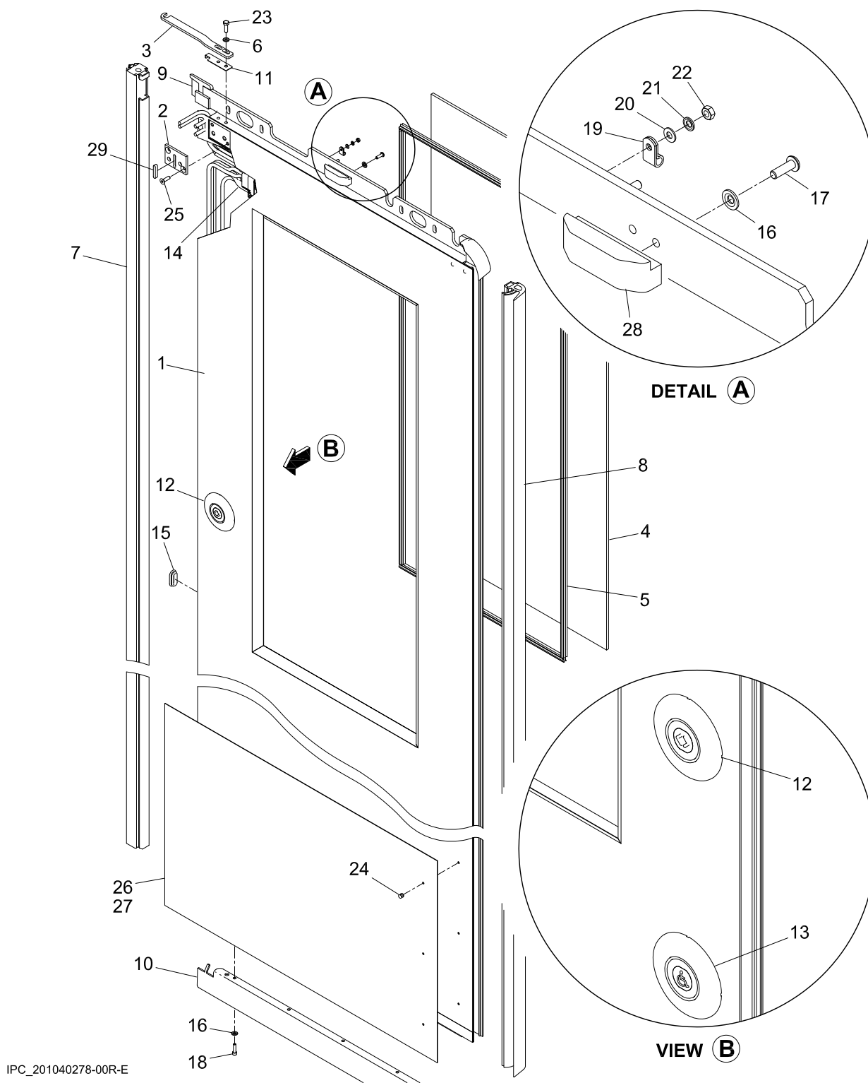
Figure 10.1 DOOR LEAF ASSEMBLY, CAB SIDE, RH (201040278)
