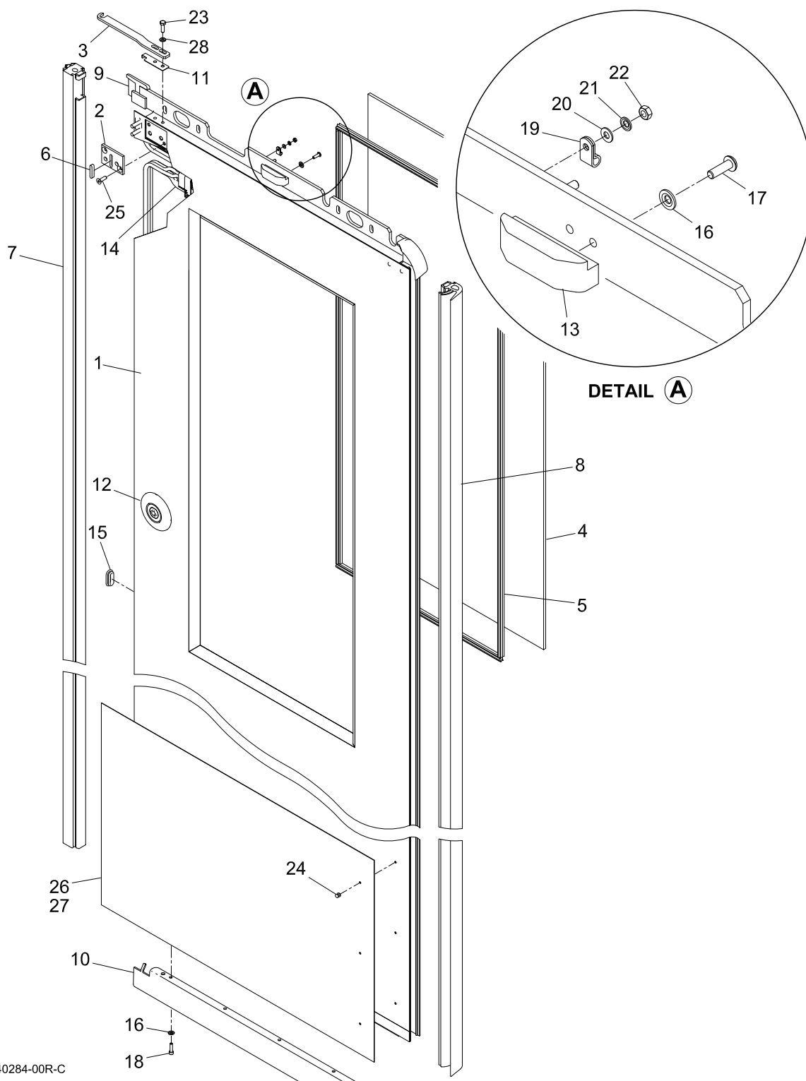
Figure 9.1 DOOR LEAF ASSEMBLY, RH (201040284)
