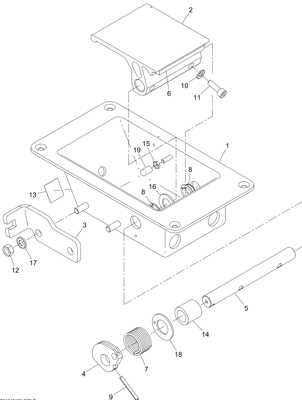
Figure 4.1 EMERGENCY EGRESS DEVICE ASSEMBLY (201040159)
