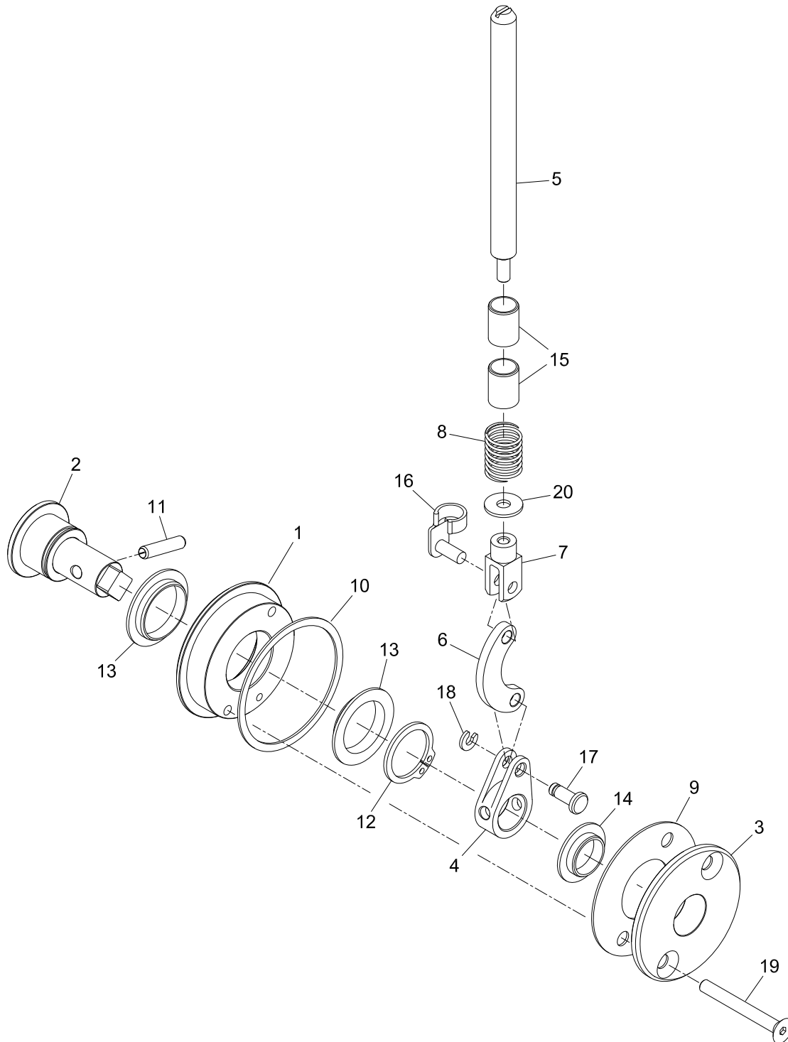
Figure 8.1.1 CUTOUT ASSEMBLY (201020386)
