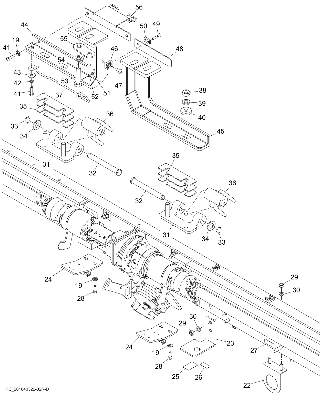
Figure 2.1 DOOR OPERATOR ASSEMBLY, RH (201040322) (Sheet 2 of 3)
