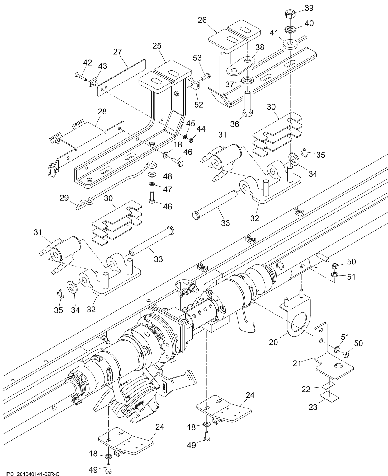
Figure 1.1 DOOR OPERATOR ASSEMBLY, LH (201040141) (Sheet 2 of 3)
