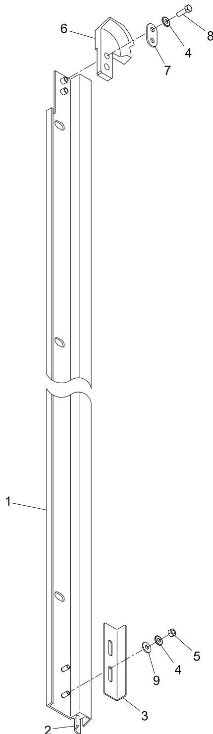
Figure 15 PORTAL SEAL ASSEMBLY, LEFT (20104022002)
