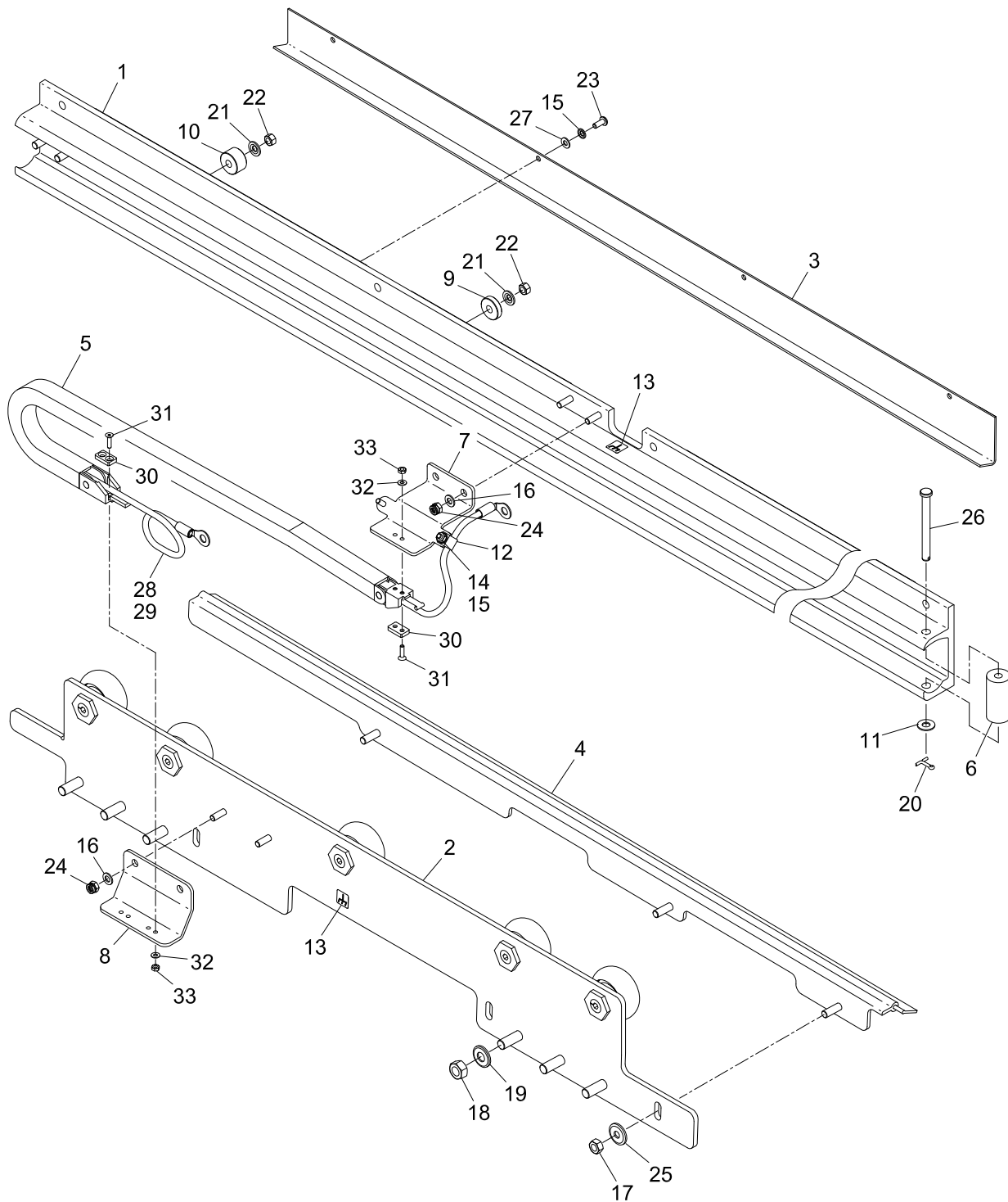
Figure 7.2 DOOR HANGER ASSEMBLY, LH (201040132)
