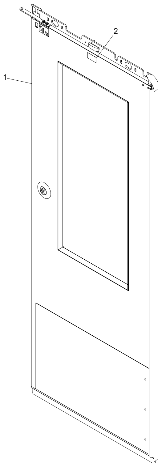
Figure 9 DOOR LEAF, RH (201040210)
