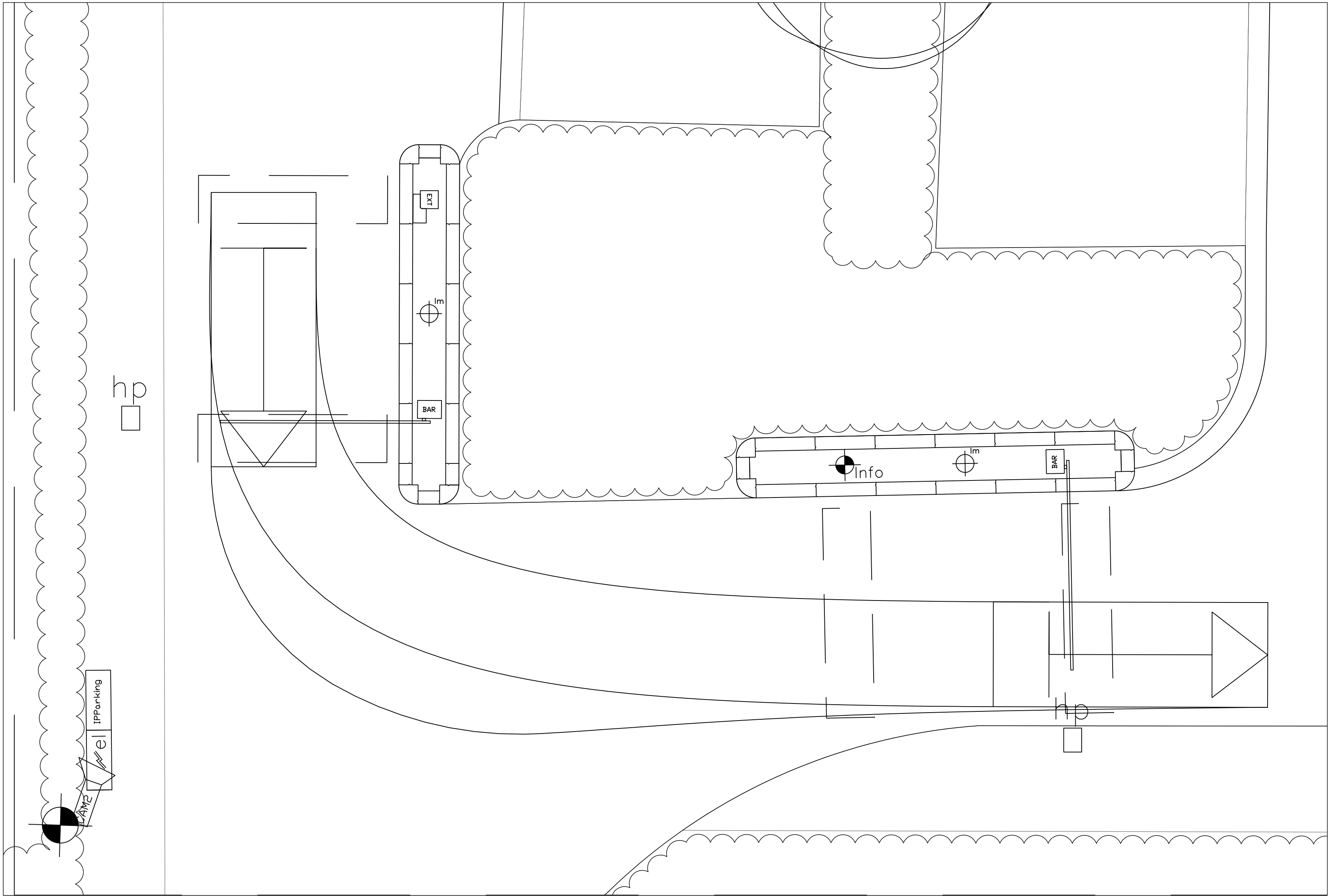
Detail 1, Entree, school 1:50
