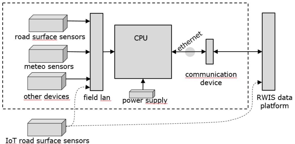
Figure 1: RWIS architecture
