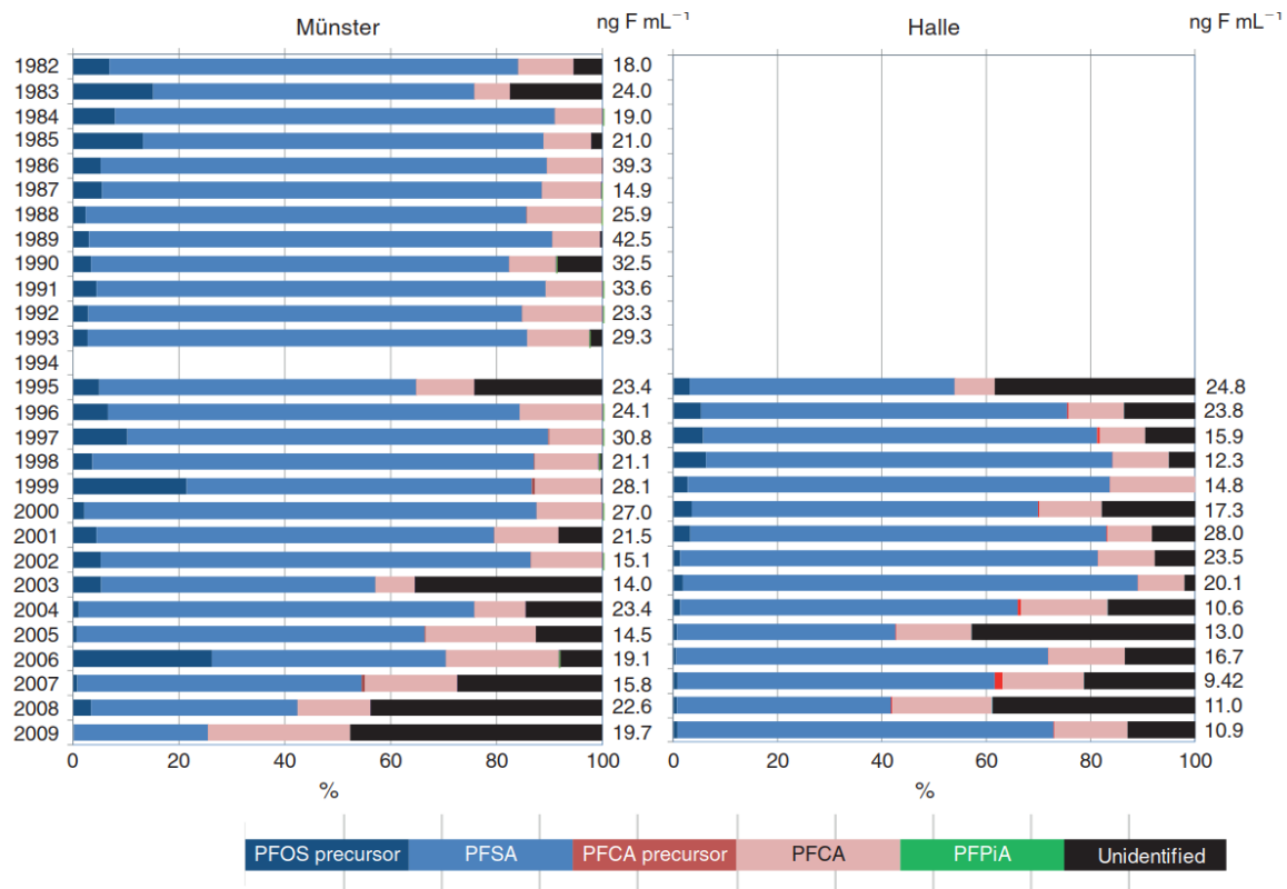
Figure 2 Composition and concentrations (ng F/ml) of EOF in German blood plasma samples (Yeung and Mabury, 2016)
