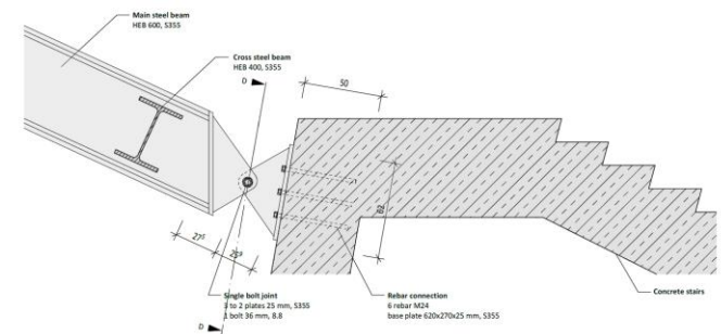
Section C-C S 1:20
