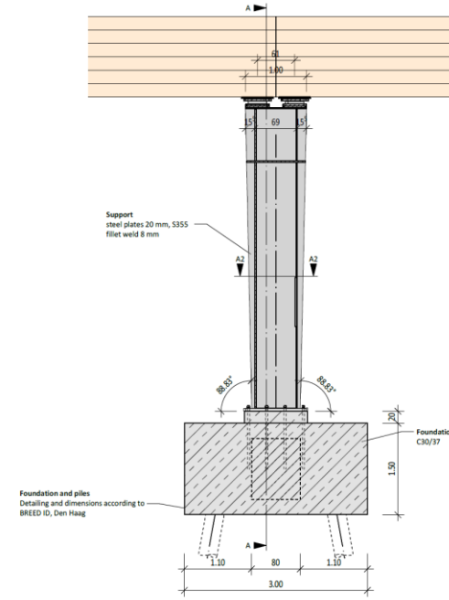
Section B-B S 1:50
