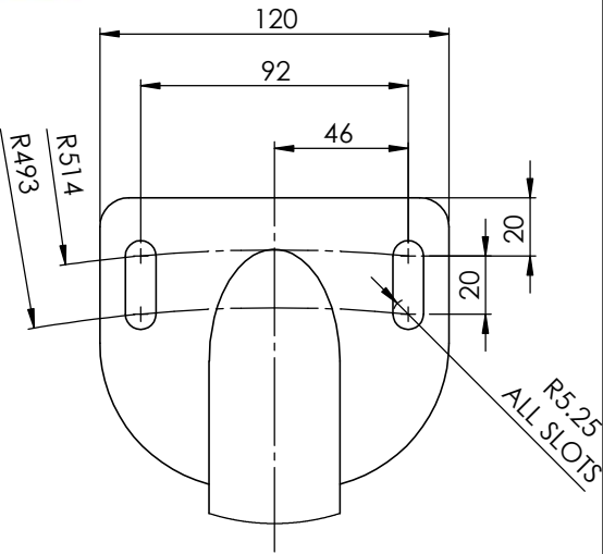
DETAIL A SCALE 1 : 2 FOOT MATERIAL: 5MM THICK 316 ST/ST
