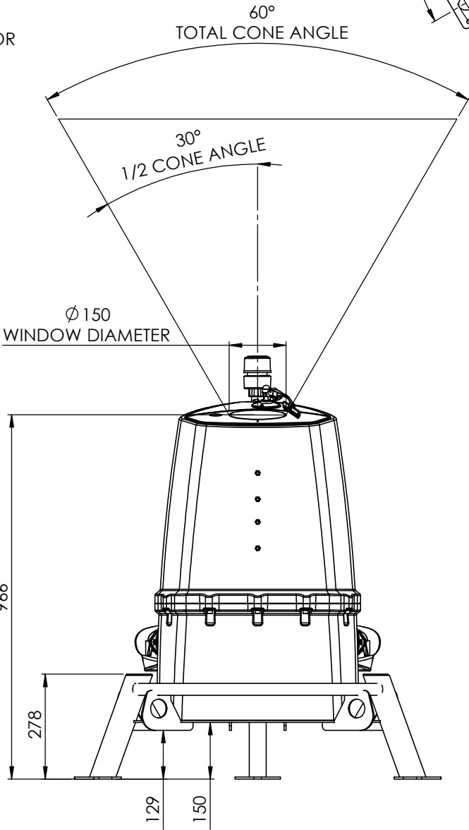
FRONT VIEW
