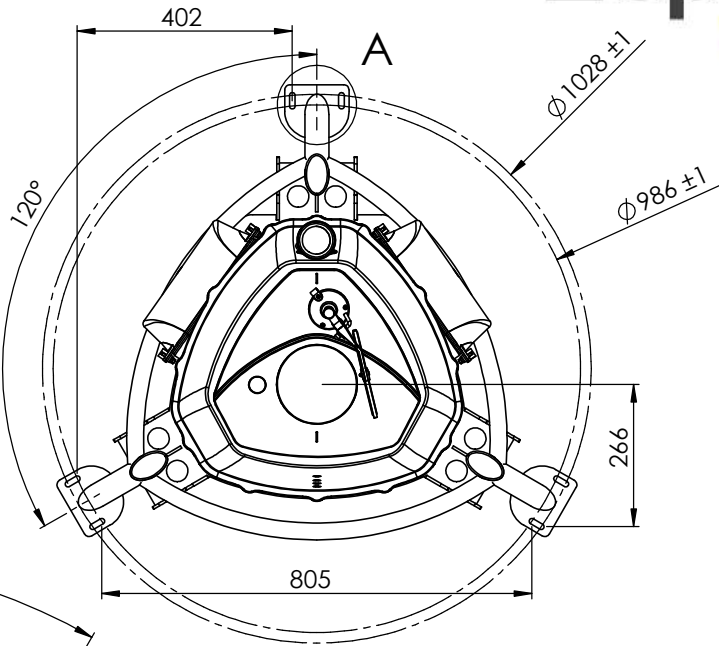
PLAN VIEW: LEG SPACING
