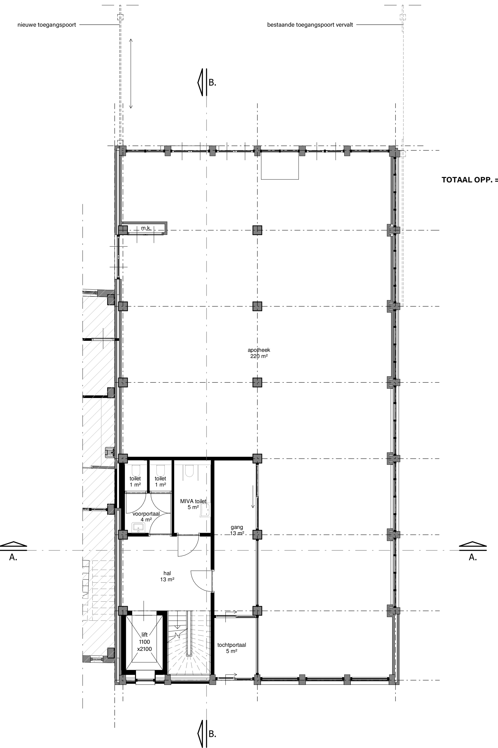
Begane grond (Peil =0)
