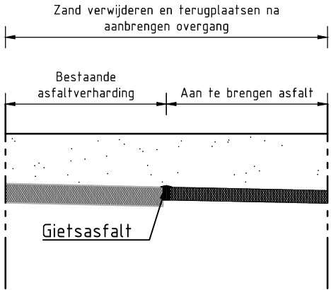
Detail 01: Overgang asfaltverharding schaal: 1:50
