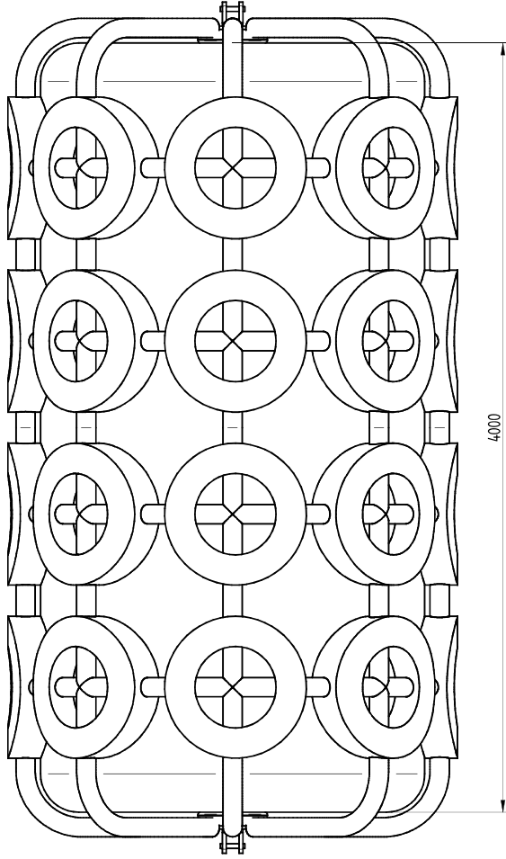
FRONT VIEW 1:25
