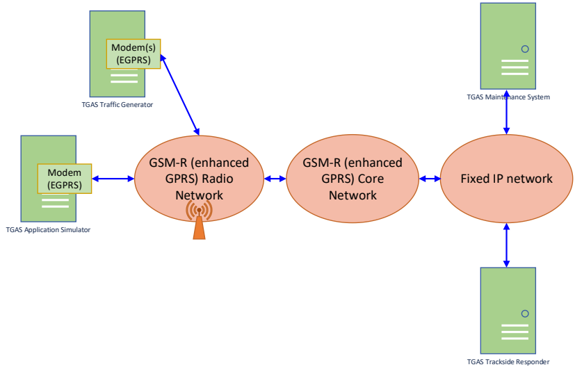
Figure 2 TGAS System overview
