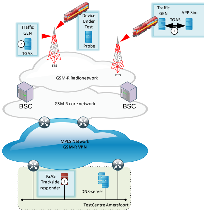
Figure 7 TGAS System architecture
